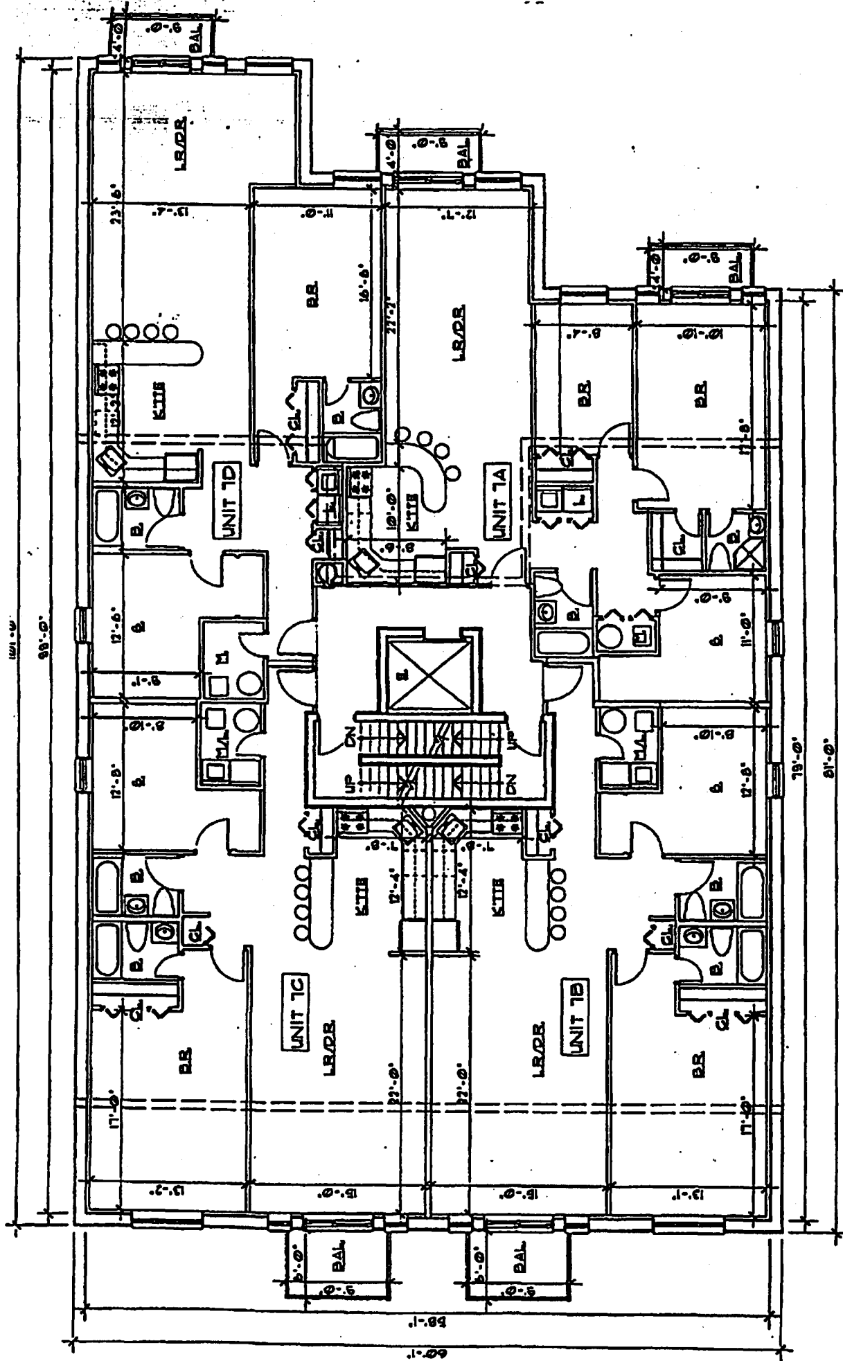
SEVENTH FLOOR PLAN
