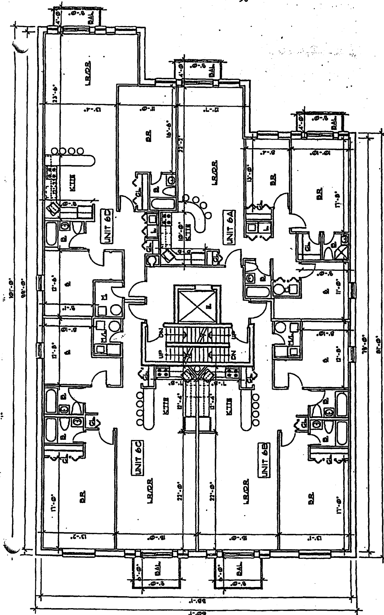
SIXTH FLOOR PLAN
