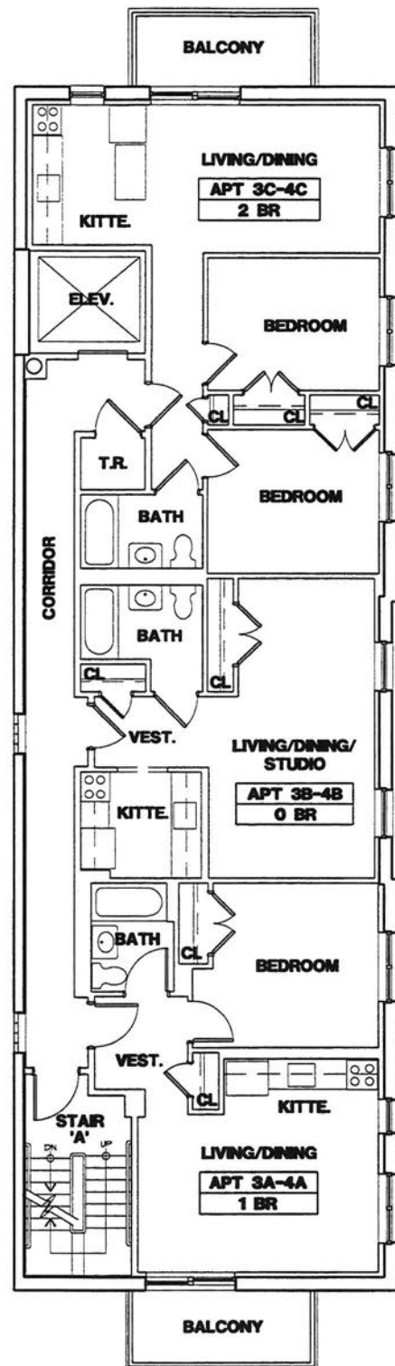
TYPICAL (3RD & 4TH) FLOOR
