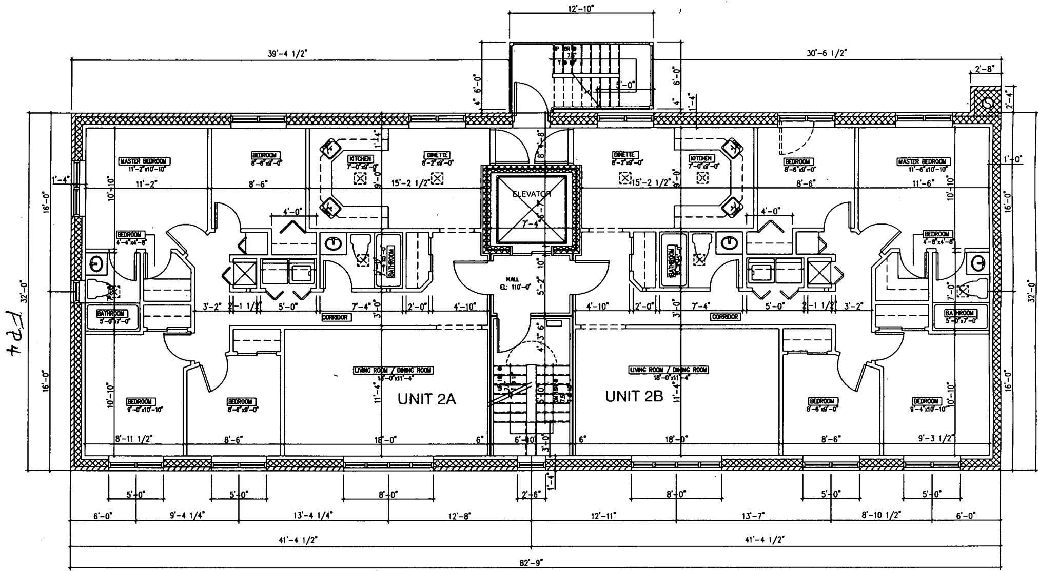
1 2nd FLOOR PLAN A-103 1/4"=1'-0"
