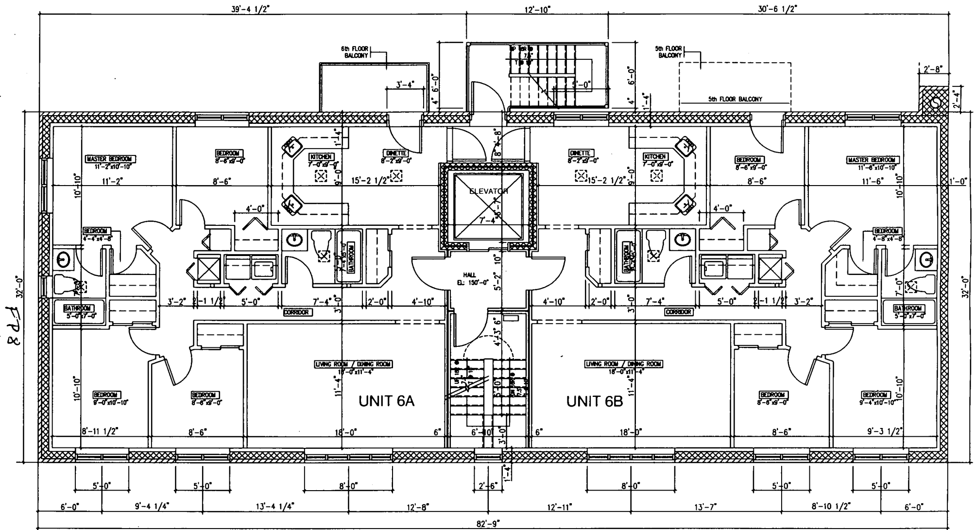
1 6th FLOOR PLAN A-107 1/4"=1'-0"
