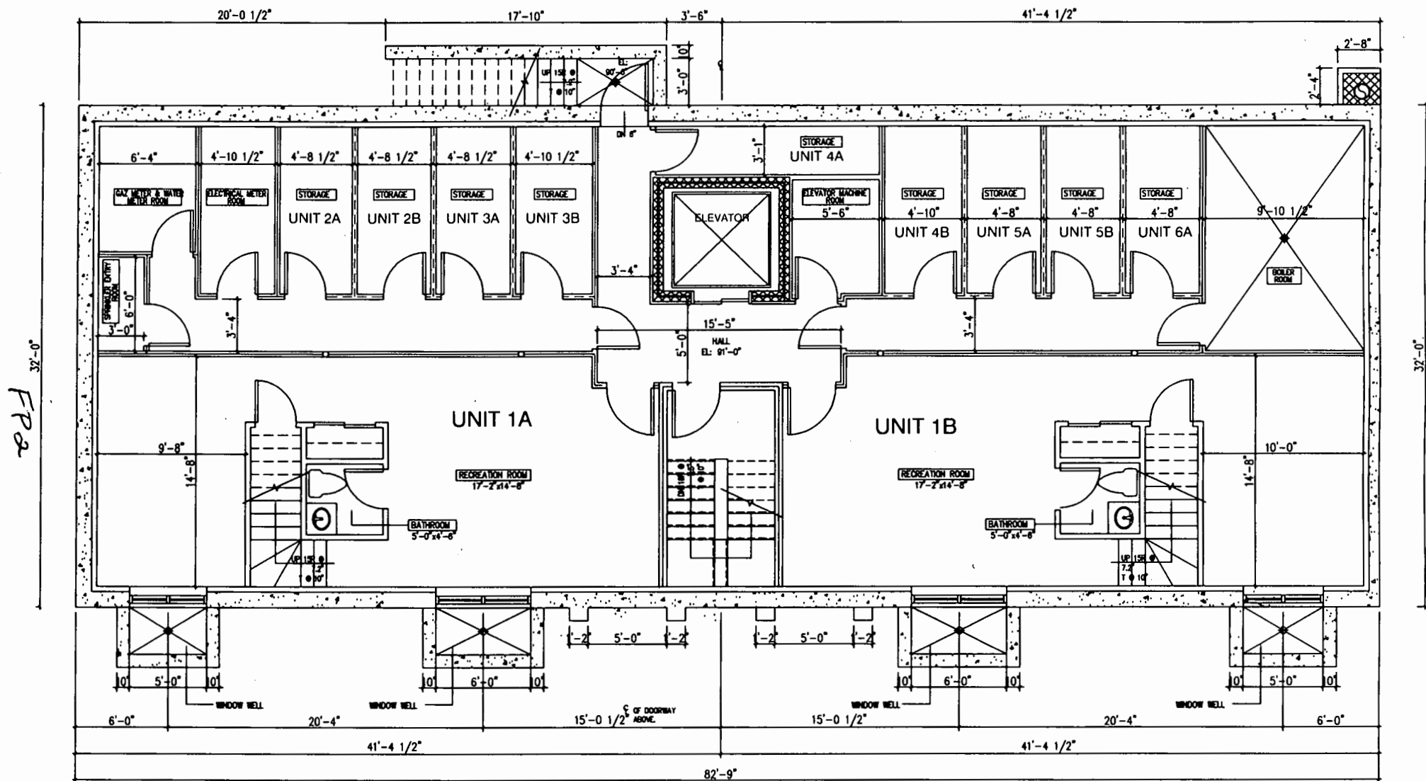
1 CELLAR FLOOR PLAN A-101 1/4"=1'-0"
