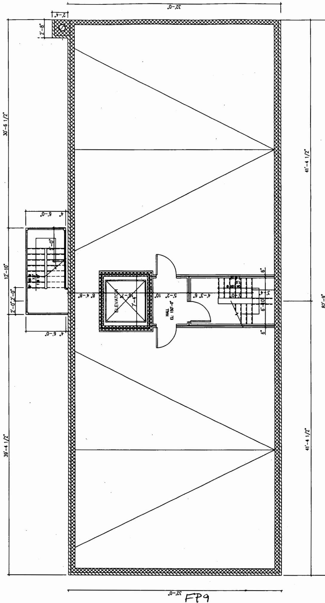
1 ROOF PLAN (COMMON) A-107 1/4"=1'-0"
