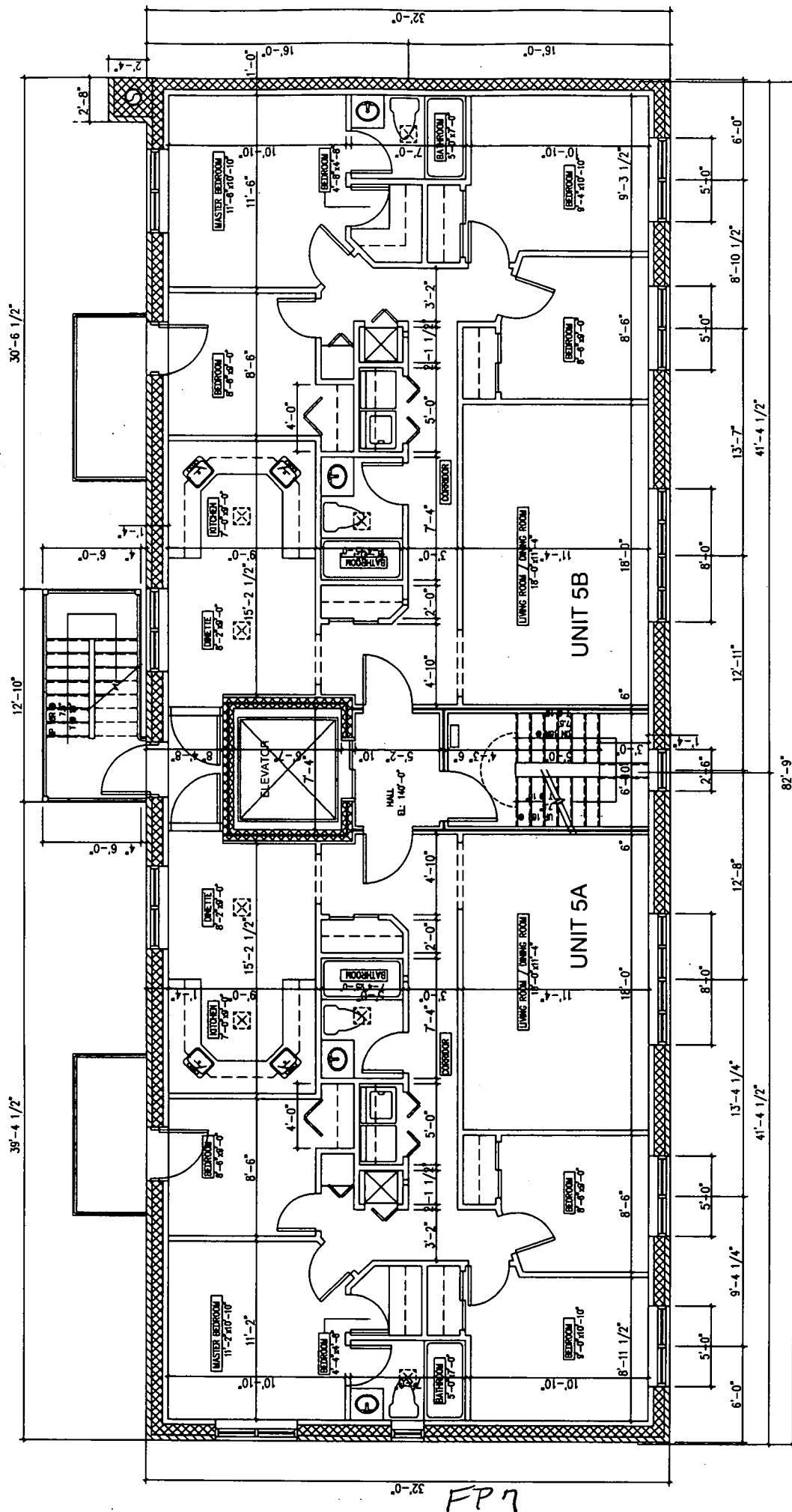
1 5th FLOOR PLAN A-105 1/4"=1'-0"
