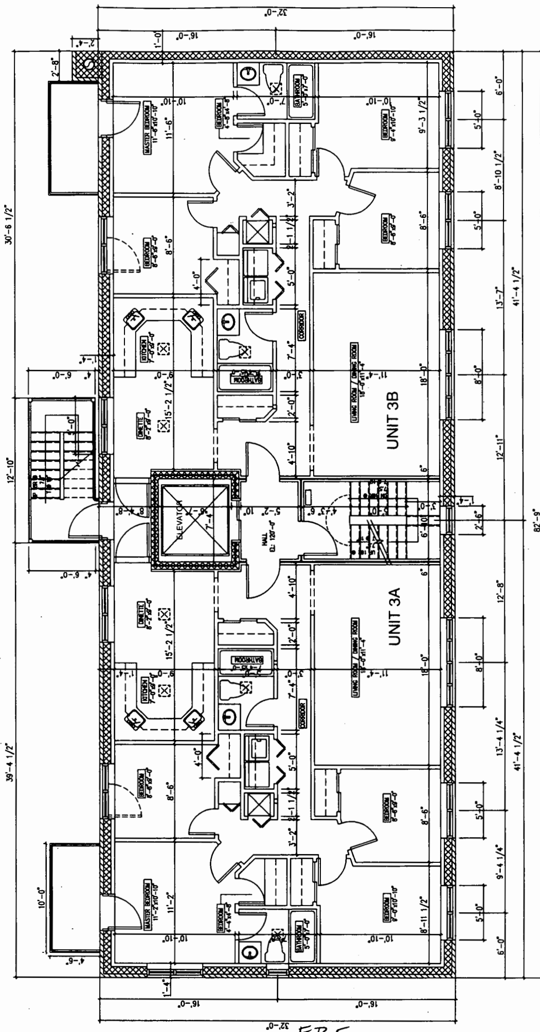
1 3rd FLOOR PLAN A-104 1/4"=1'-0"
