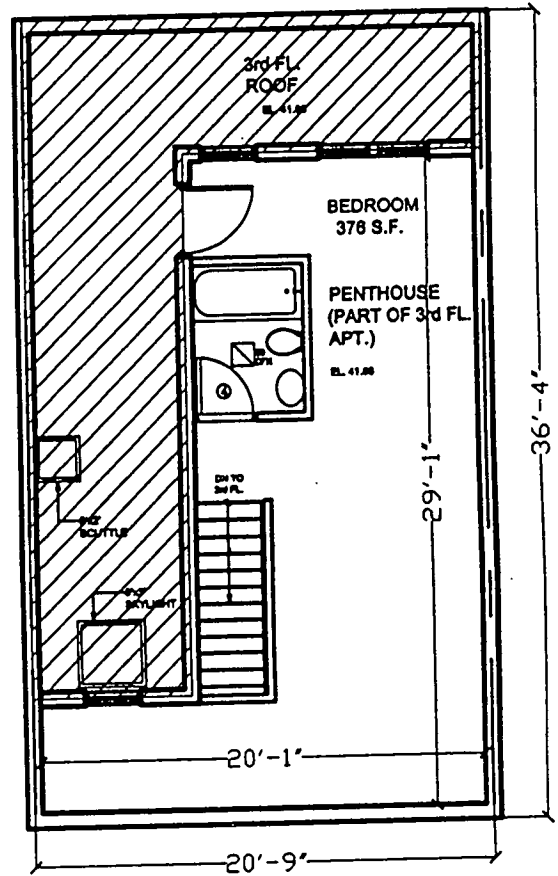
PENTHOUSE PART OF 3rd FL.
