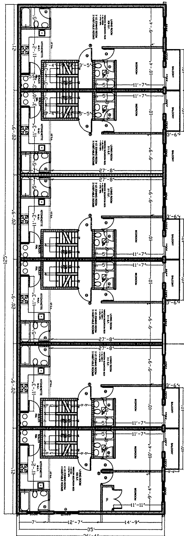
2nd FLOOR PLAN NTS
