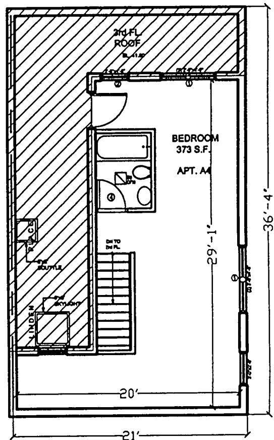
PENTHOUSE PART OF 3rd FL.
