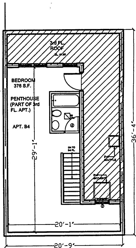
PENTHOUSE PART OF 3rd FL.
