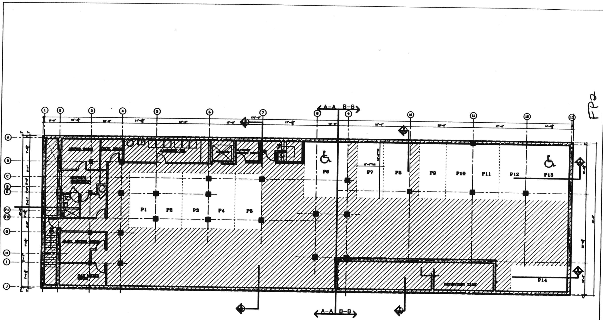
CELLAR PLAN
