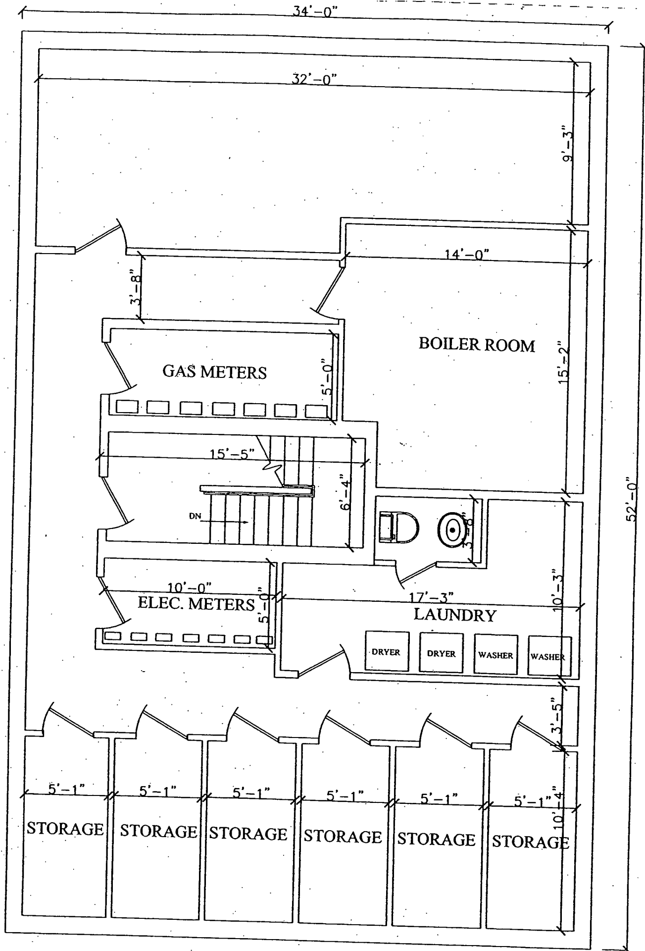
CELLAR FLOOR PLAN
