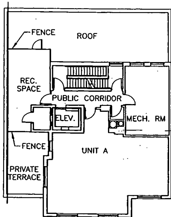
7TH FLOOR KEY PLAN
