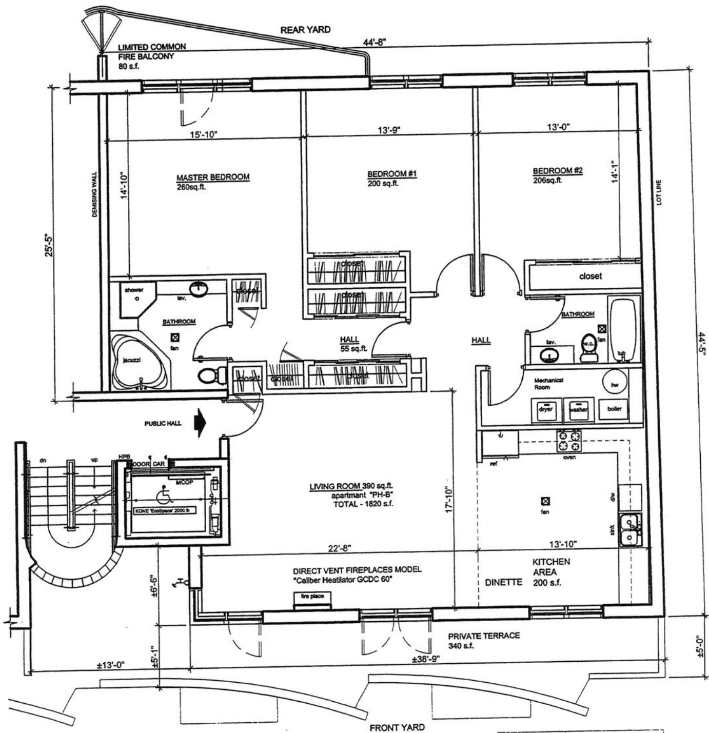
A-13 RESIDENCE APARTMENT "PH-B" THIRD FLOOR (ALL DIMENSIONS AND SQUARE FOOTAGES ARE APPROXIMATE) TOTAL APT. "PH-B" = 1820 S.F. 0 1 2 4 8 FEET SCALE: 1/8" = 1'-0"
