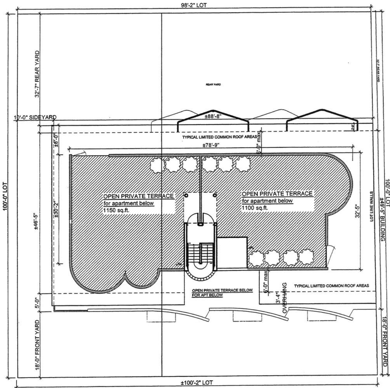
A-14 ROOF PRIVATE TERRACE (ALL DIMENSIONS AND SQUARE FOOTAGES ARE APPROXIMATE)
