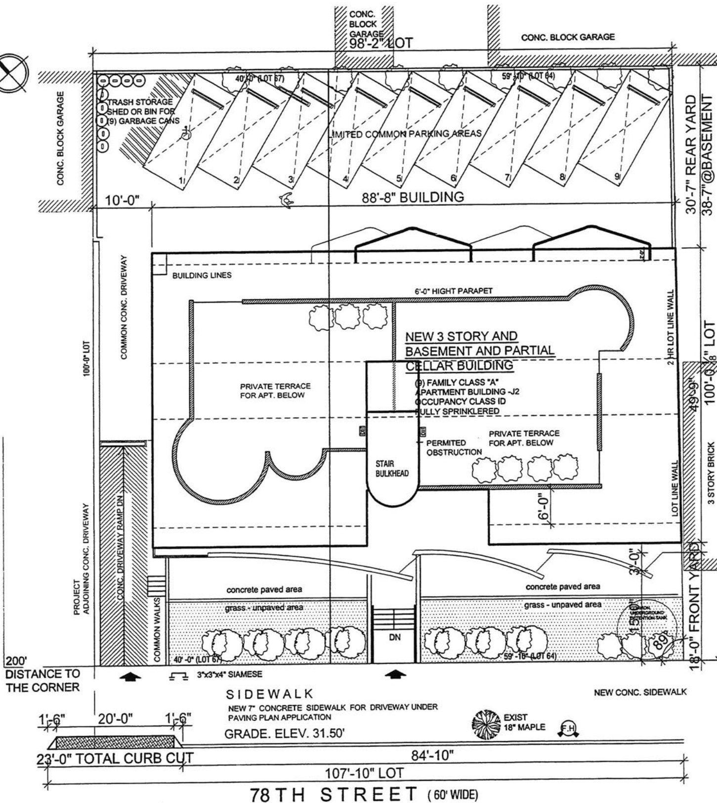
A-1 PLOT PLAN (ALL DIMENSIONS AND SQUARE FOOTAGES ARE APPROXIMATE)
