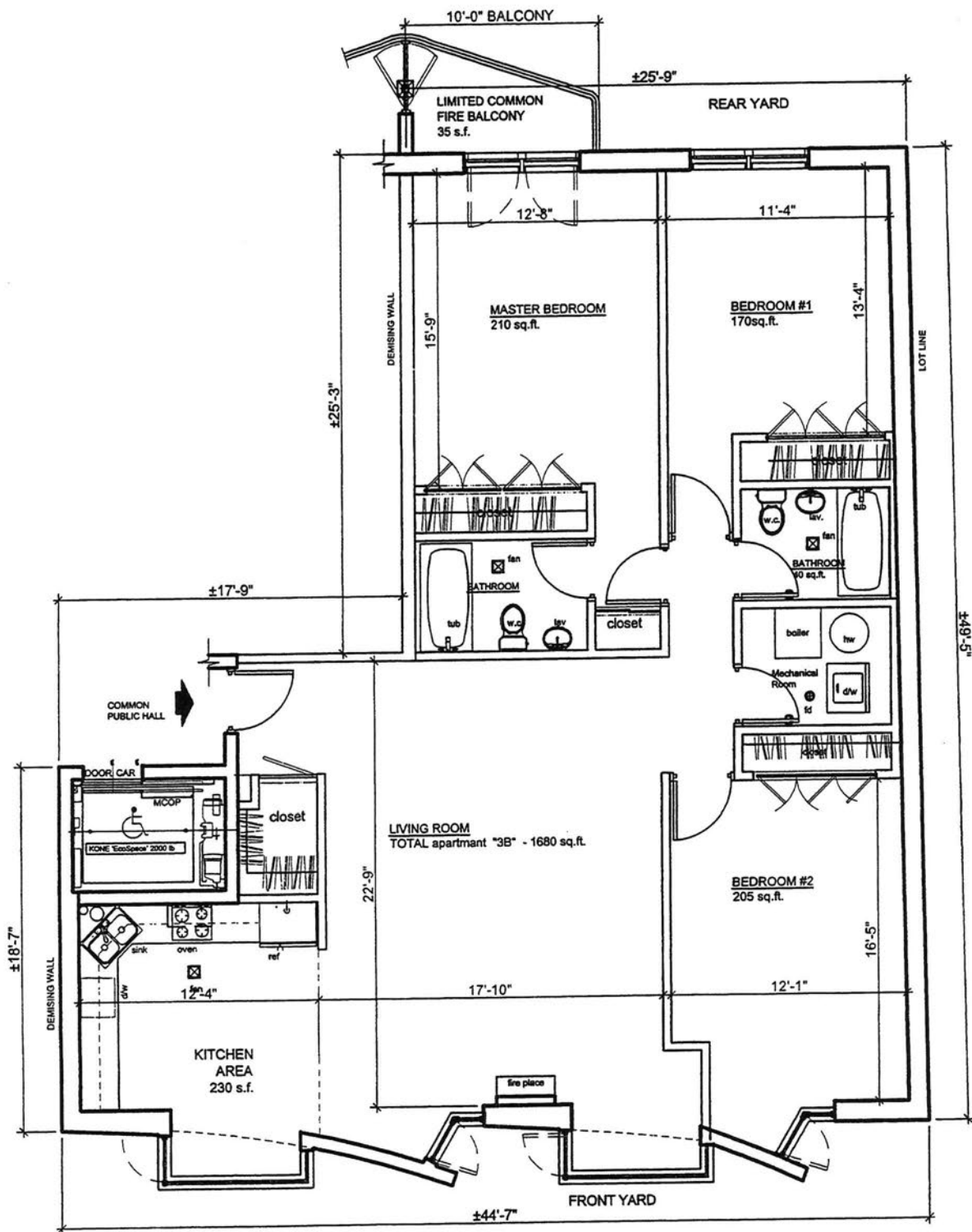
A-11 RESIDENCE APARTMENT "3B" SECOND FLOOR (ALL DIMENSIONS AND SQUARE FOOTAGES ARE APPROXIMATE) TOTAL APT. "3B" = 1680 S.F. 0 1 2 4 8 FEET SCALE: 1/8" = 1'-0"
