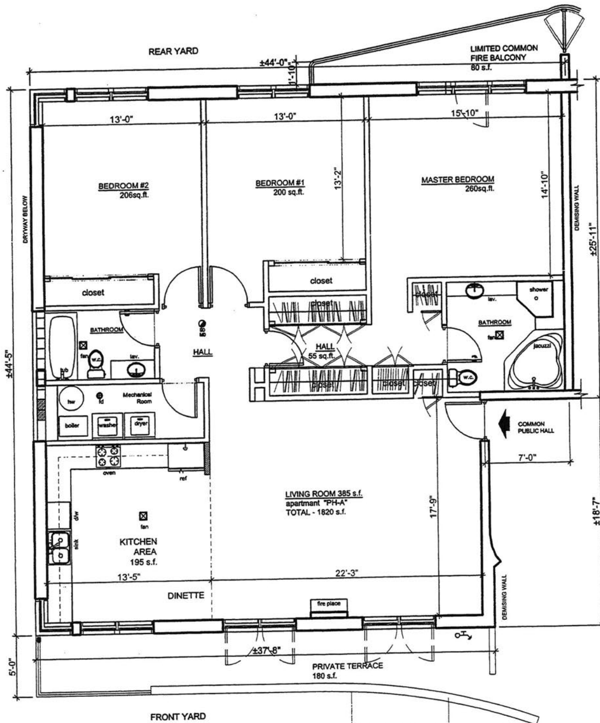
A-12 RESIDENCE APARTMENT "PH-A" THIRD FLOOR (ALL DIMENSIONS AND SQUARE FOOTAGES ARE APPROXIMATE)
