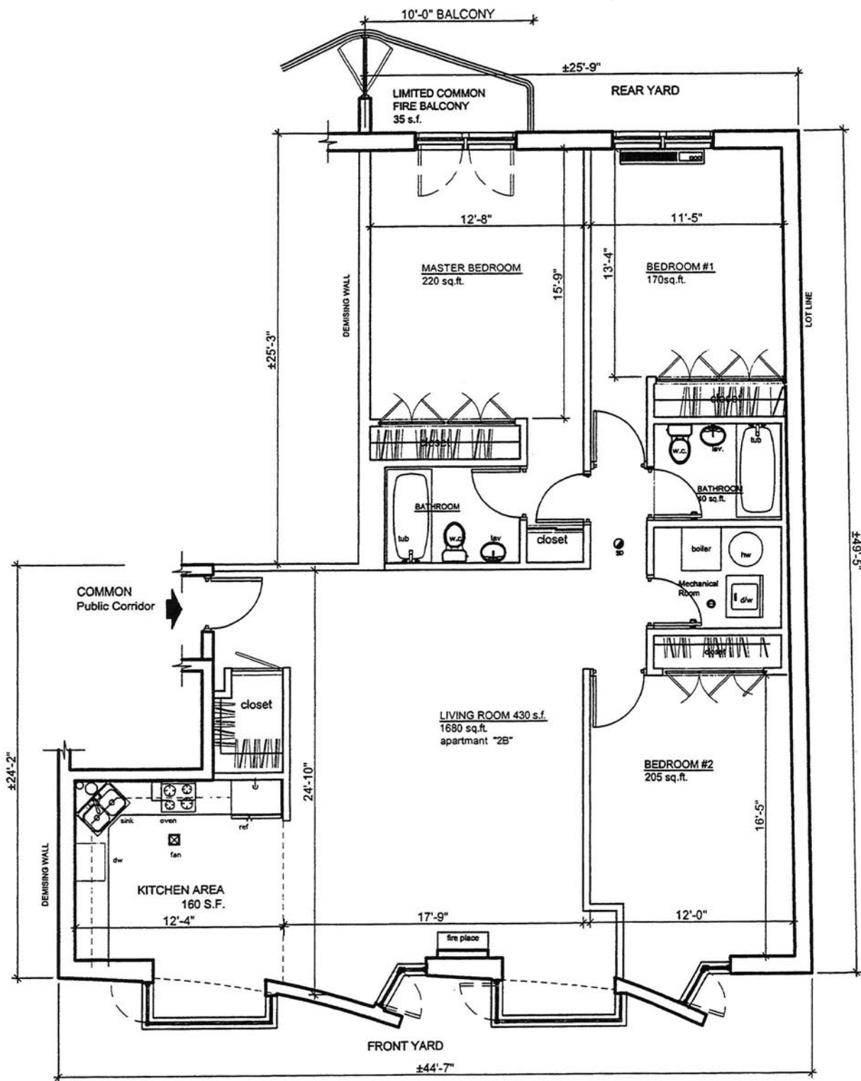
A-7 RESIDENCE APARTMENT "2B" FIRST FLOOR (ALL DIMENSIONS AND SQUARE FOOTAGES ARE APPROXIMATE) TOTAL APT. "2B" = 1680 S.F. 0 1 2 4 8 FEET SCALE: 1/8" = 1'-0"
