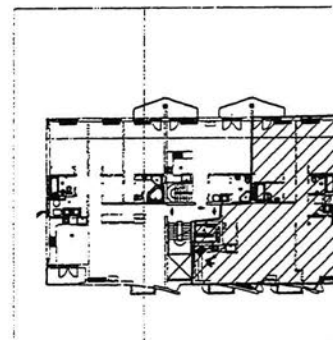
A-7 RESIDENCE APARTMENT "2B" FIRST FLOOR (ALL DIMENSIONS AND SQUARE FOOTAGES ARE APPROXIMATE) TOTAL APT. "2B" = 1680 S.F. 0 1 2 4 8 FEET SCALE: 1/8" = 1'-0"
