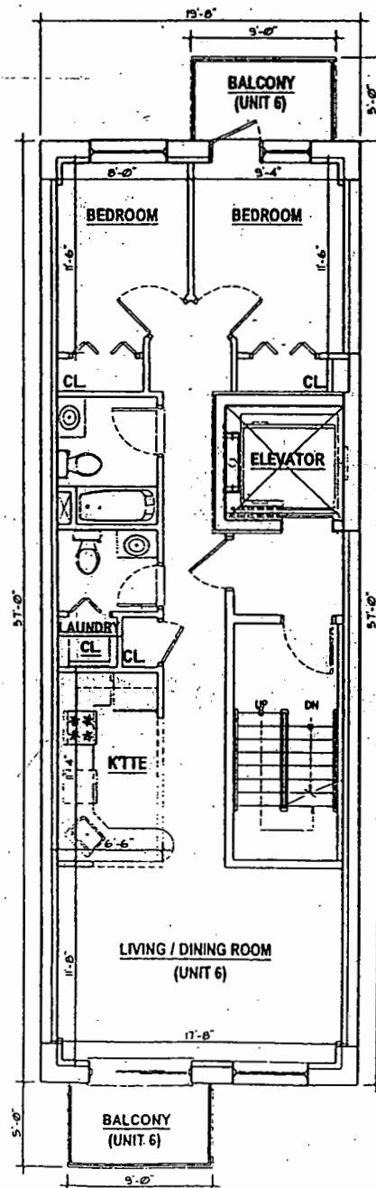
SIXTH FLOOR PLAN
