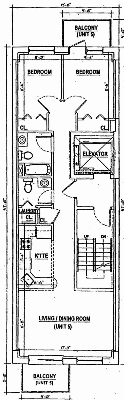
FIFTH FLOOR PLAN
