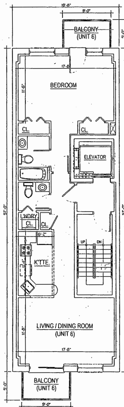
SIXTH FLOOR PLAN
