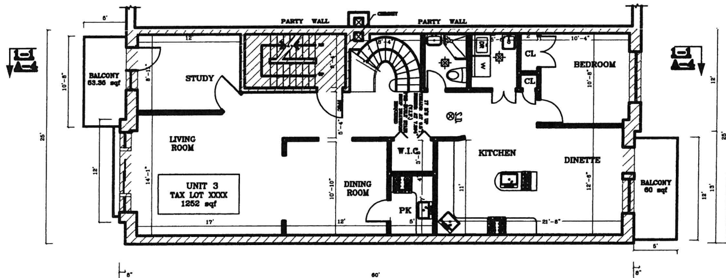
THIRD FLOOR PLAN SCALE: 1/4"=1'-0"
