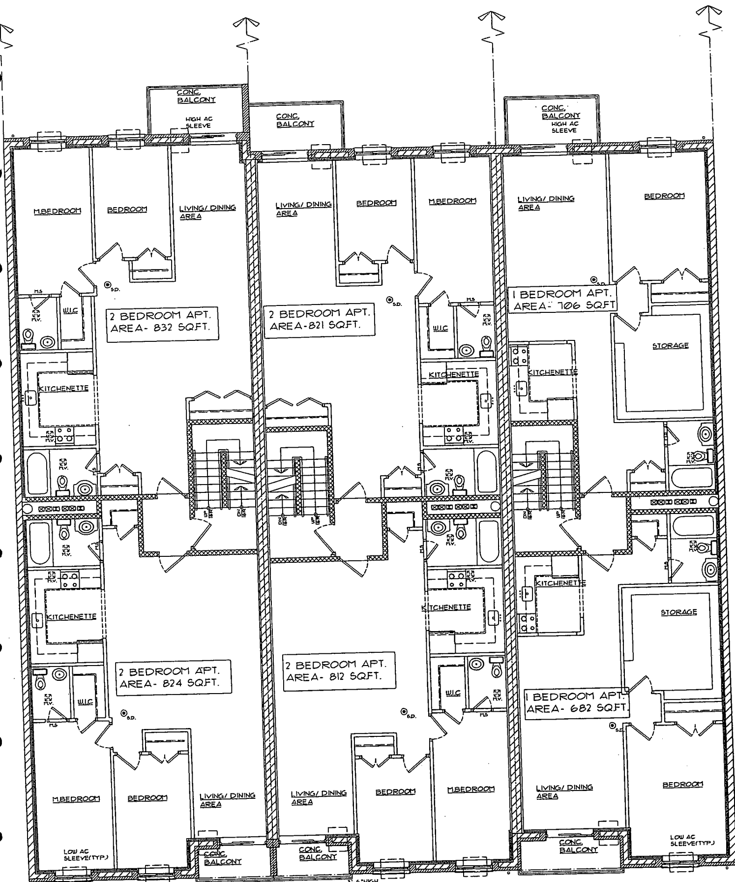
2ND, 3RD AND 4TH FLOOR PLAN
