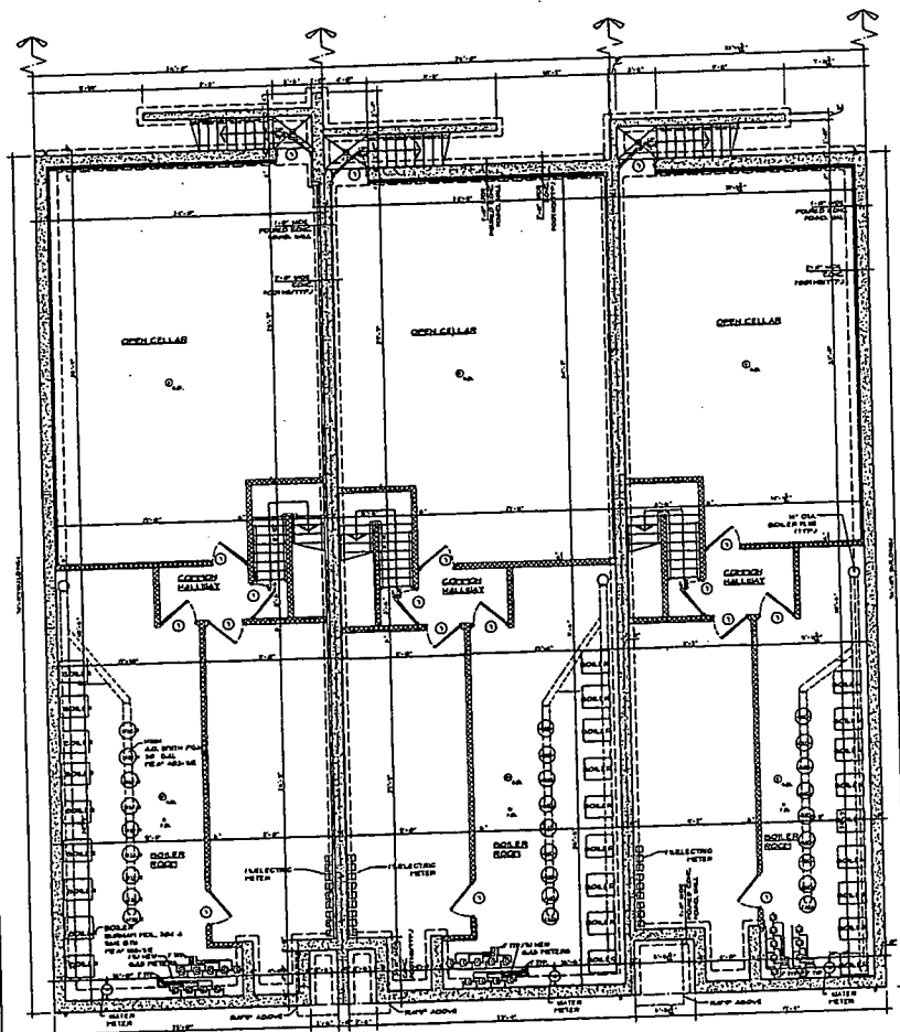
CELLAR FLOOR PLAN SCALE: 1/4" = 1'-0"
