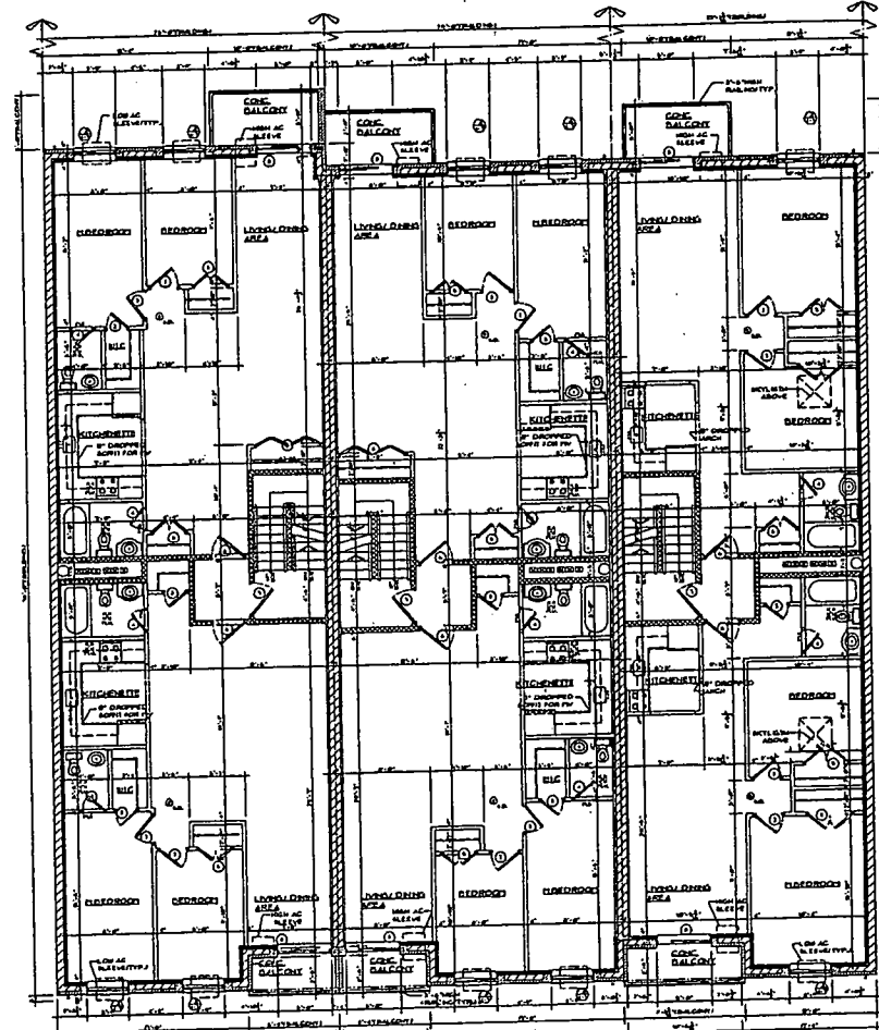
4TH FLOOR PLAN SCALE: 1/4" = 1'-0"
