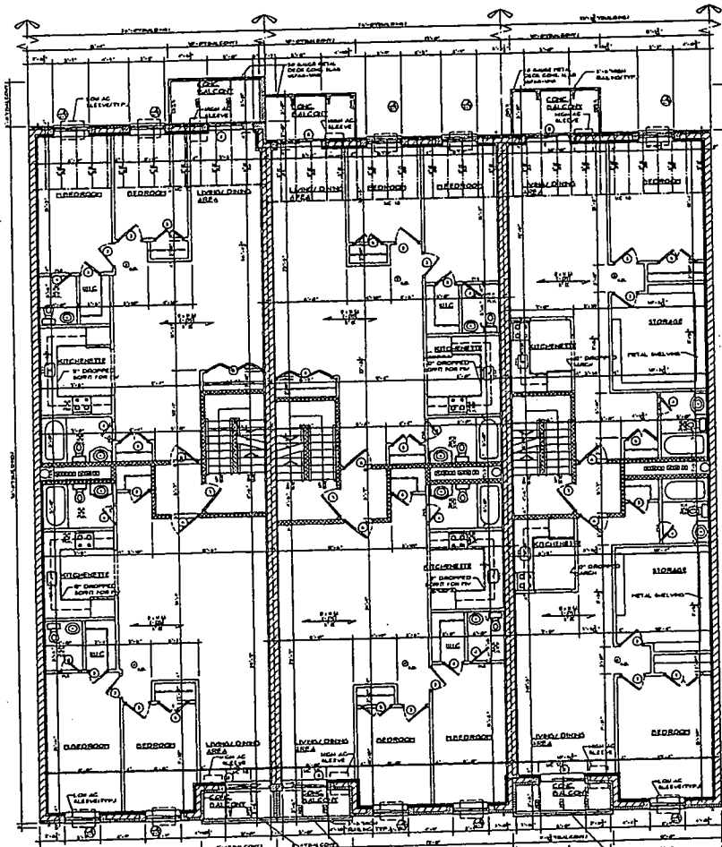
2ND AND 3RD FLOOR PLAN SCALE: 1/4" = 1'-0"
