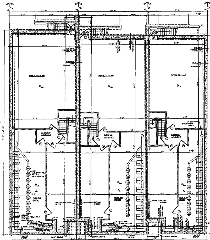
CELLAR FLOOR PLAN
