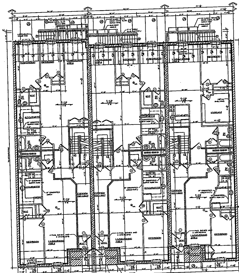
1ST FLOOR PLAN SCALE: 1/4" = 1'-0"
