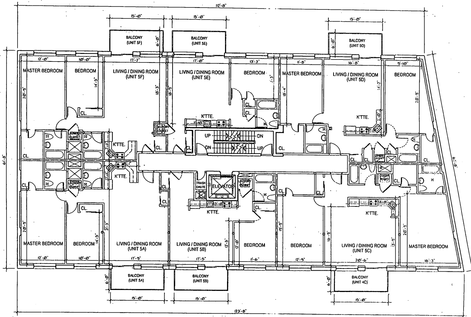
FIFTH FLOOR PLAN
