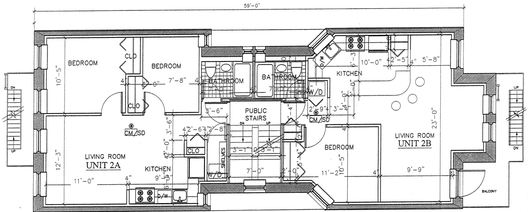
1 2ND FLOOR PLAN A1.03 Scale: 1/4" = 1'-0"
