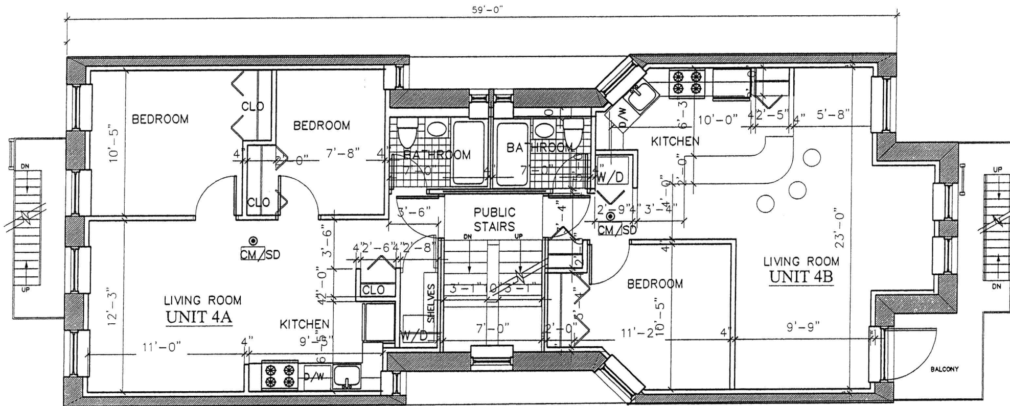
1 4TH FLOOR PLAN A1.03 Scale: 1/4" = 1'-0"
