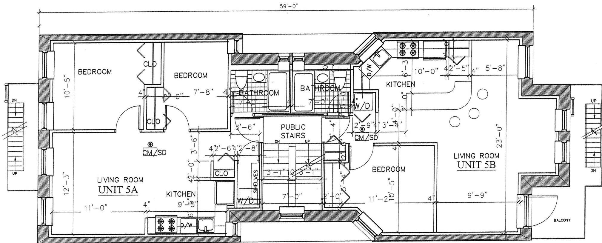
1 5TH FLOOR PLAN A1.03 Scale: 1/4" = 1'-0"
