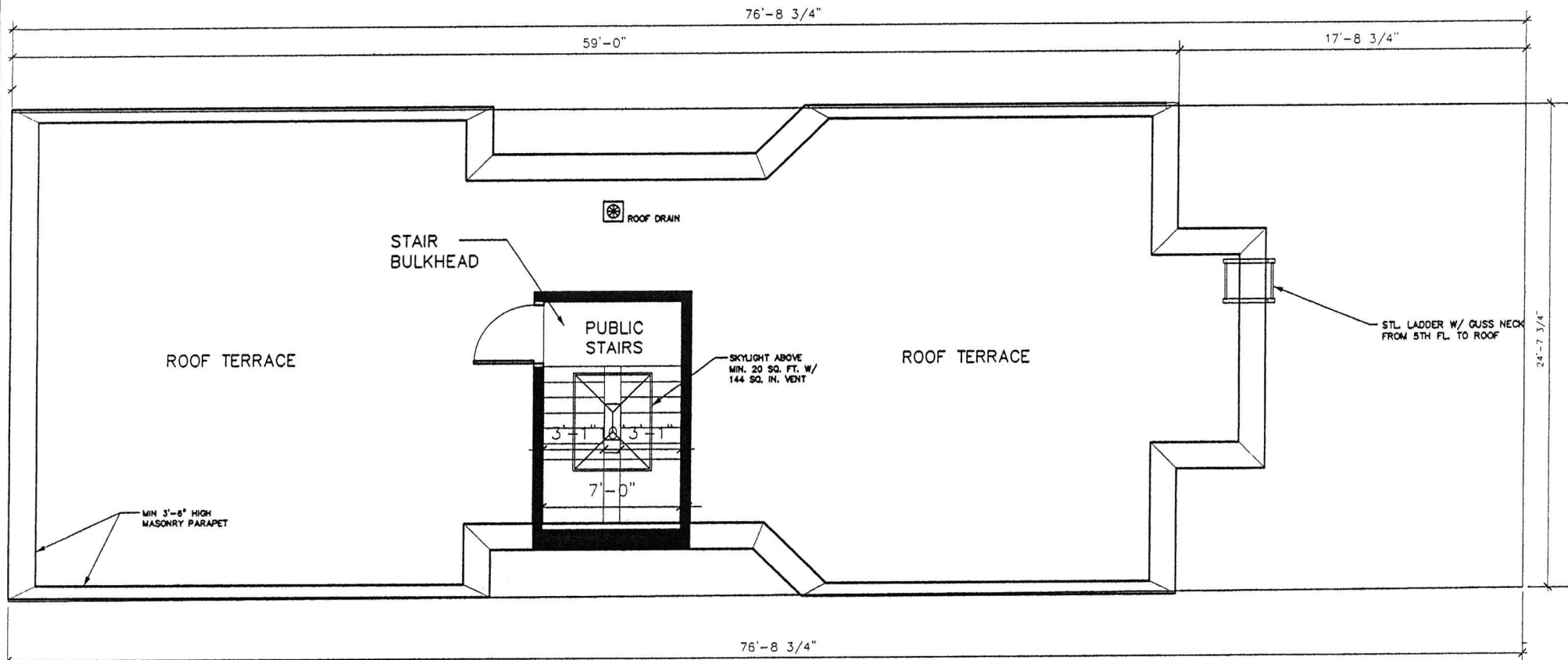
2 ROOF PLAN A1.03 Scale: 1/4" = 1'-0"
