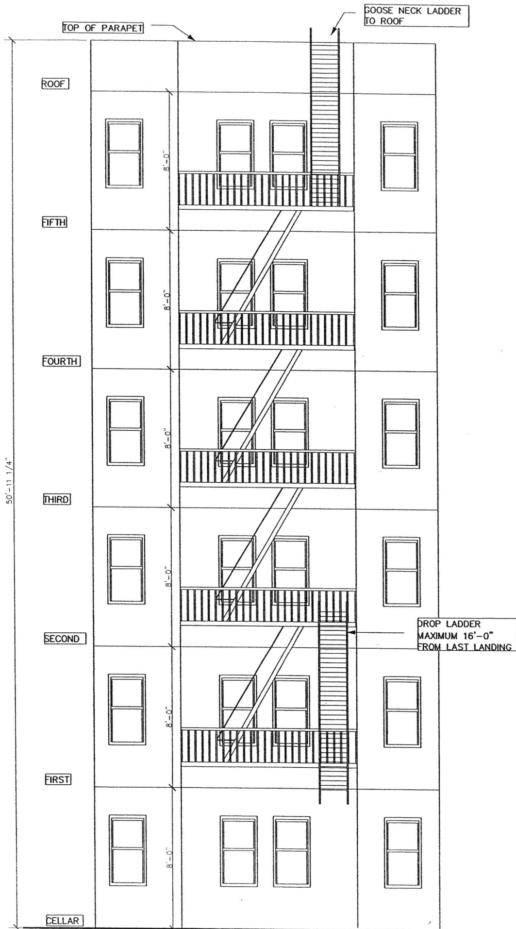
REAR ELEVATION
