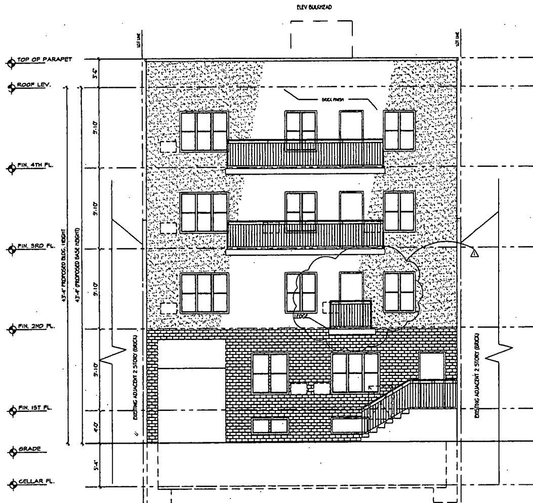
FRONT ELEVATION (@ 62nd STREET)
