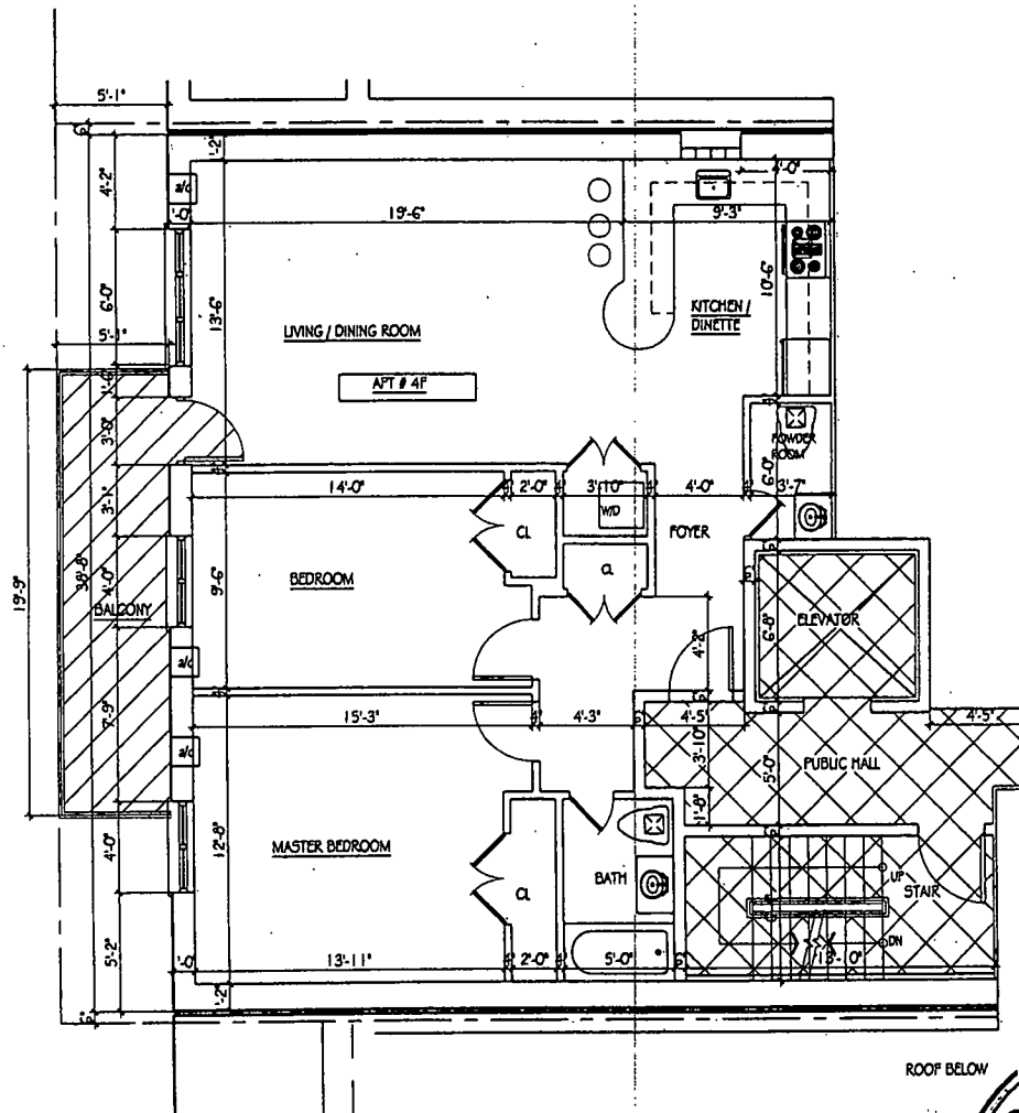
4TH FLOOR FRONT
