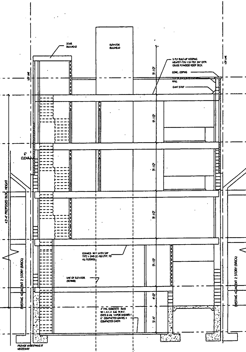
CROSS SECTION
