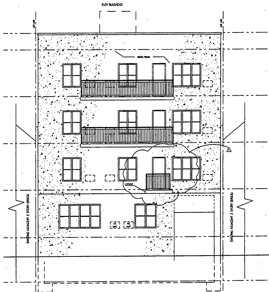
REAR ELEVATION
