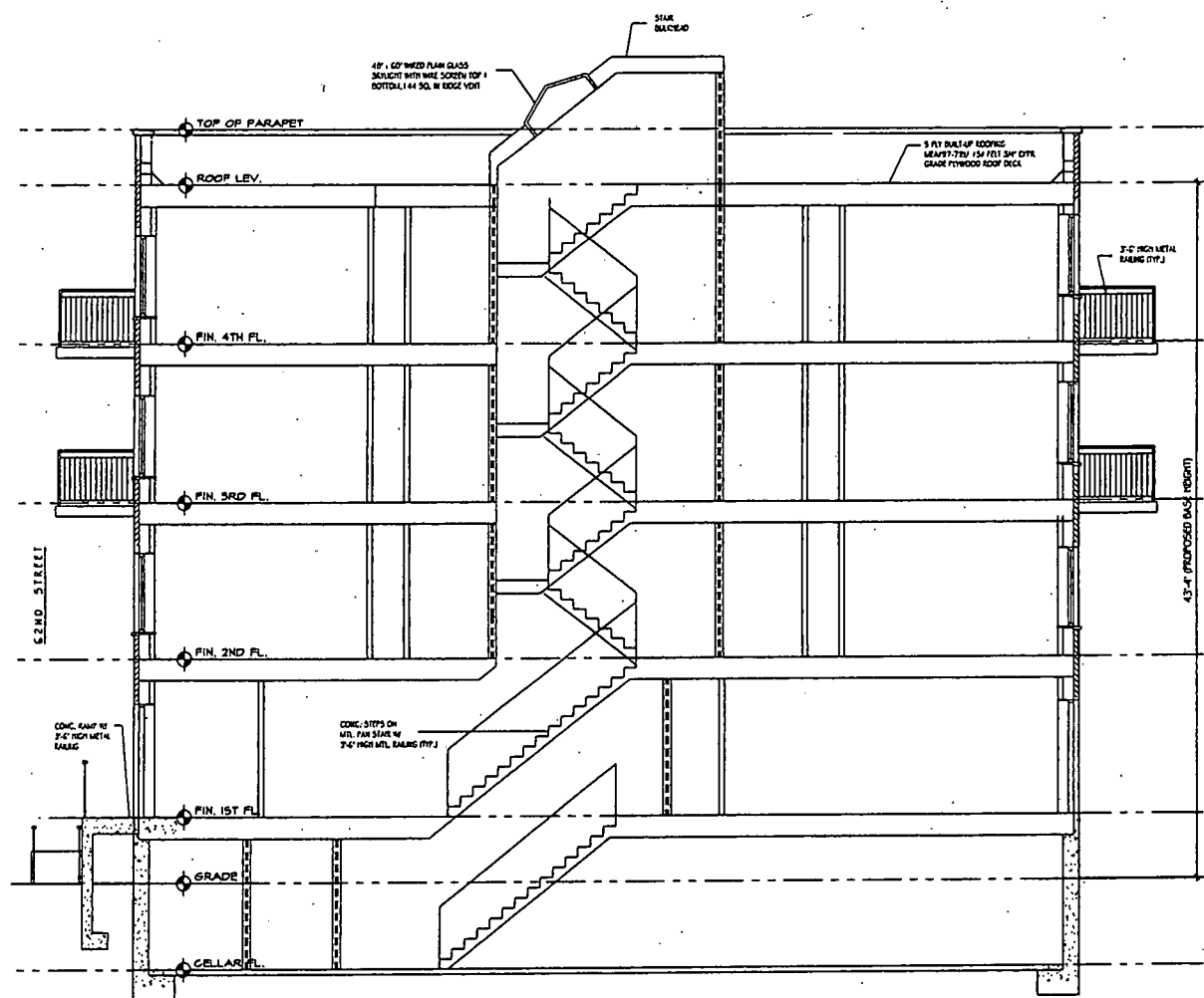
FRONT ELEVATION (@ 62nd STREET)
