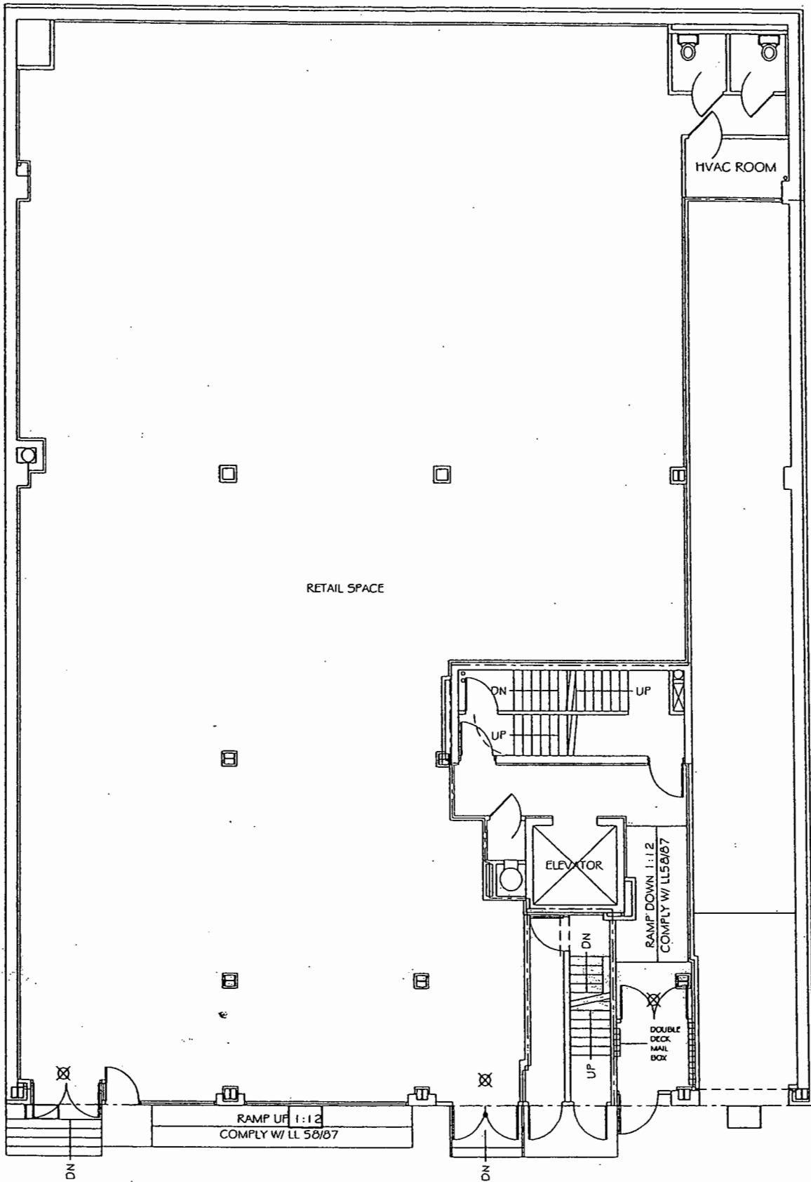
BASEMENT FLOOR KEY PLAN
