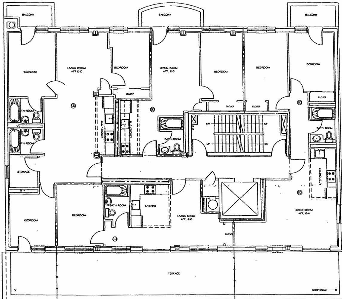
SIXTH FLOOR KEY PLAN
