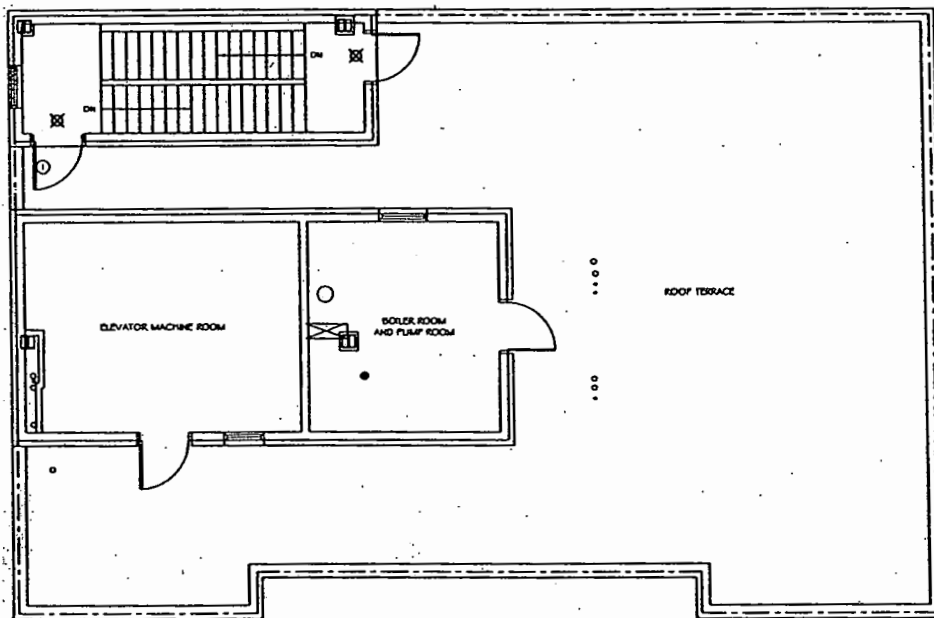
MECHANICAL PENTHOUSE FLOOR PLAN (MAIN ROOF PLAN)
