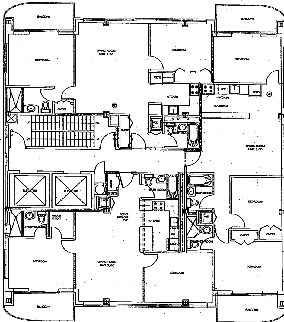
TYPICAL FLOOR PLAN (3RD TO 8TH FLOOR)
