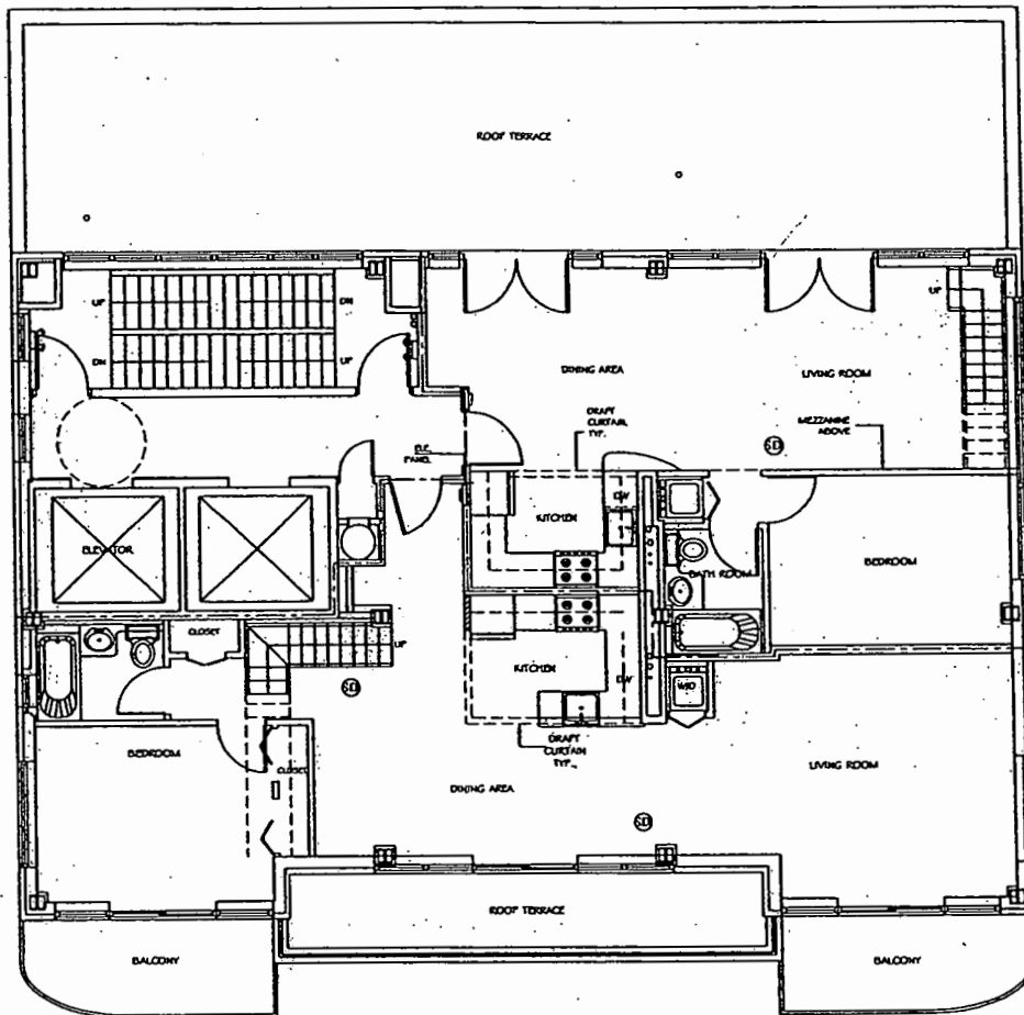
TENTH FLOOR PLAN
