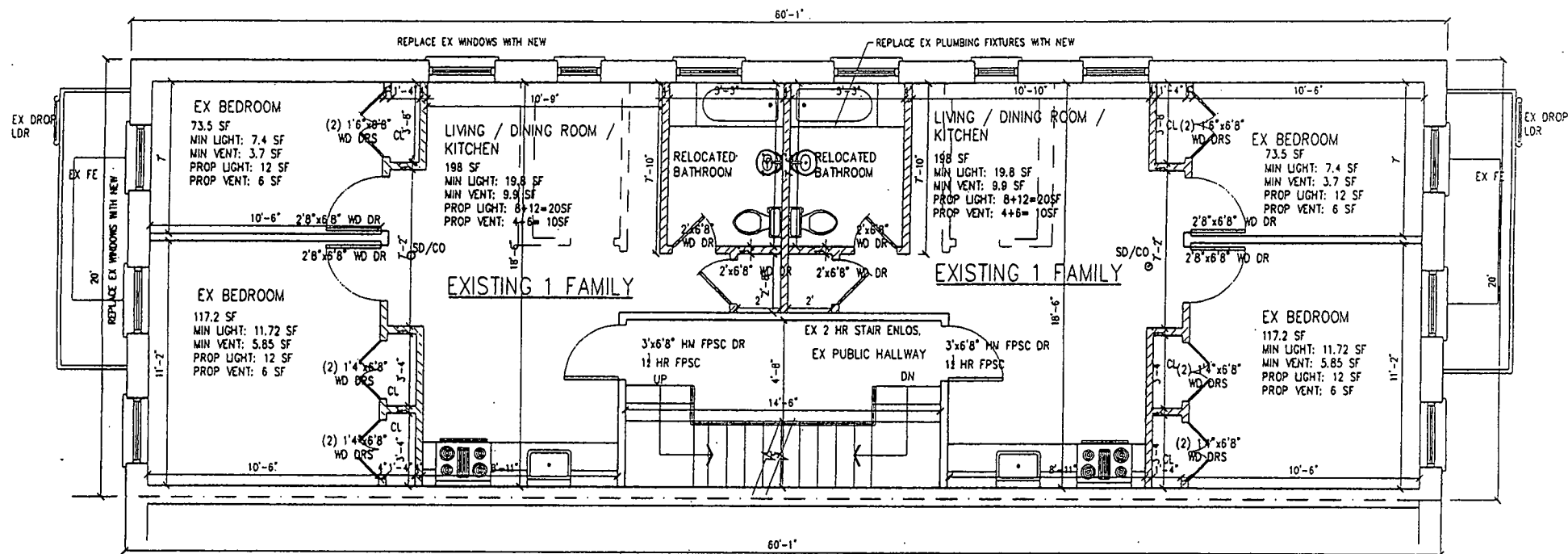
PROPOSED 2nd FLOOR PLAN
