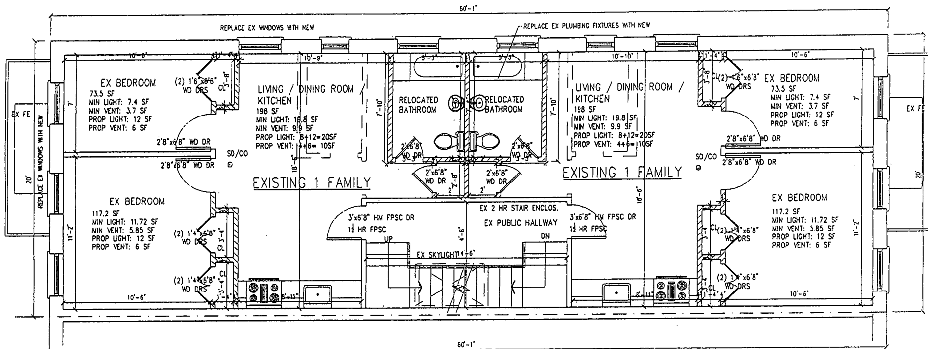
PROPOSED 3rd FLOOR PLAN SCALE: 1/8" = 1'-0" CLG HT = 9'-0"
