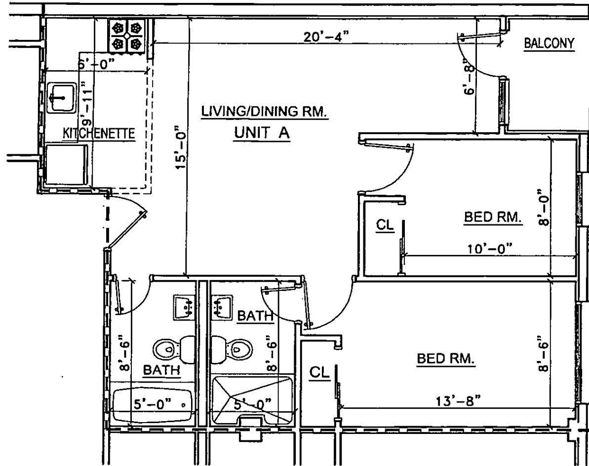
FOURTH FLOOR UNIT 4A 747.27 S.F.
