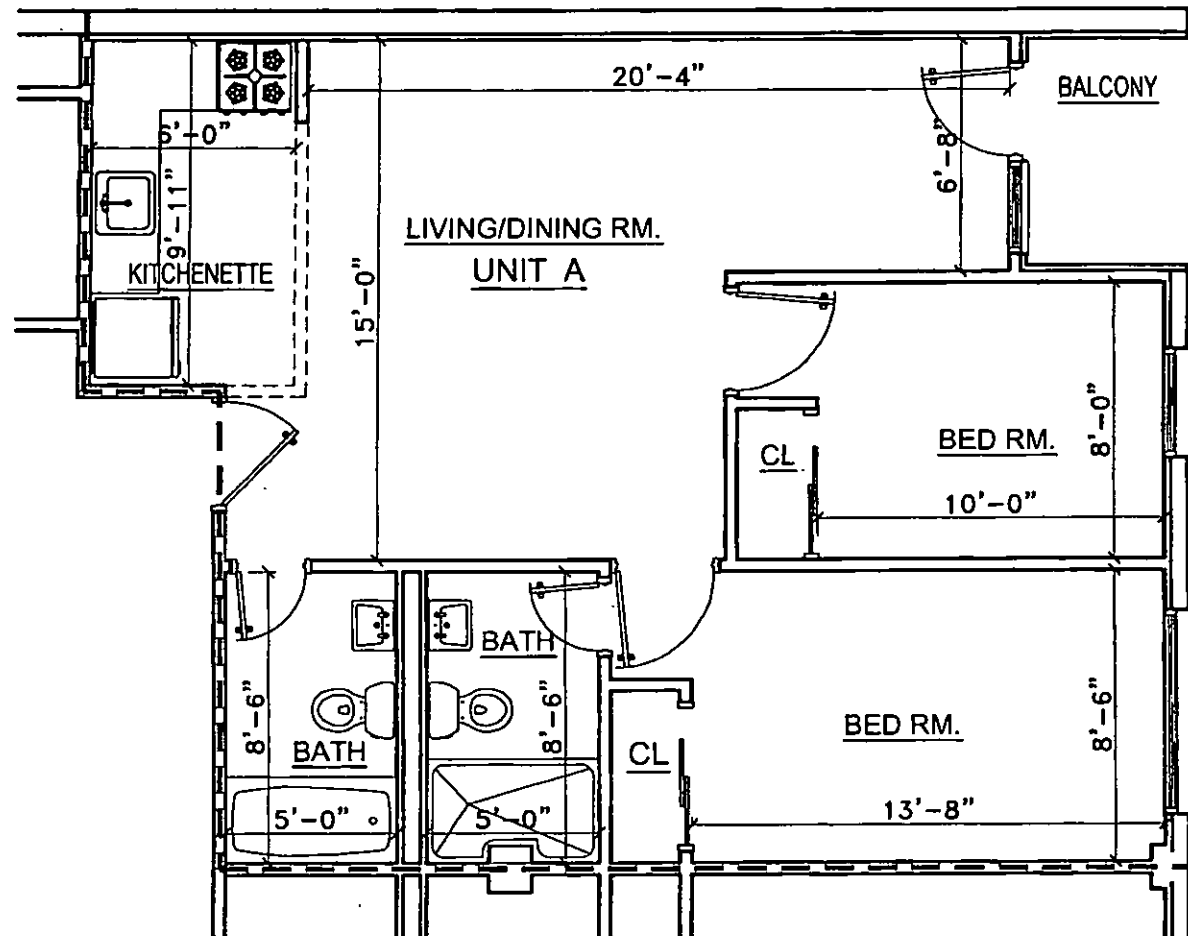
THIRD FLOOR UNIT 3A 747.27 S.F.
