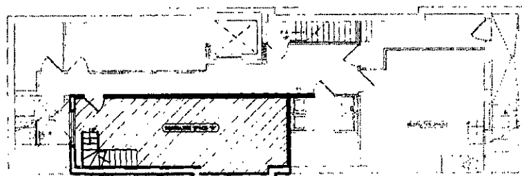
KEY CELLAR FLOOR PLAN
