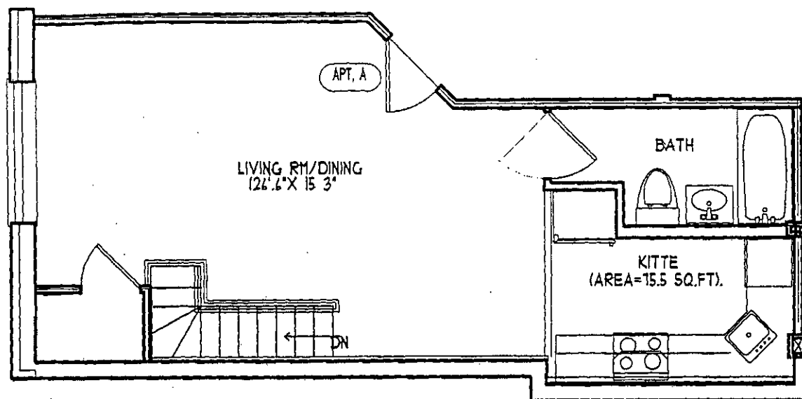
FIRST FLOOR PLAN APT. "A"
