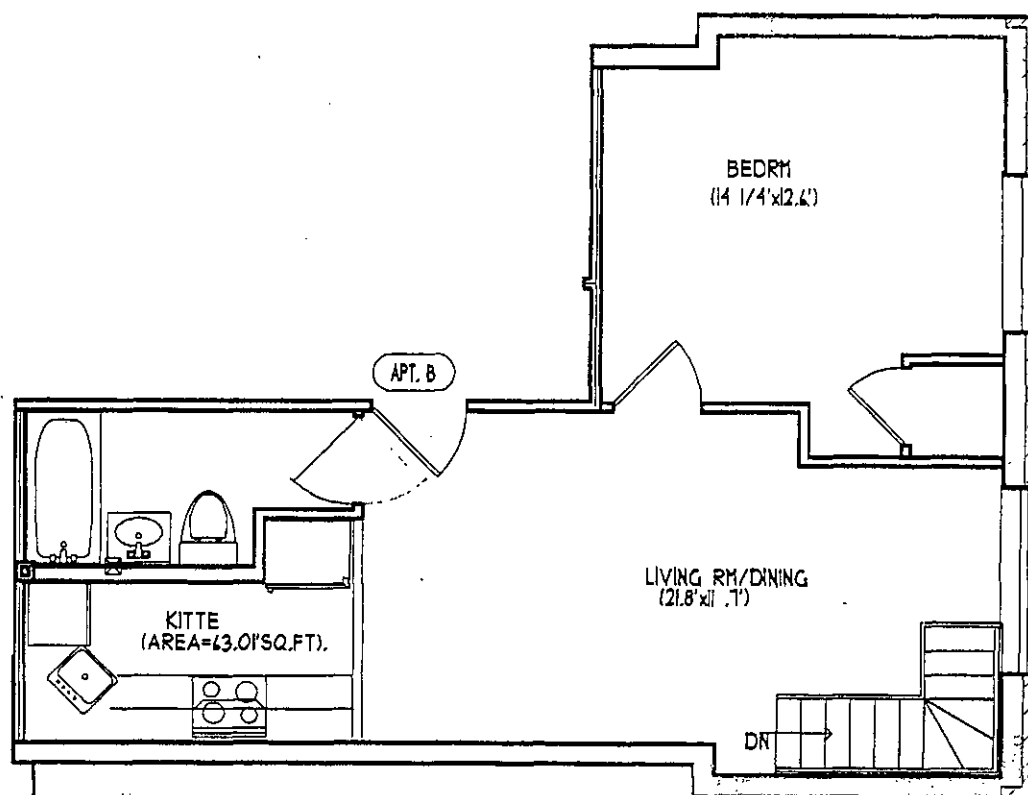
FIRST FLOOR PLAN APT. "B"
