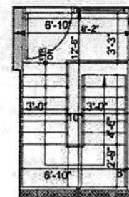
APT. 3 UL DUPLEX AREA = 41.8 S.F.
