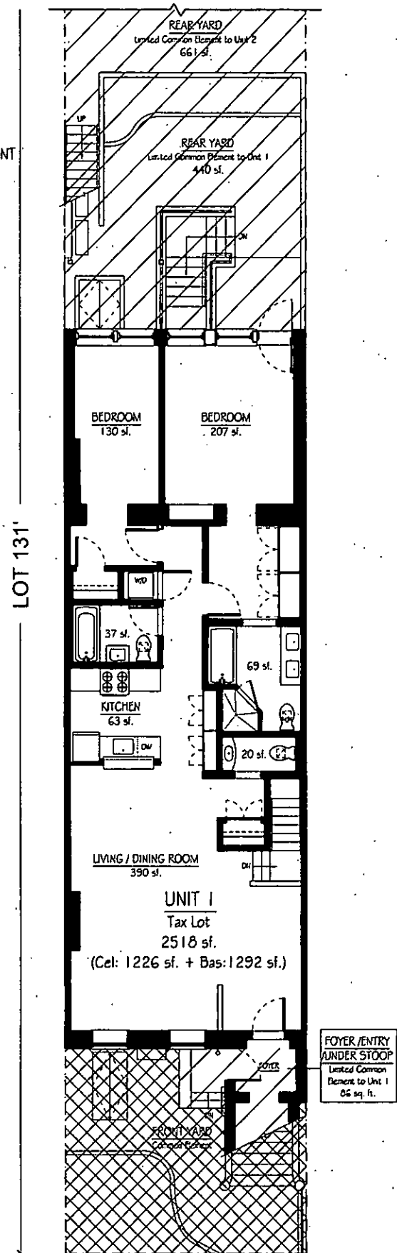
5 Basement Floor Plan 3/32" = 1'-0"
