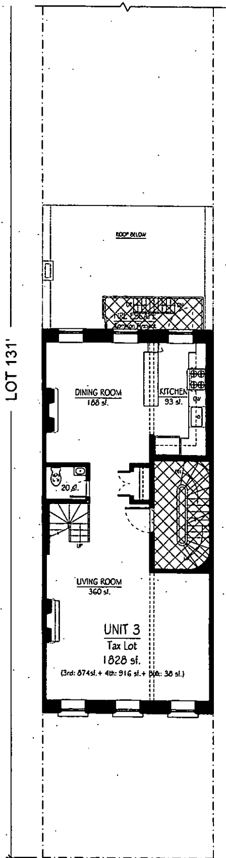
8 Third Floor Plan 3/32" = 1'-0"
