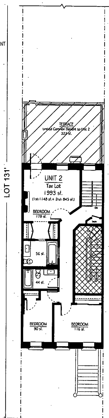
7 Second Floor Plan 3/32" = 1'-0"
