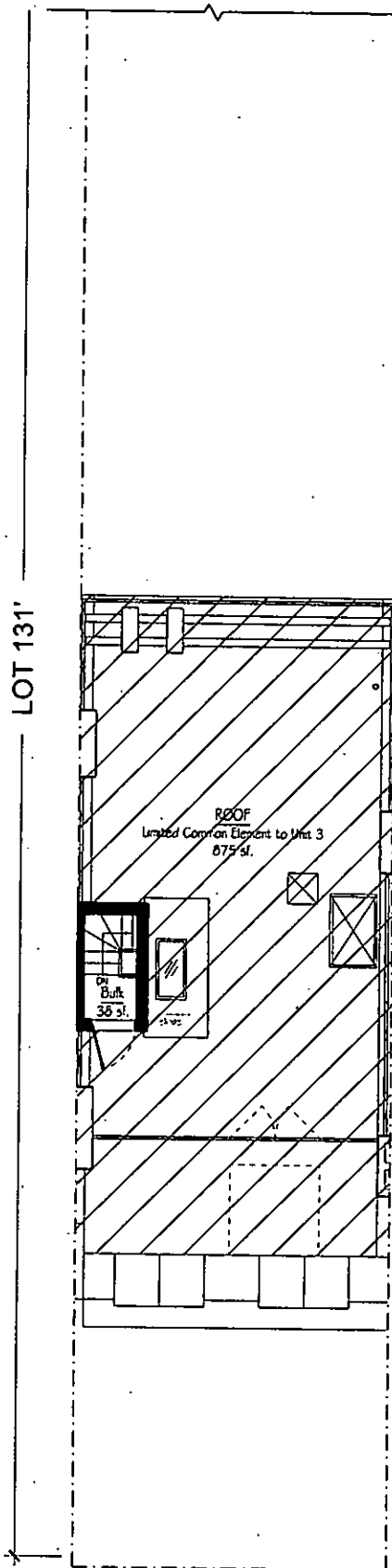
10 Roof Plan 3/32" = 1'-0"
