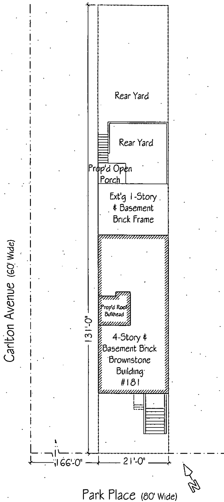
① Site Plan 1/16" = 1'-0"
