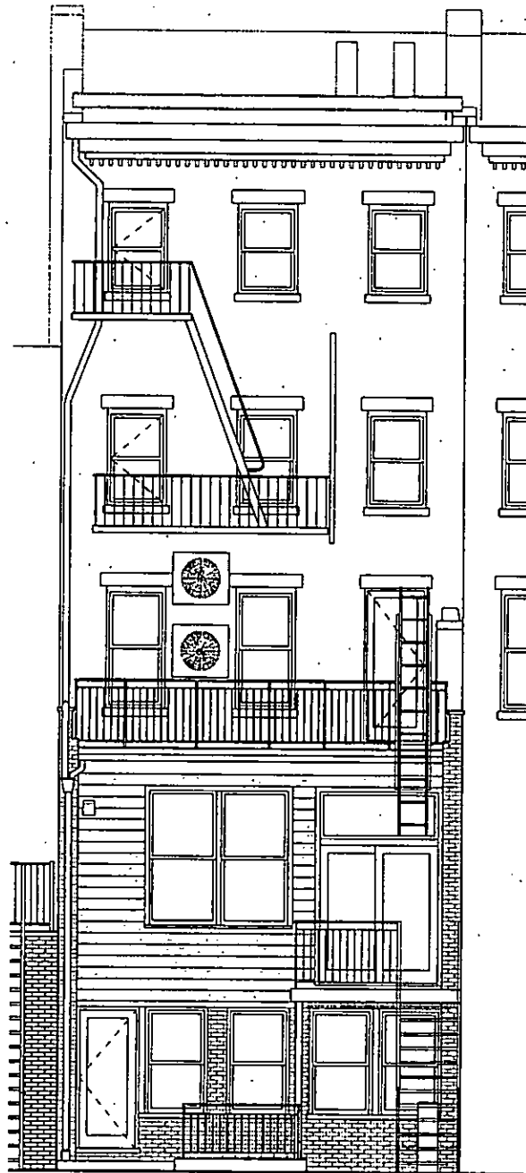
③ Rear Facade \frac{1}{8}" = 1'-0"
