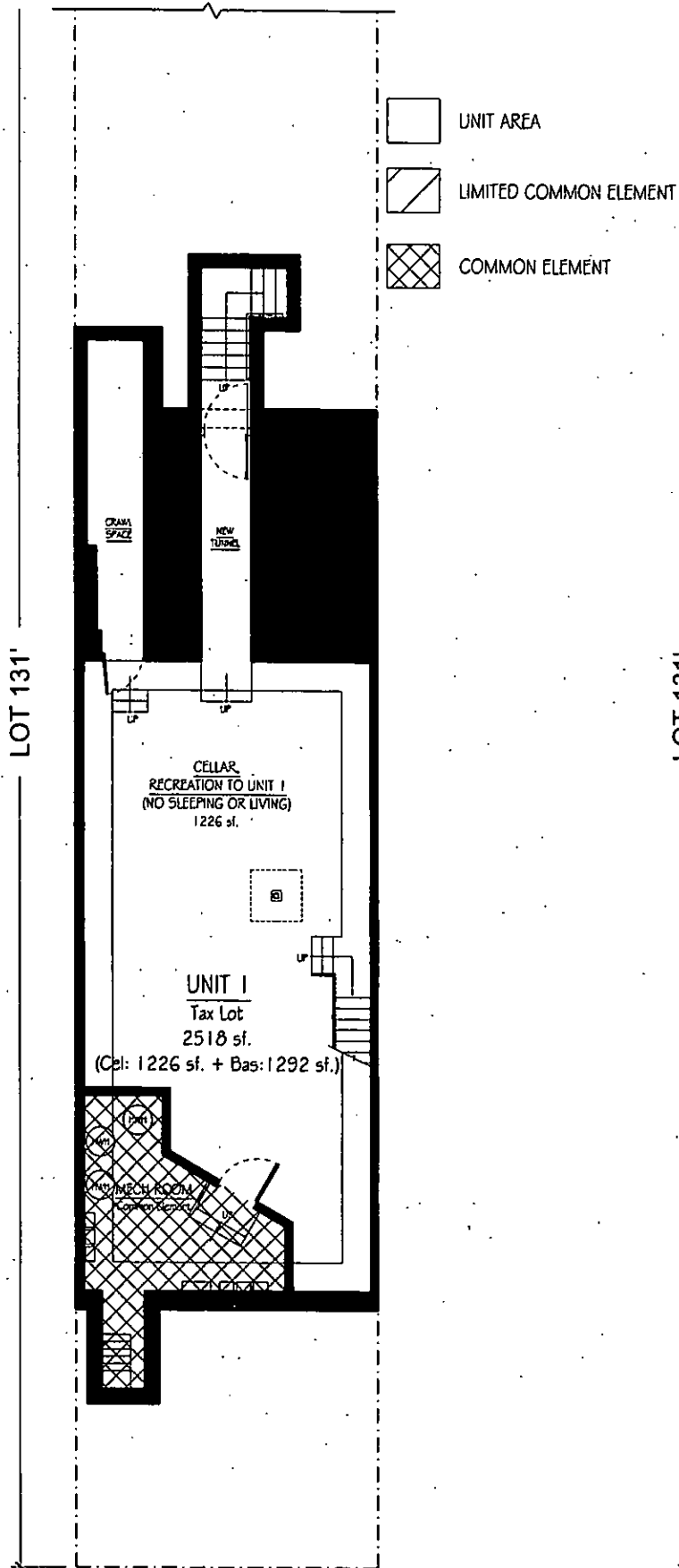
4 Cellar Floor Plan 3/32" = 1'-0"
