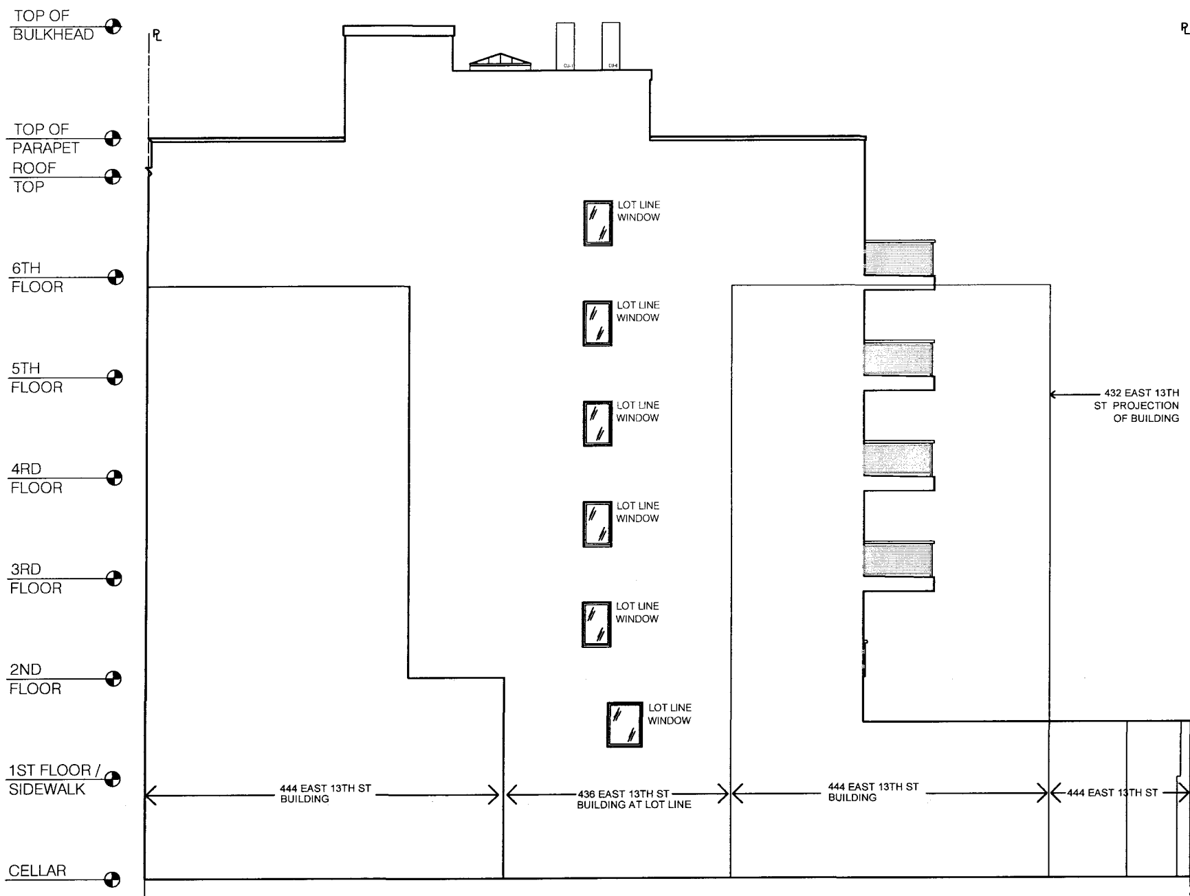
EAST ELEVATION (RIGHT SIDE)
