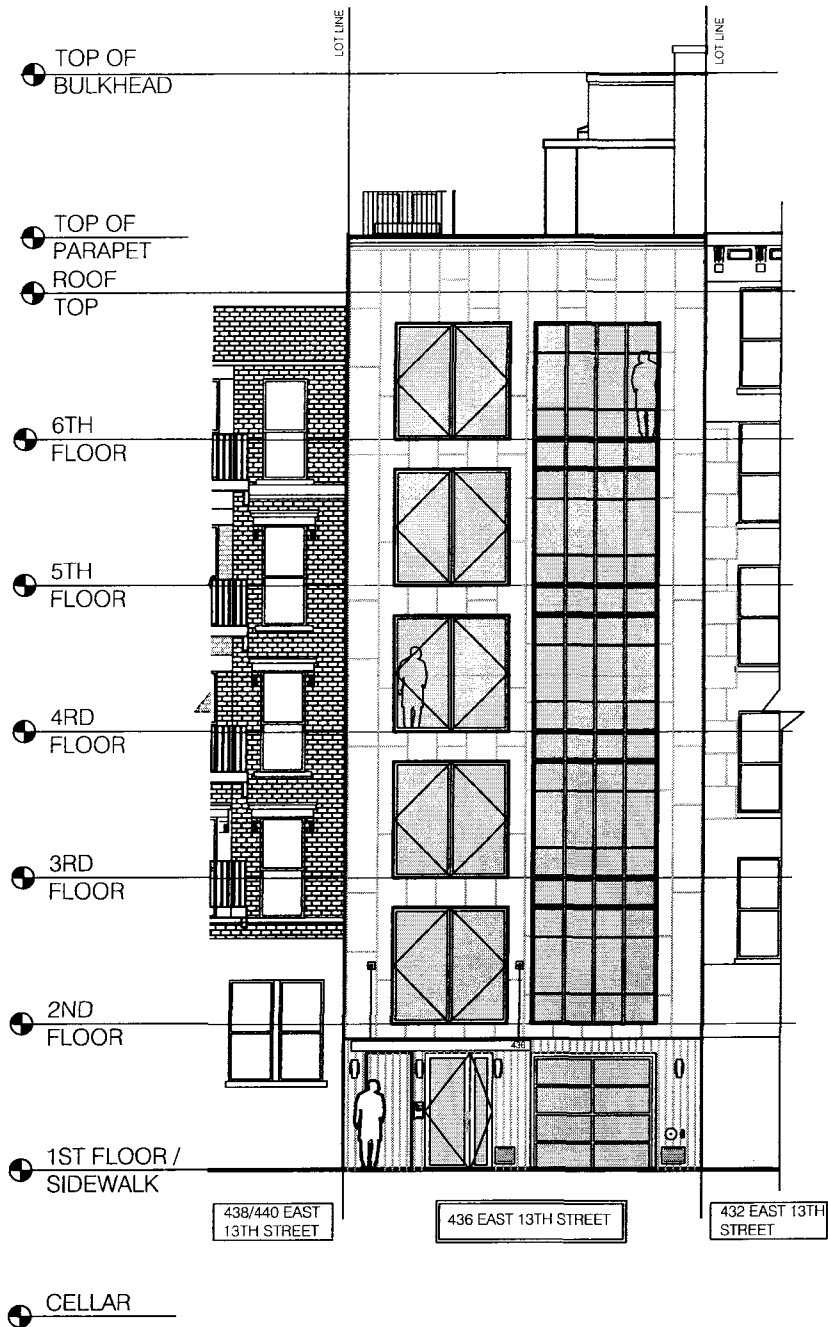
FRONT FACADE
