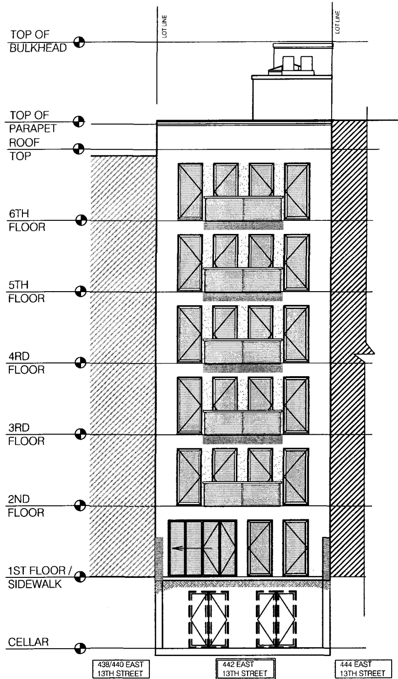
REAR FACADE
