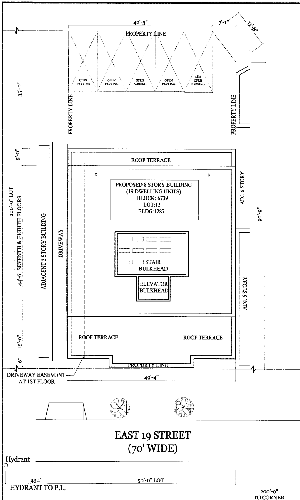
PLOT PLAN SCALE 1/16"=1'-0" 1287 EAST 19TH STREET, BROOKLYN 11230
