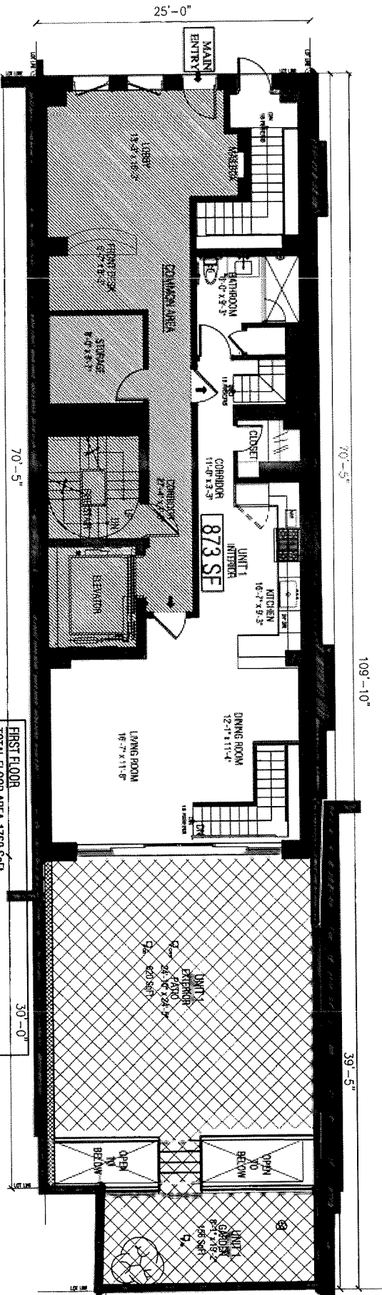
P2 FIRST FLOOR
