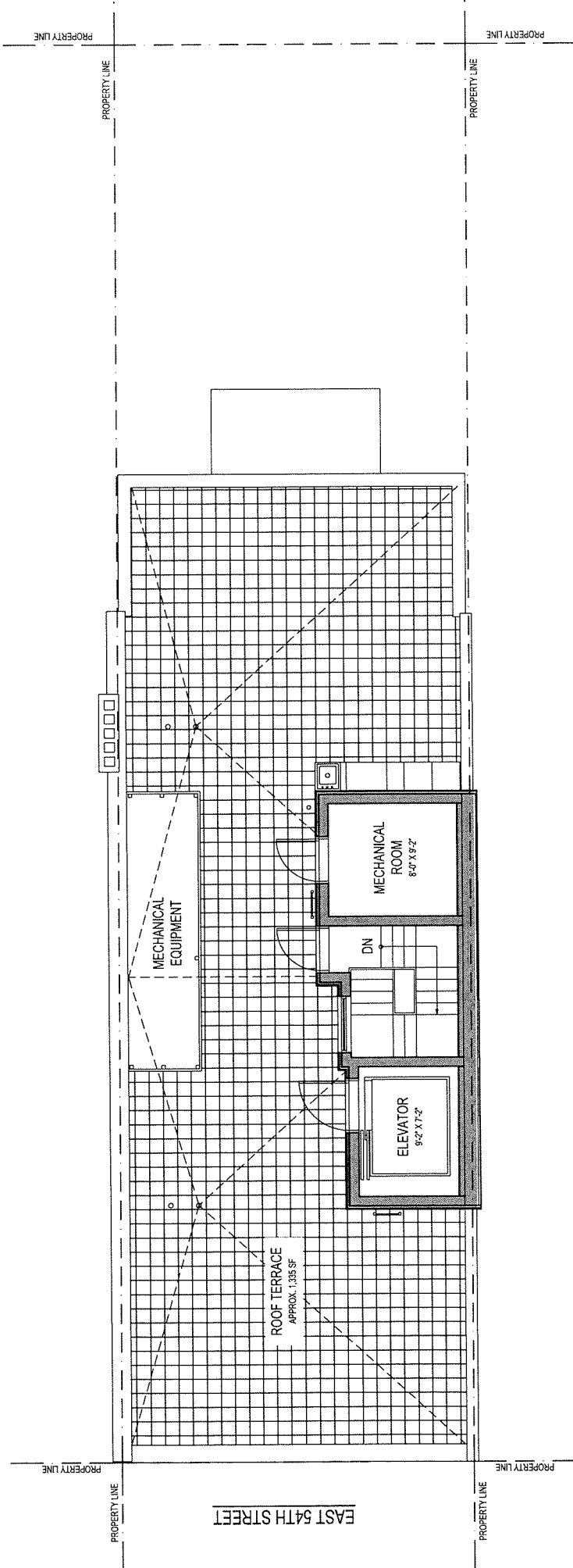
ROOF PLAN
