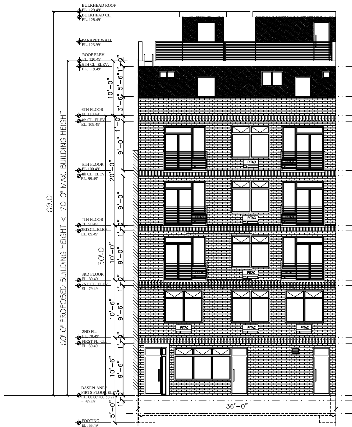
FRONT ELEVATION
