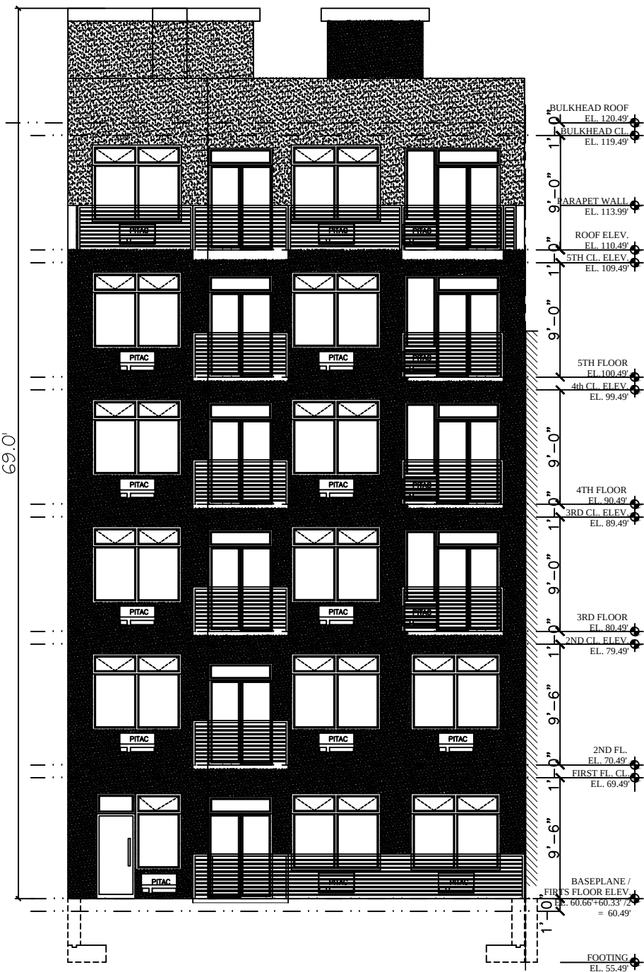
REAR ELEVATION
