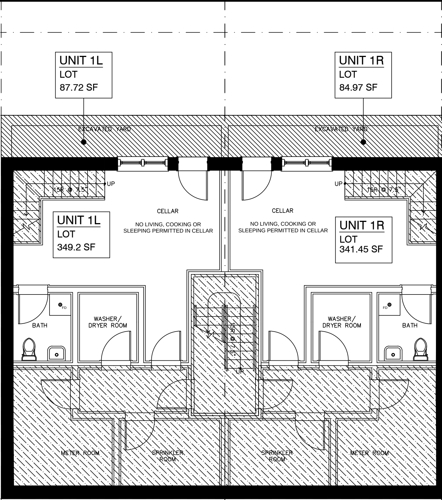
216 Pulaski st CELLAR FLOOR PLAN
