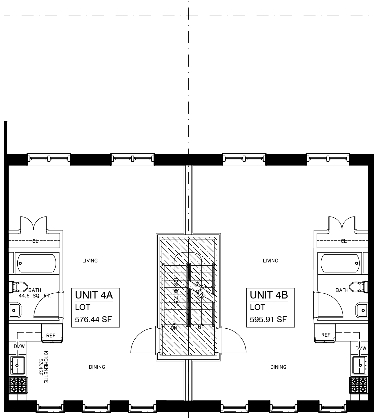
210 Pulaski st FOURTH FLOOR PLAN
