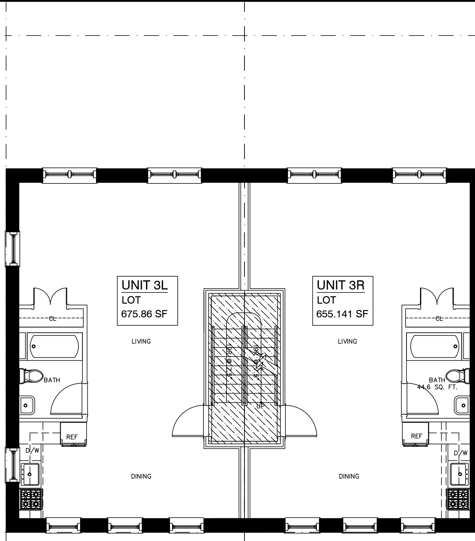
216 Pulaski st THIRD FLOOR PLAN
