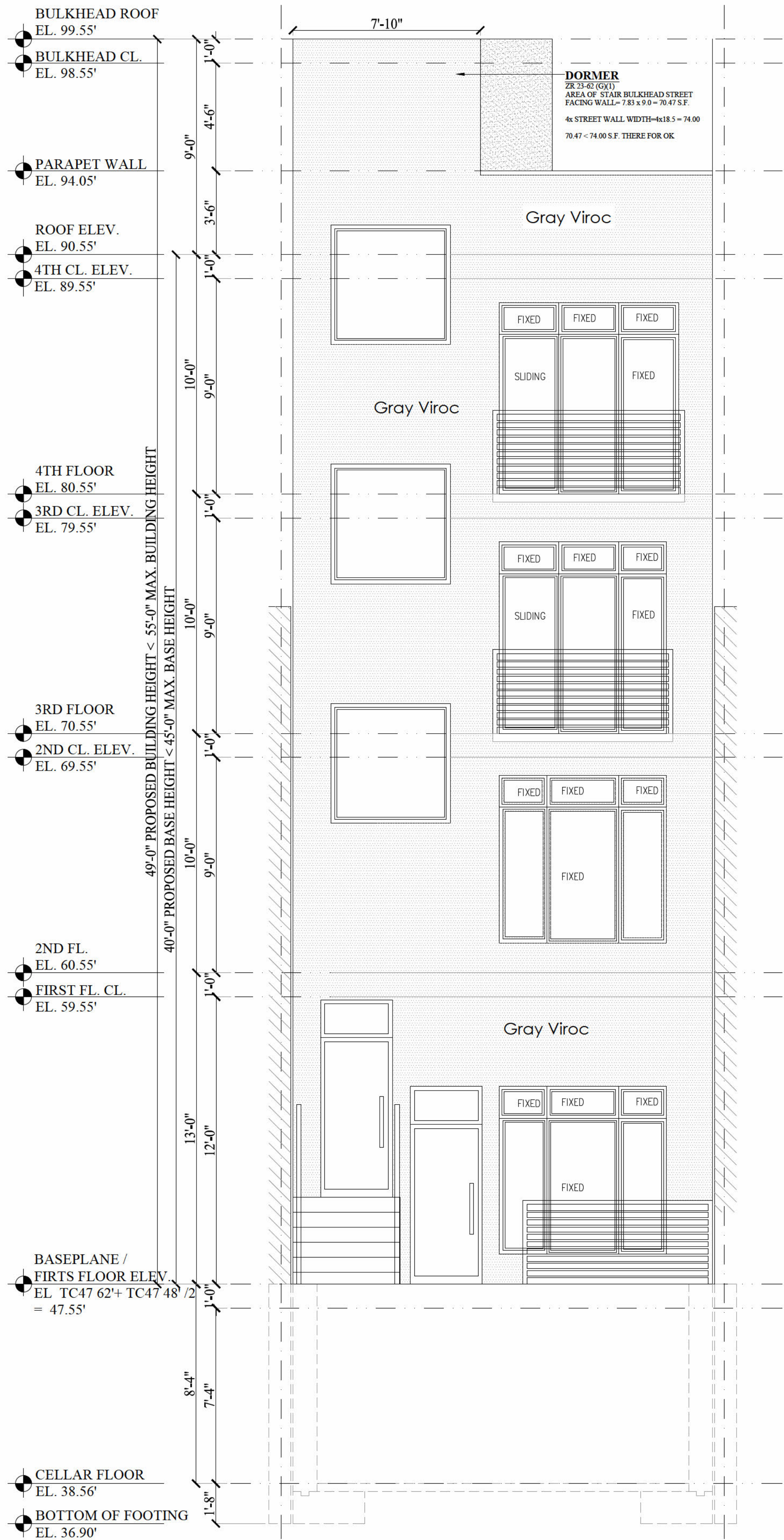
FRONT ELEVATION
