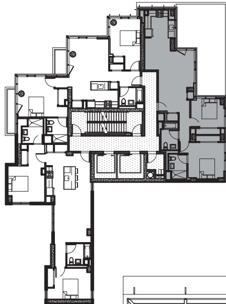
10TH FLOOR PLAN
