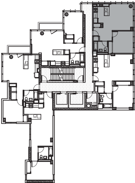
5TH FLOOR PLAN KEY SCALE: 1/32" = 1'-0"
