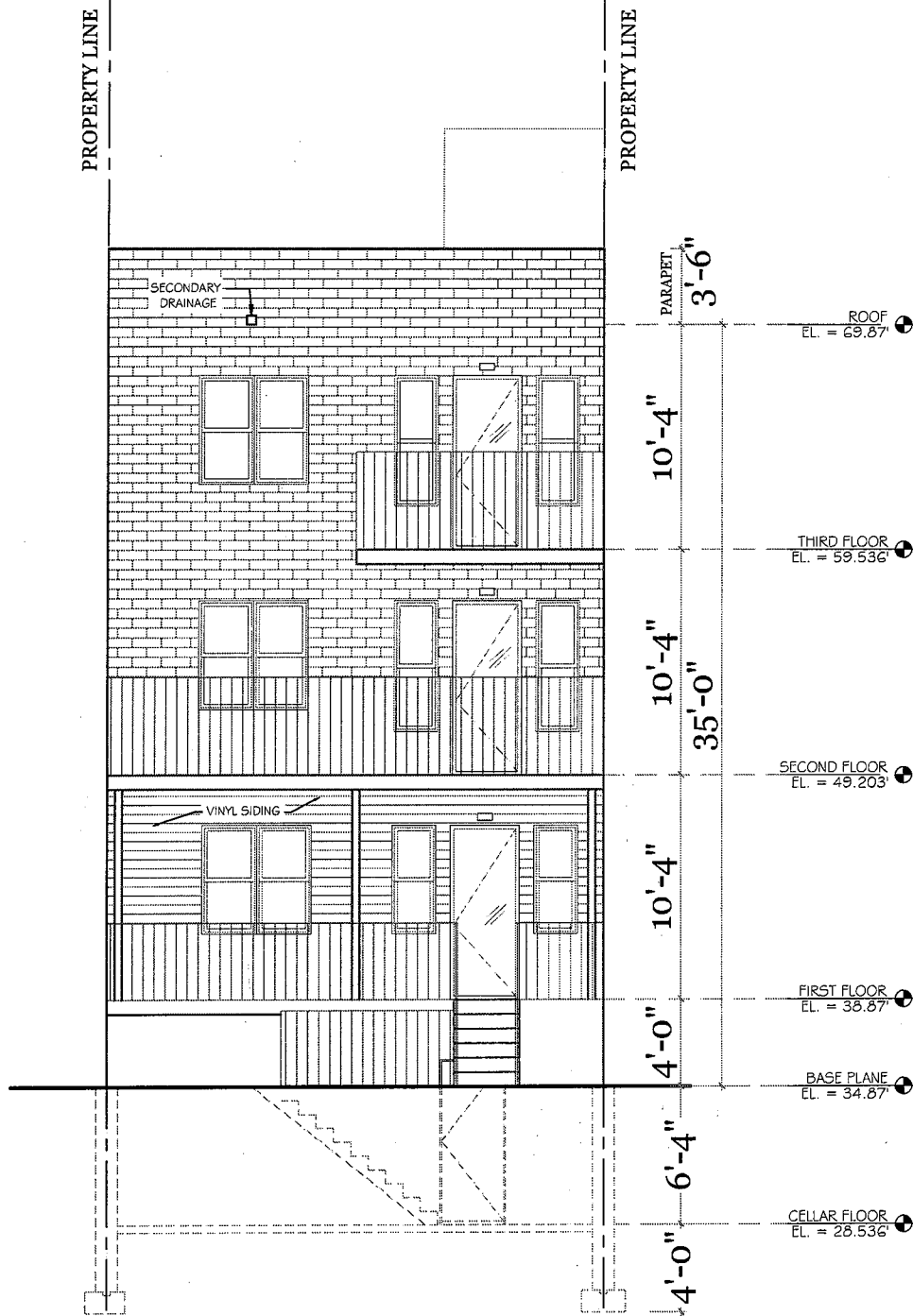
REAR ELEVATION SCALE 1/8" = 1'-0"
