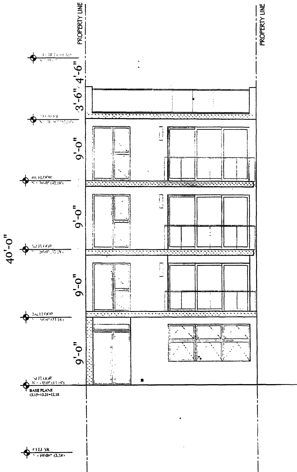
FRONT ELEVATION SCALE 1/8" = 1'-0"
