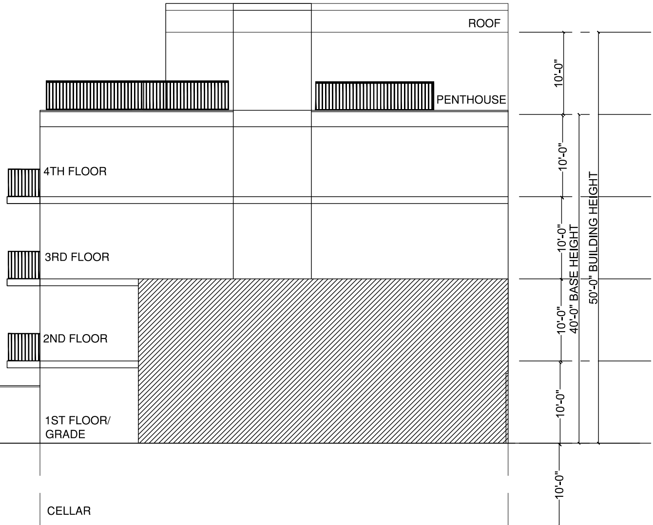
WEST ELEVATION PLAN
