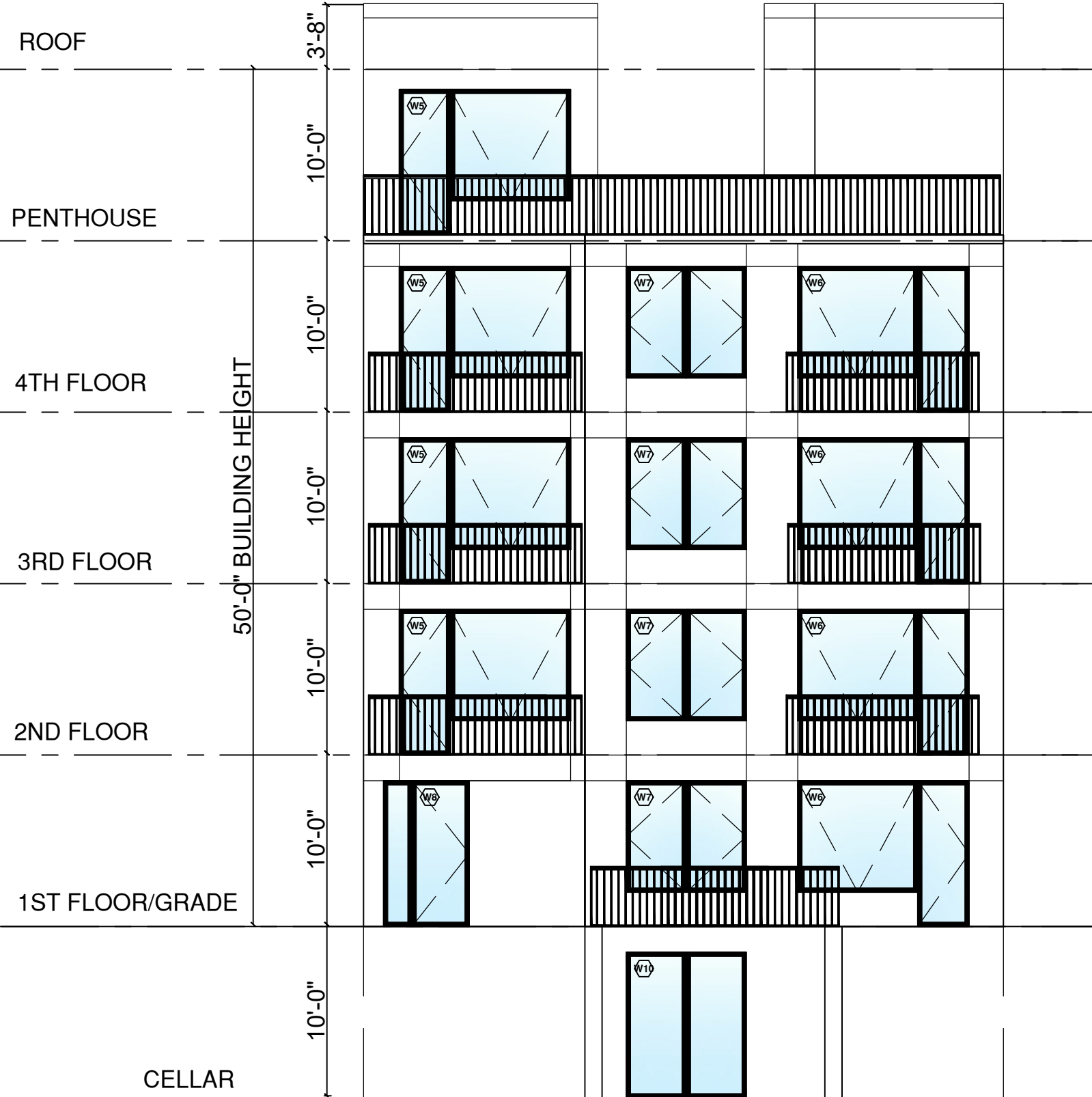
REAR ELEVATION PLAN
