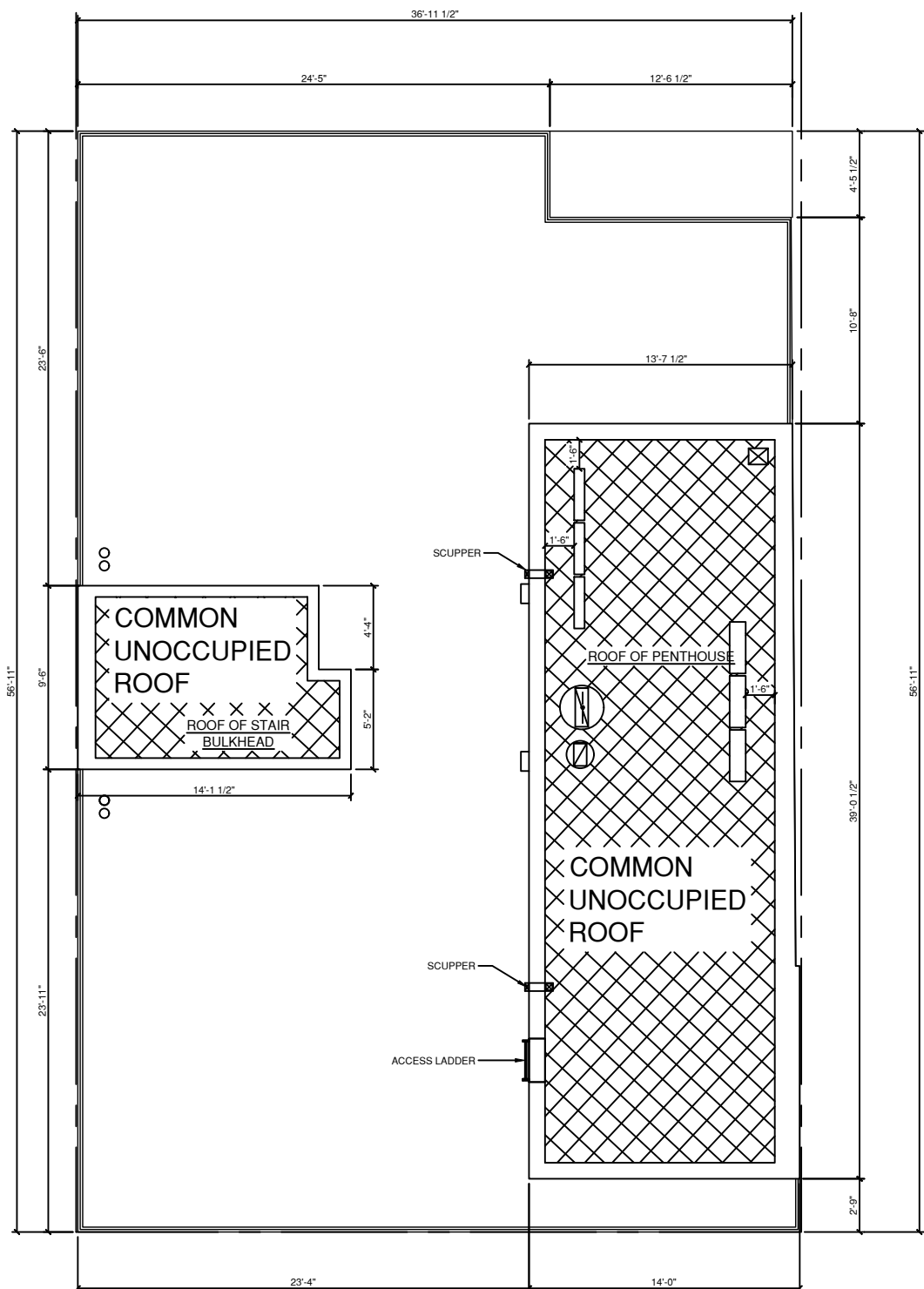
ROOF FLOOR PLAN
