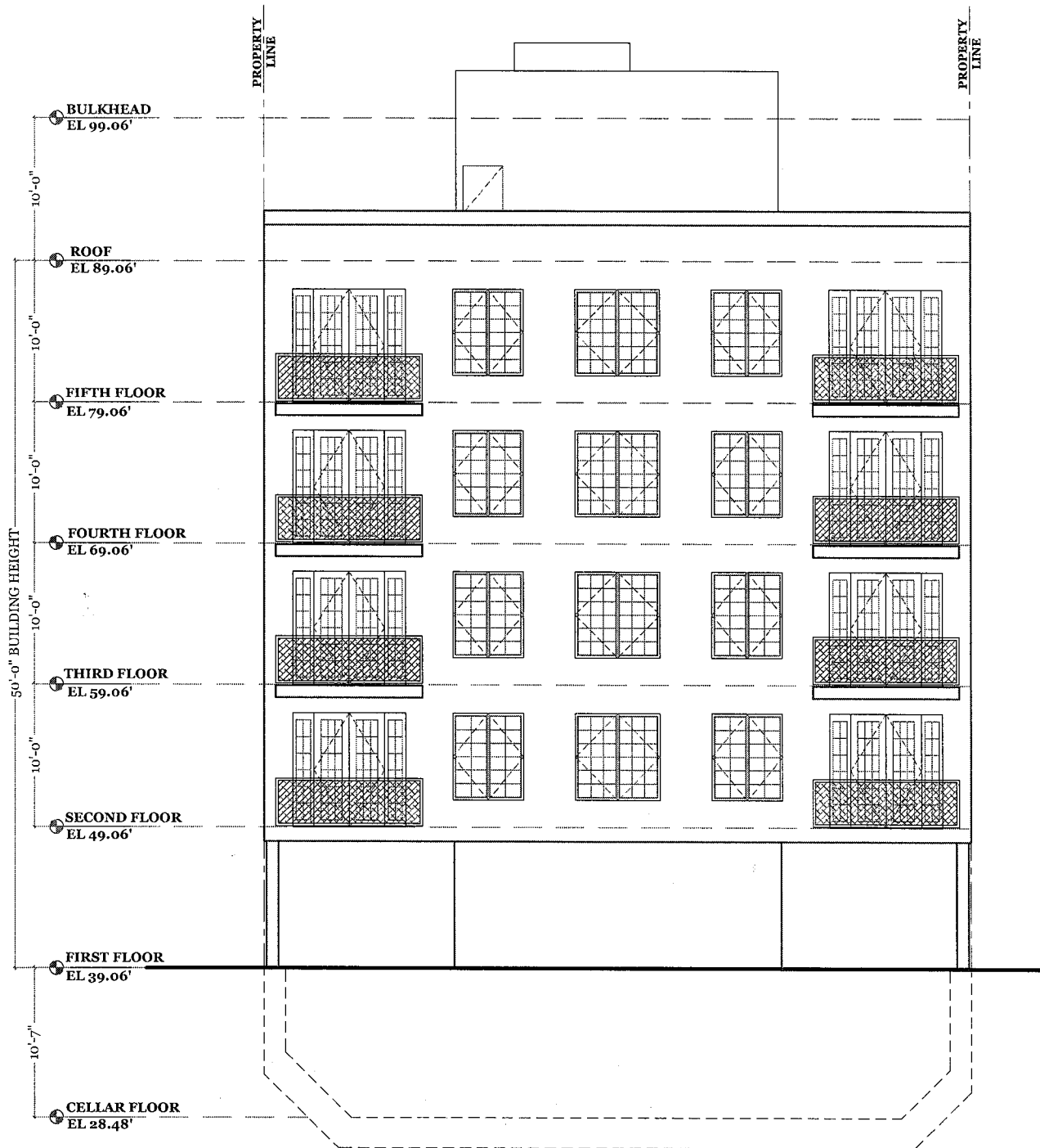
REAR ELEVATION SCALE 3/32"=1'-0"
