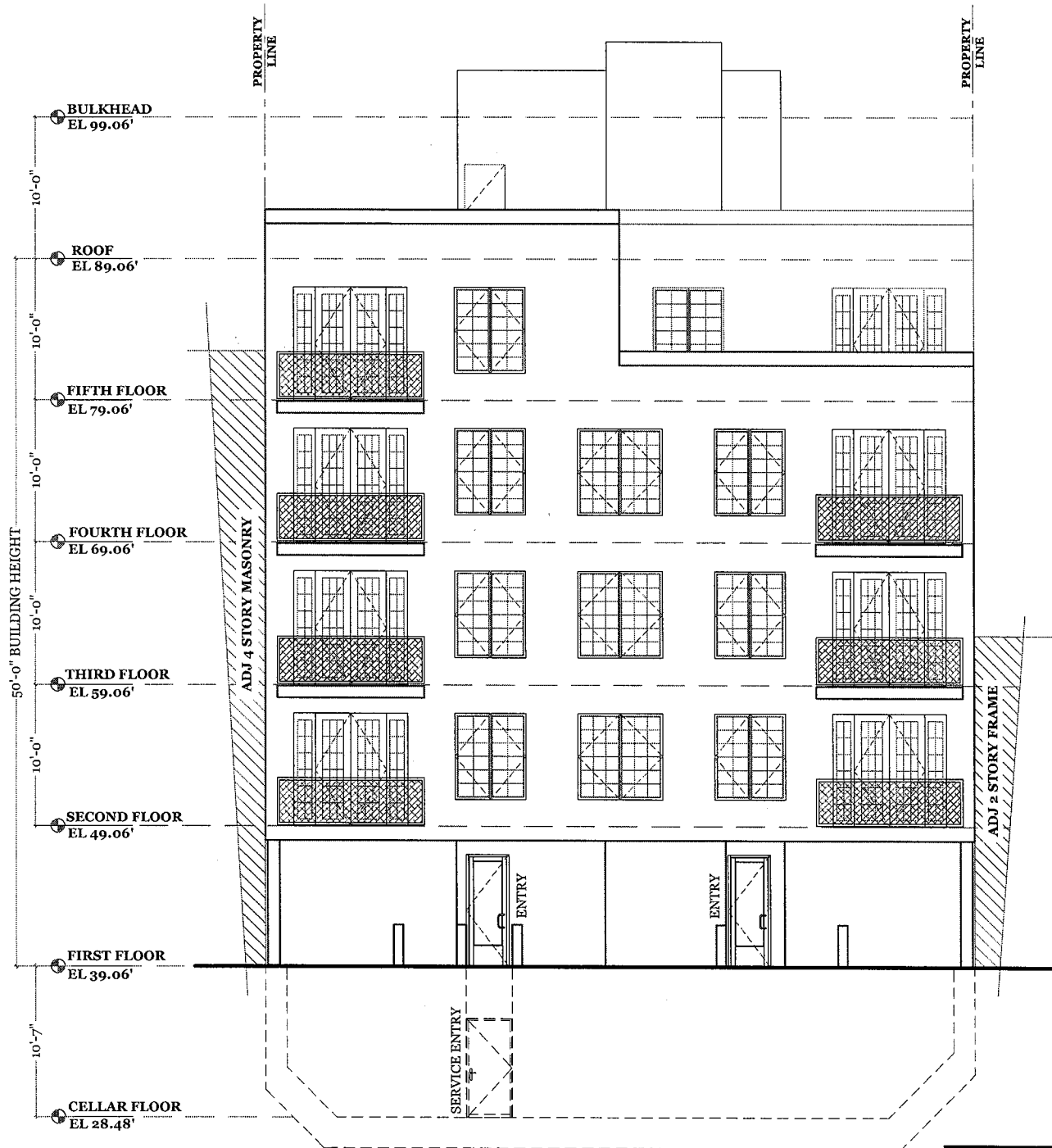
FRONT ELEVATION SCALE 3/32"=1'-0"
