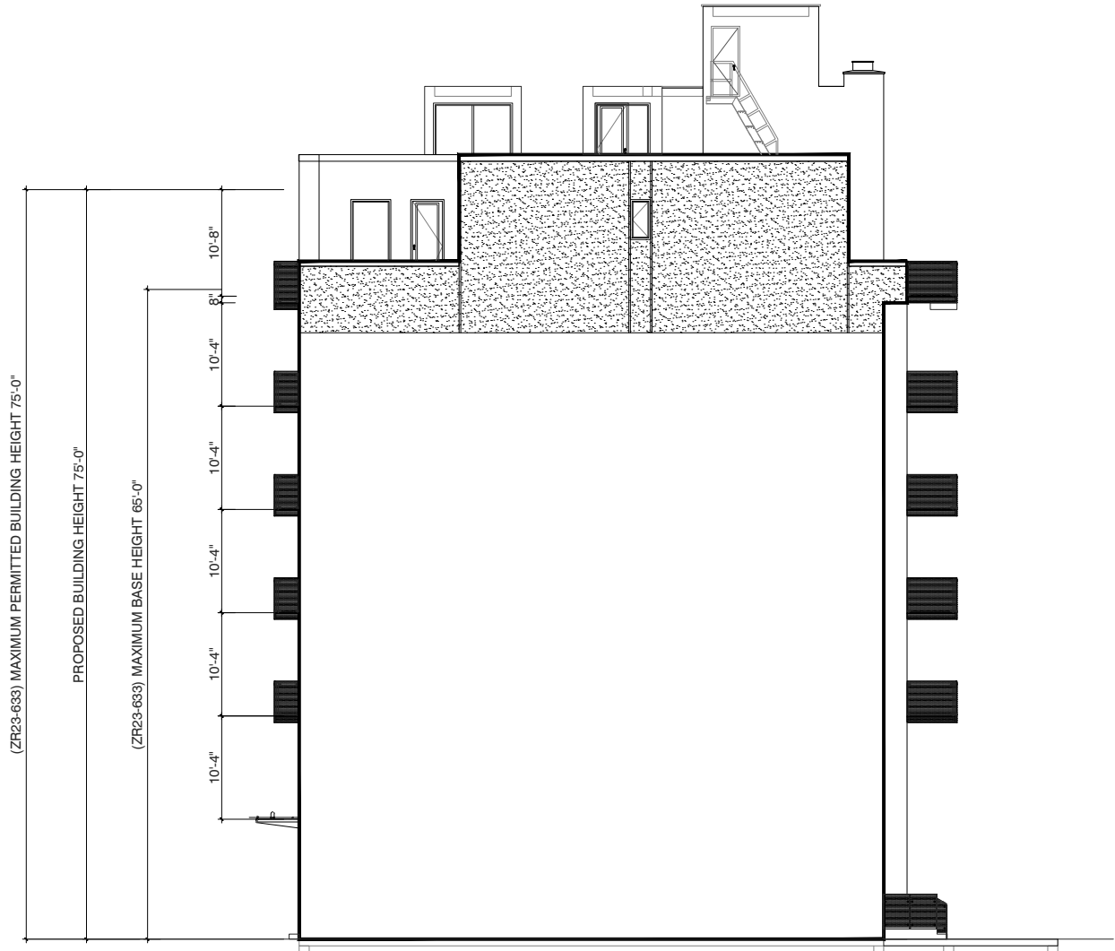
EAST ELEVATION
