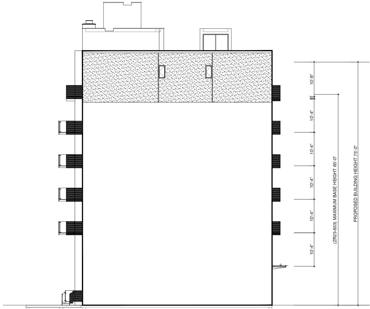
WEST ELEVATION
