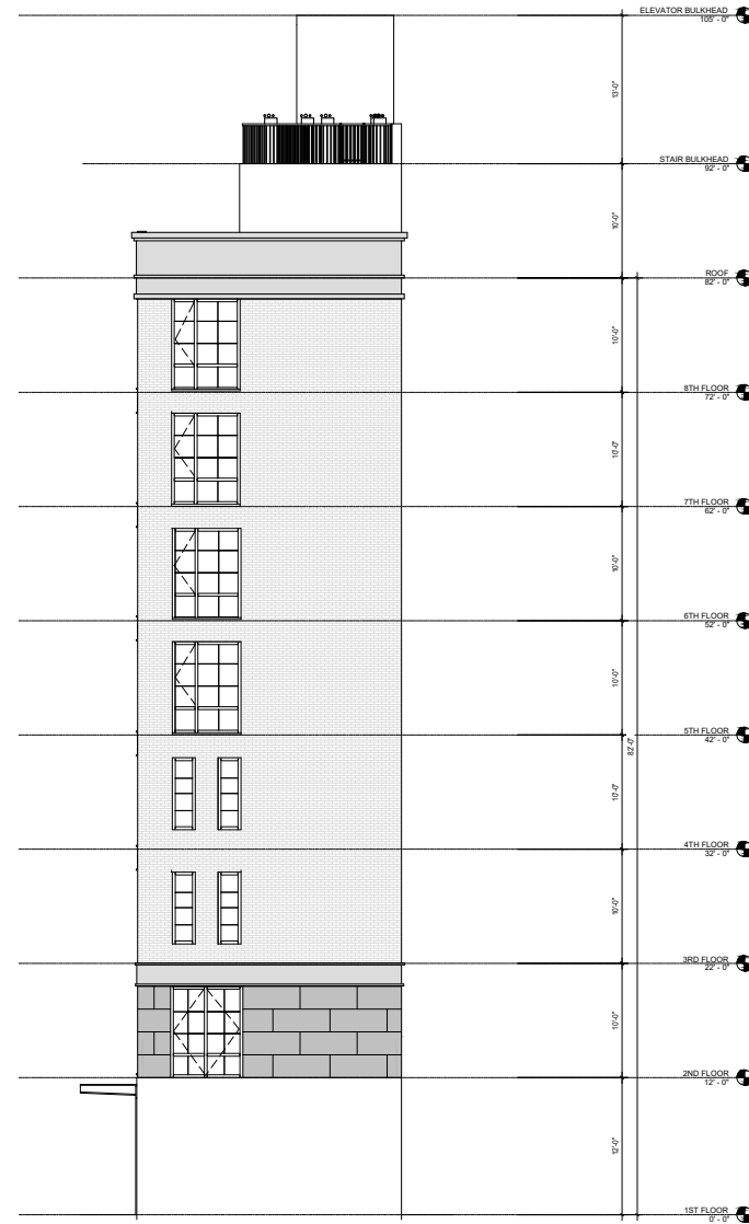
NORTH ELEVATION
