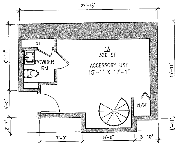
UNIT 1A (APARTMENT WITH ACCESSORY USE CELLAR - LOWER LEVEL)
