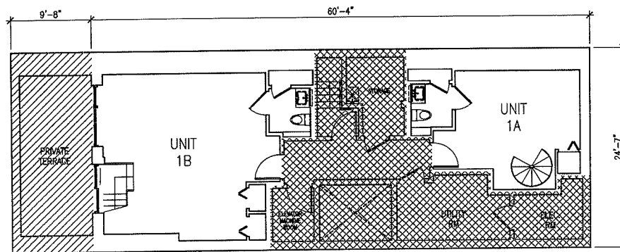
CELLAR PLAN
