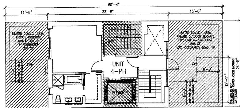
5TH FLOOR PLAN (DUPLEX UPPER LEVEL)
