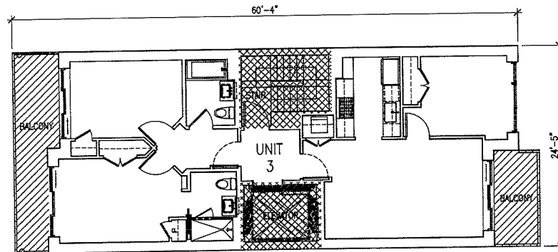
3RD FLOOR PLAN
