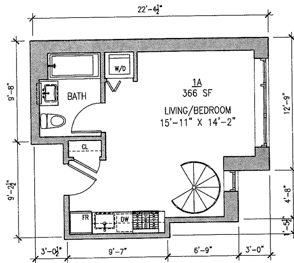
UNIT 1A (APARTMENT WITH ACCESSORY USE CELLAR - 1ST FLOOR)
