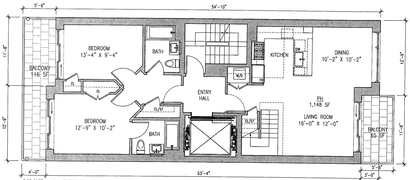
UNIT 4 - PENTHOUSE (DUPLEX 4TH FLOOR LEVEL)
