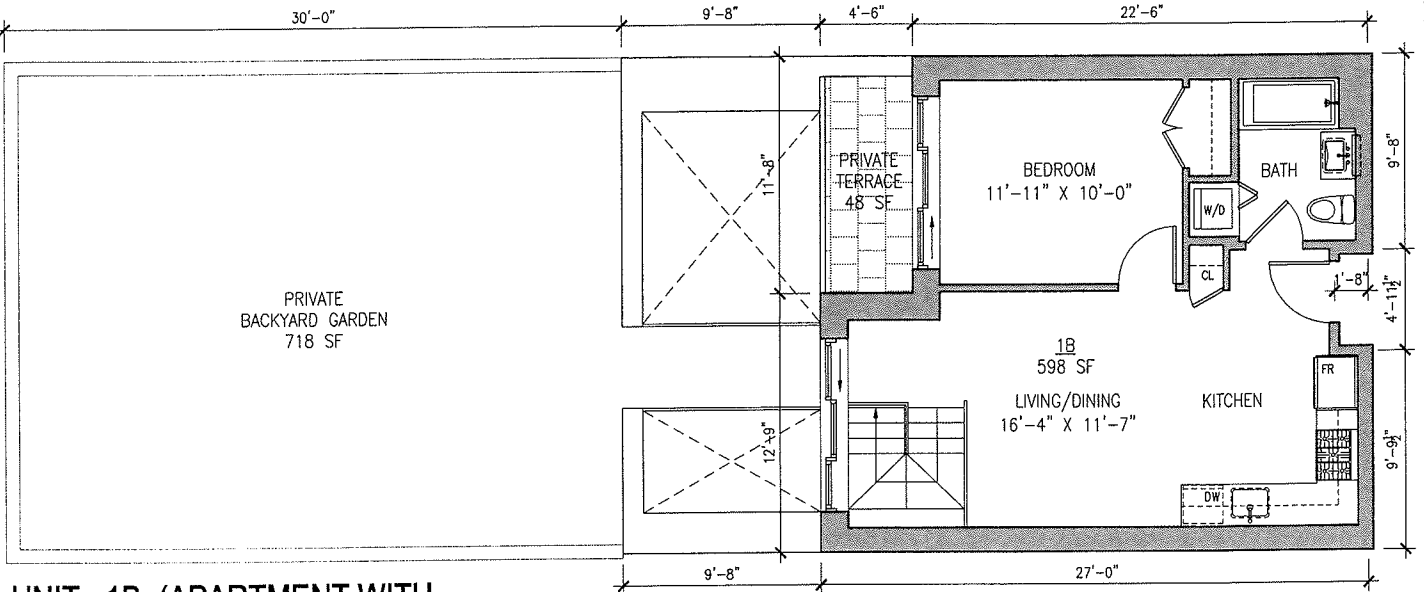
UNIT 1B (APARTMENT WITH ACCESSORY USE CELLAR - 1ST FLOOR)
