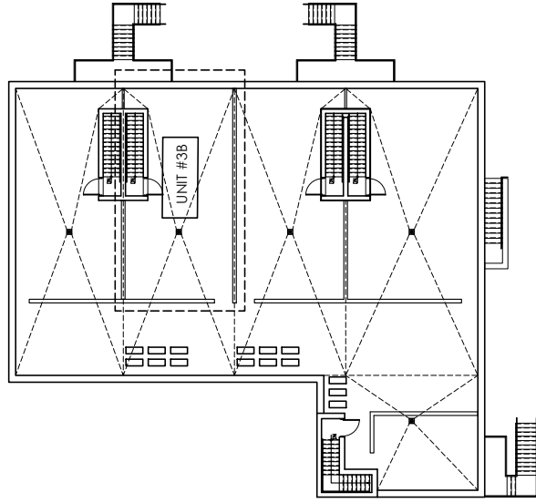
THIRD FLOOR KEY PLAN N.T.S
