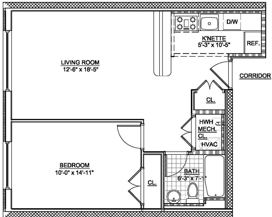
ONE BEDROOM GROSS FLOOR AREA: 676 S.F.
