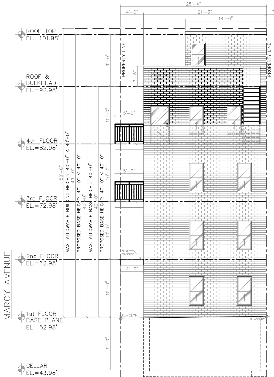
QUINCY STREET FRONT ELEVATION PLAN
