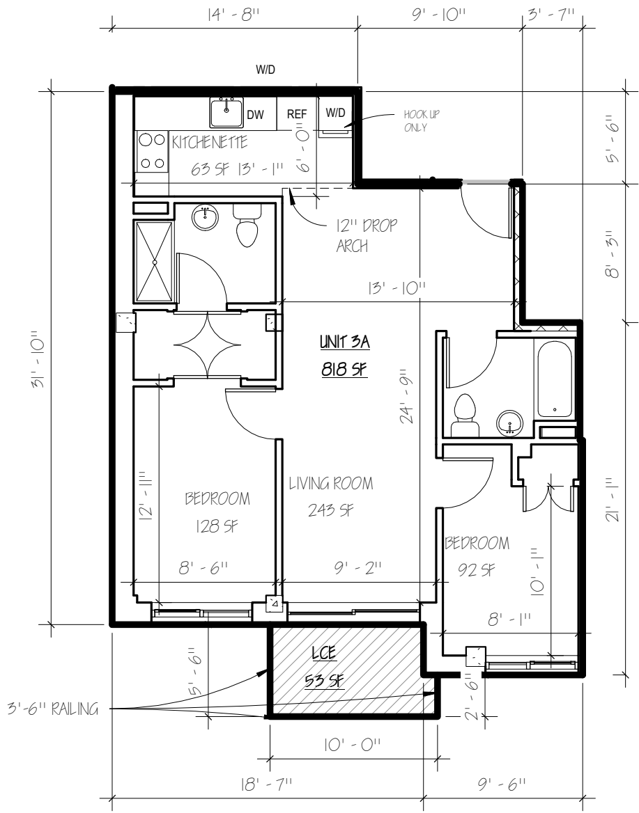
1 3 FL - 7 FL UNIT A 1/8" = 1'-0"
