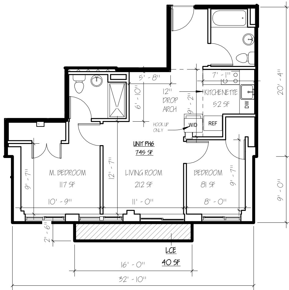
1 9 FL UNIT PH6 1/8" = 1'-0"
