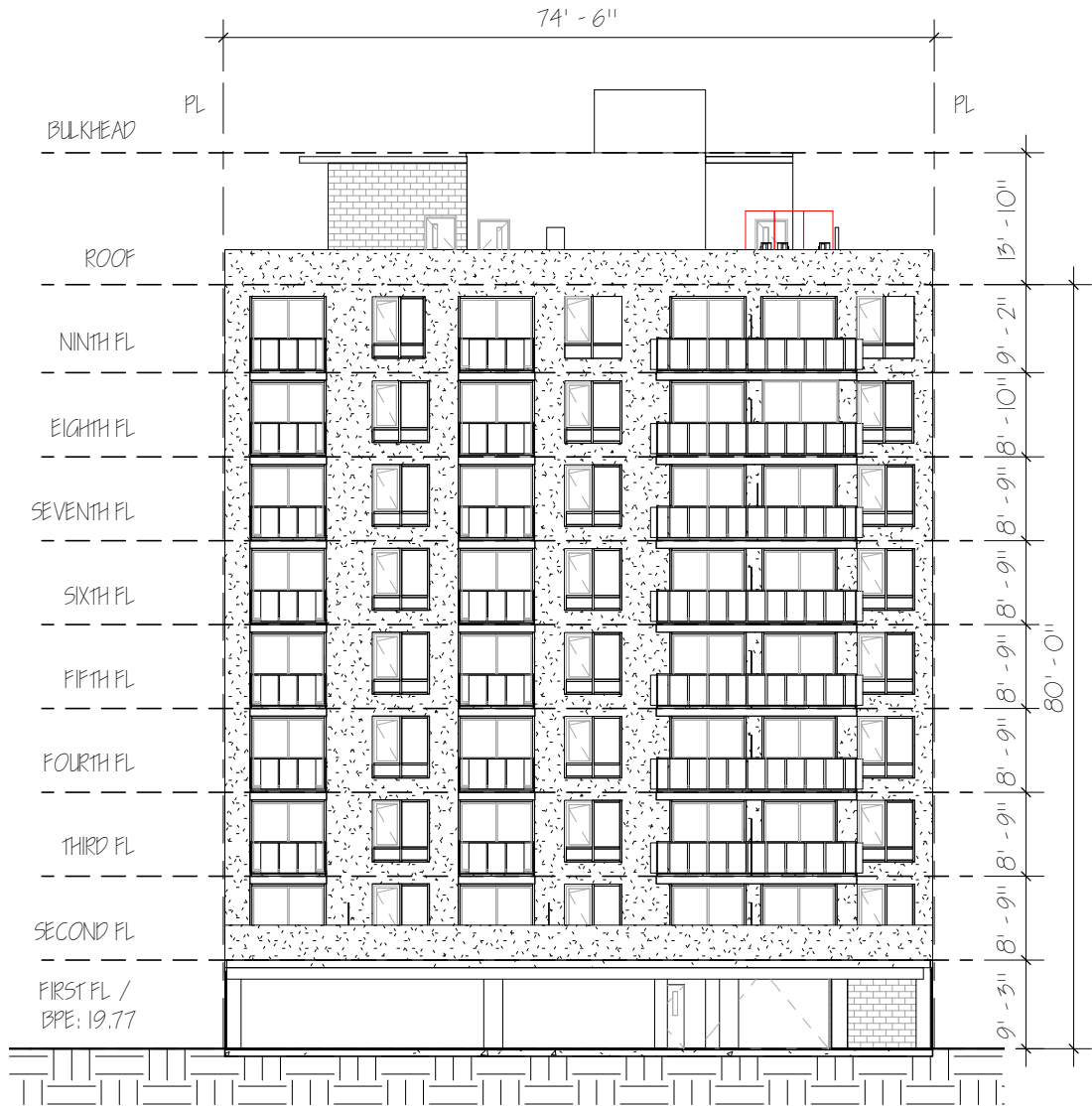
1 REAR ELEVATION - CONDO 1" = 20'-0"
