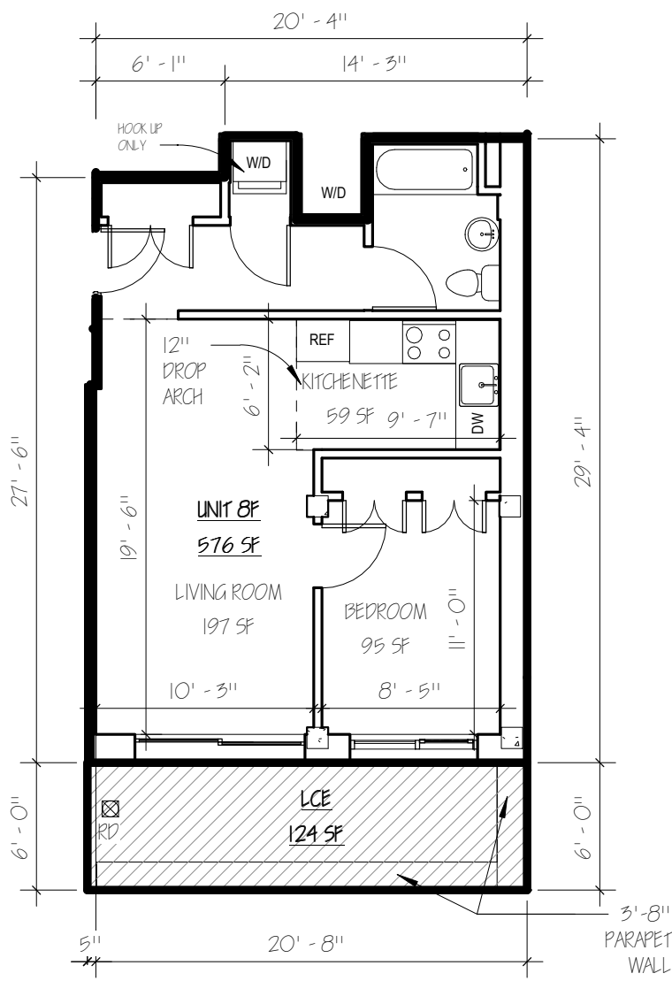
1 8 FL UNIT 8F 1/8" = 1'-0"
