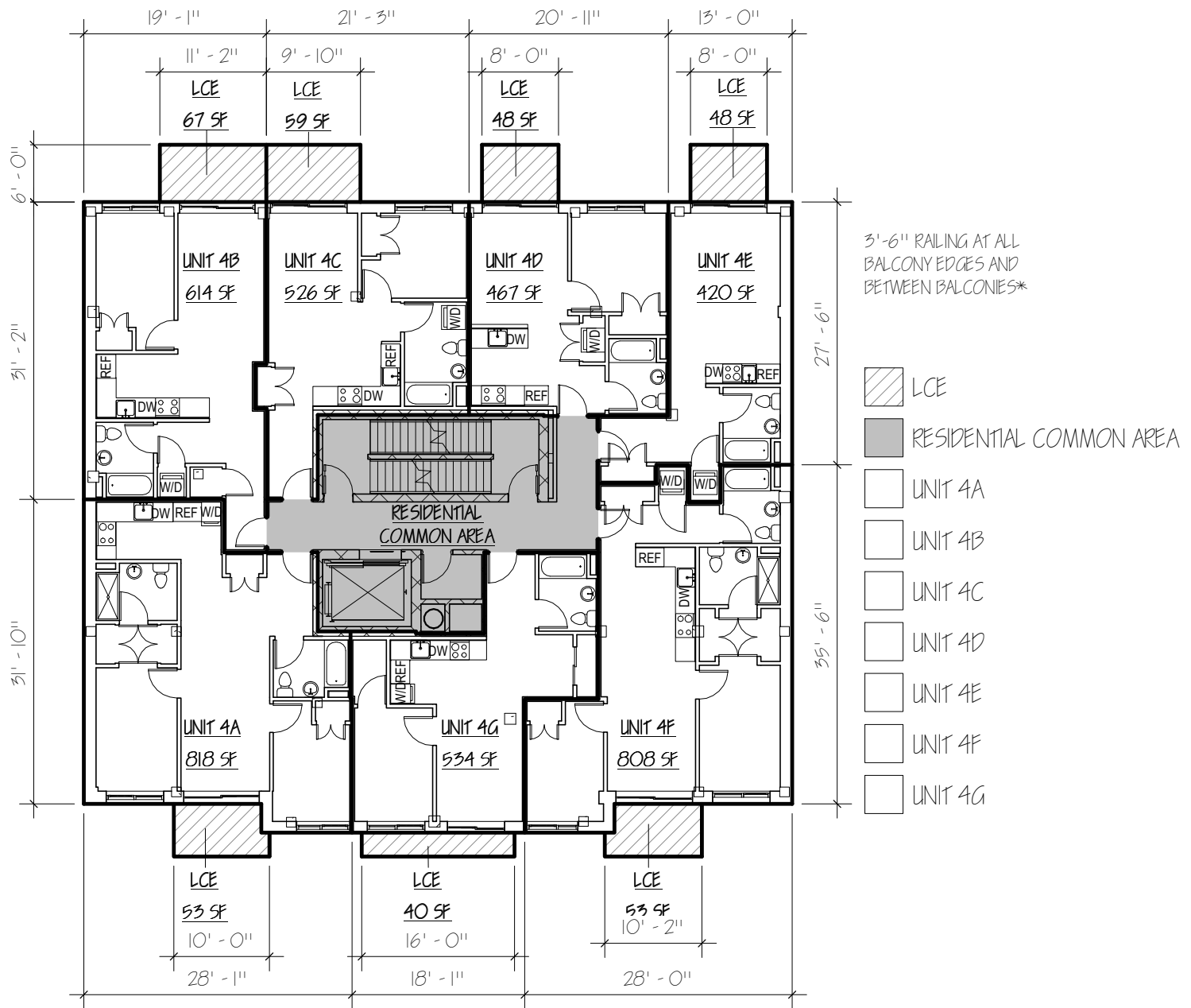
1 04-FOURTH FL. 1/16" = 1'-0"
