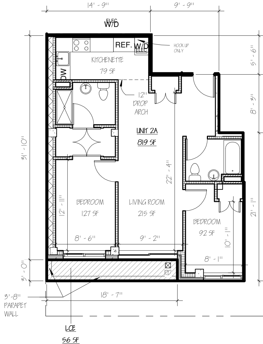
1 2 FL UNIT A 1/8" = 1'-0"
