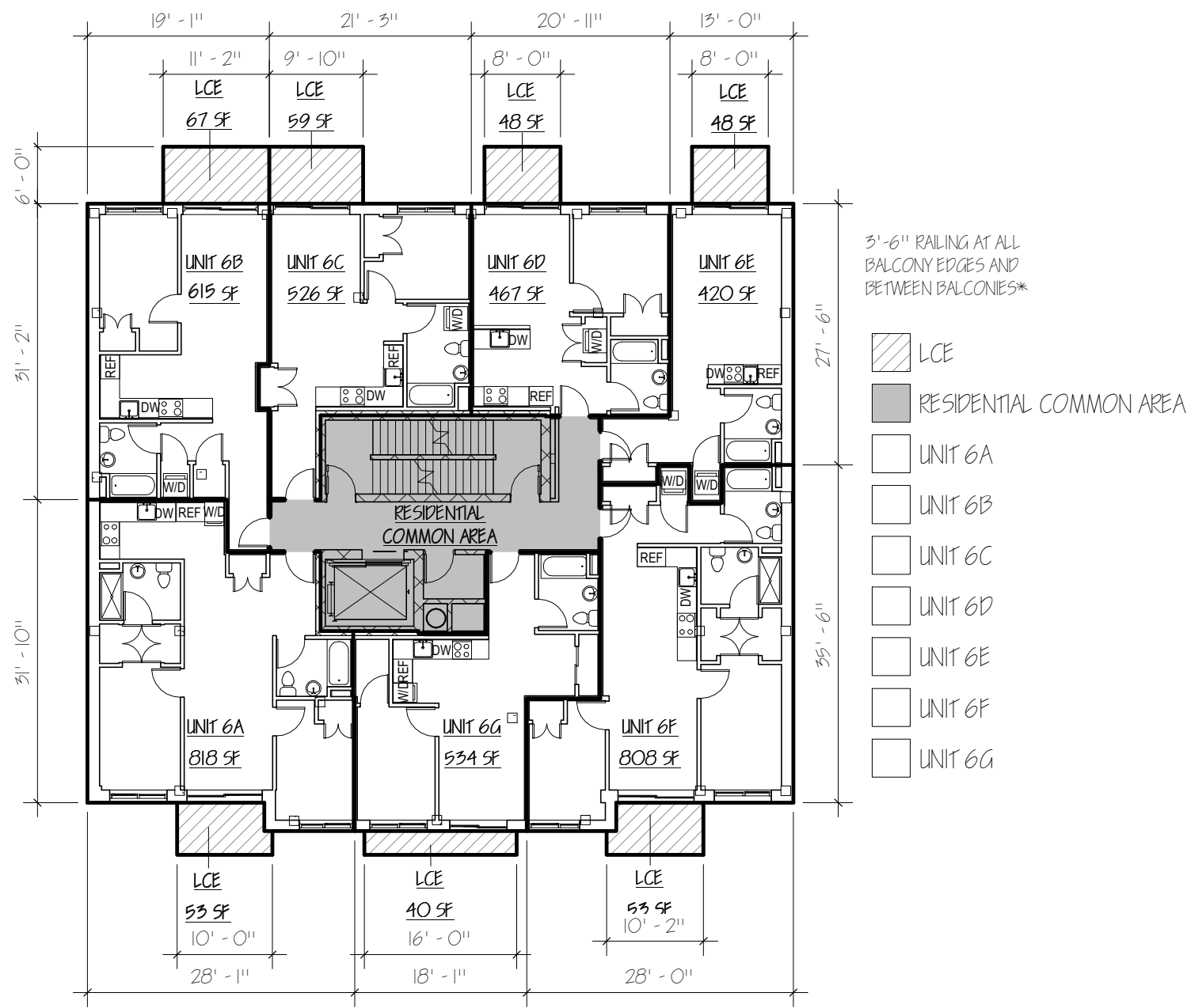
1 06-SIXTH FL. 1/16" = 1'-0"
