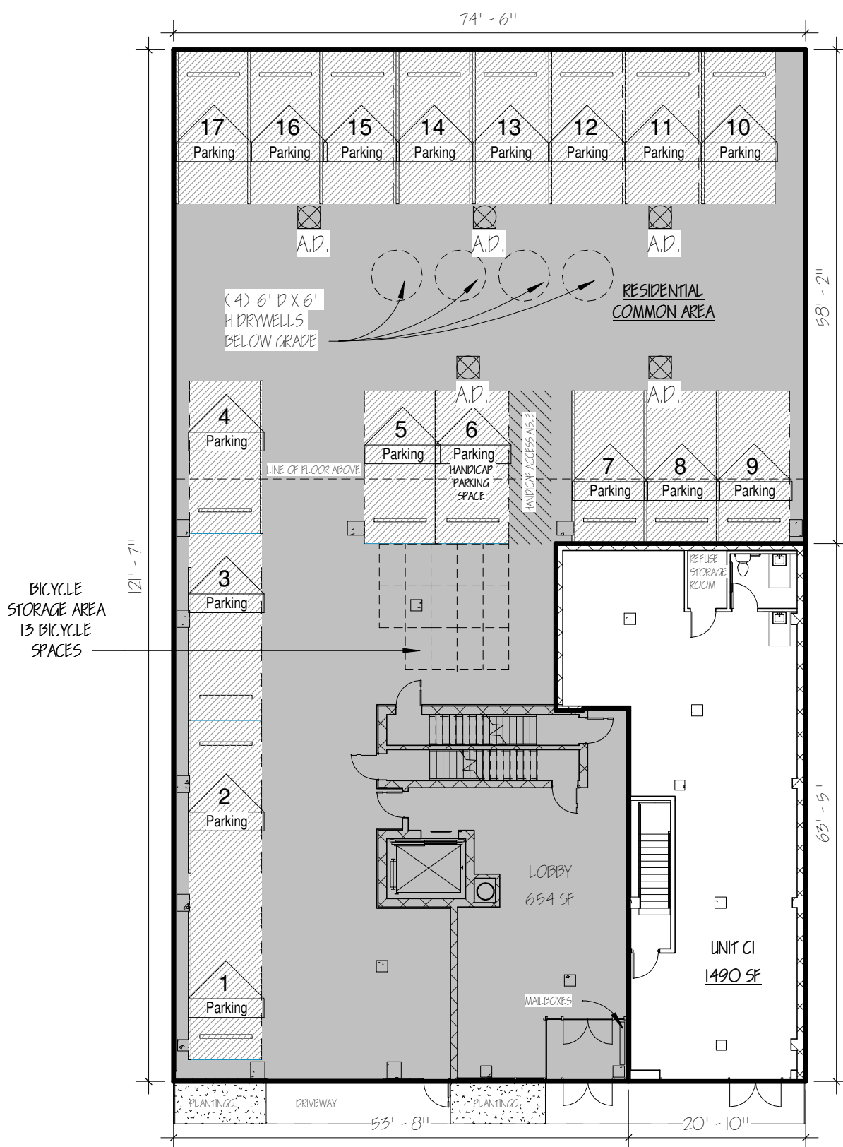
1 01-FIRST/GRADE FL. / BPE 1/16" = 1'-0"
