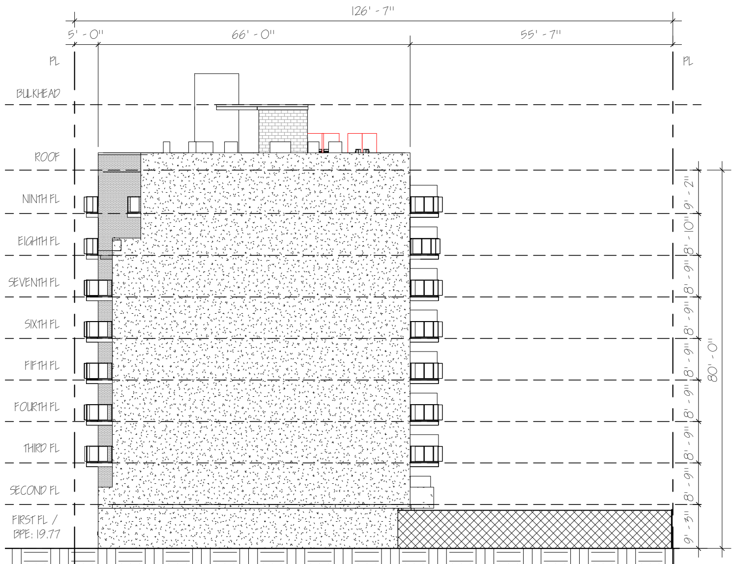
1 RIGHT SIDE ELEVATION - CONDO 1" = 20'-0"
