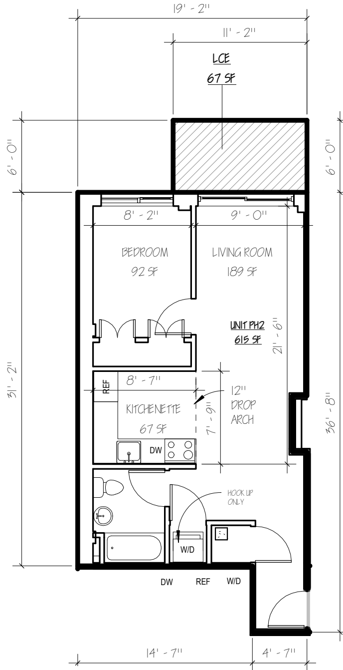
1 9 FL UNIT PH2 1/8" = 1'-0"
