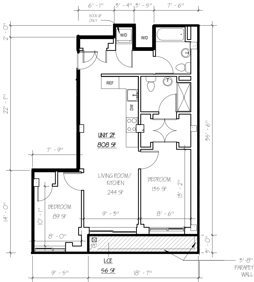
1 2 FL UNIT F 1/8" = 1'-0"
