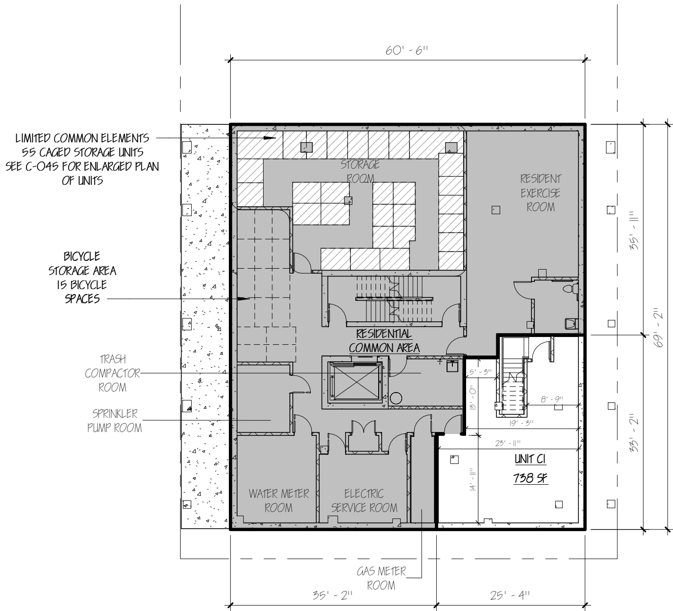
1 00-CELLAR FL 1/16" = 1'-0"
