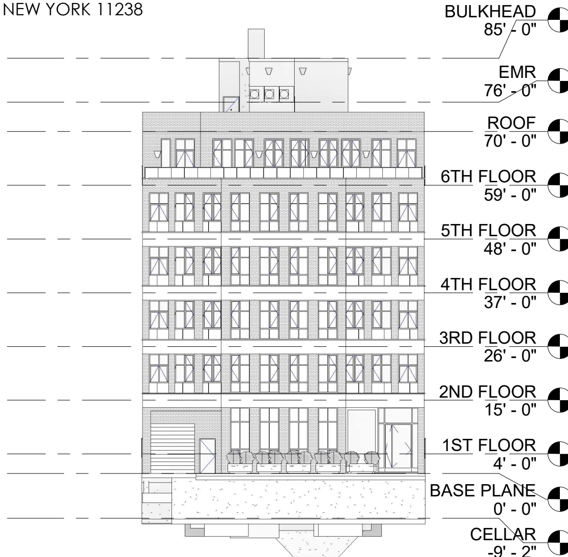
① EAST ELEVATION 1" = 20'-0"
