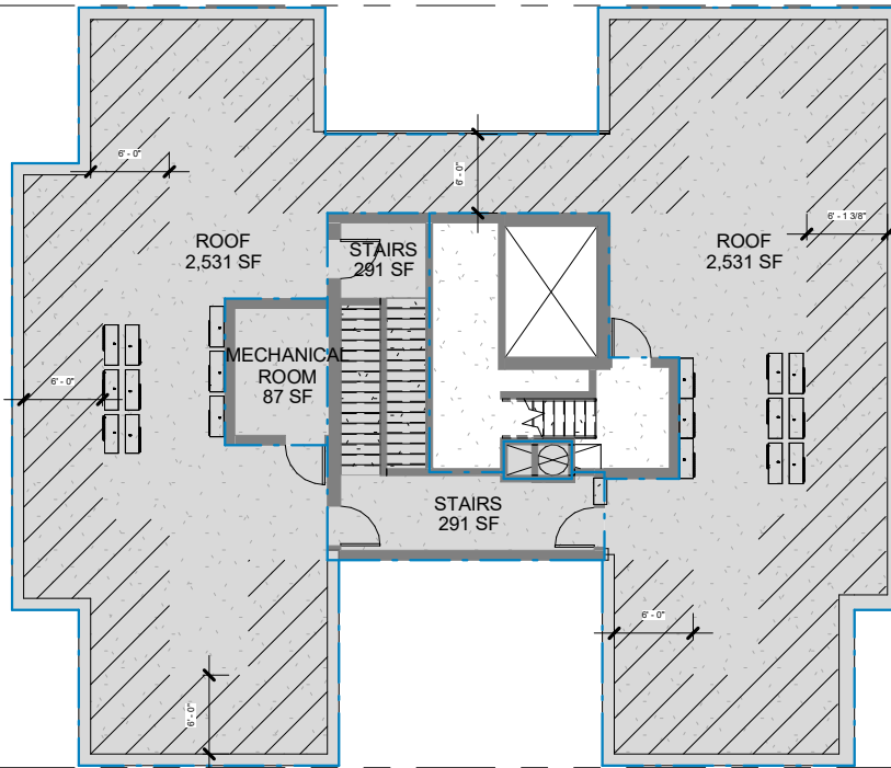
1 ROOF PLAN 1/16" = 1'-0"
