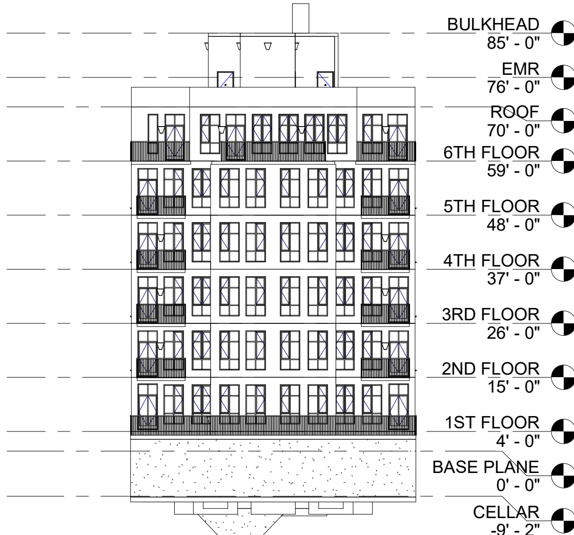
1 WEST ELEVATION 1" = 20'-0"
