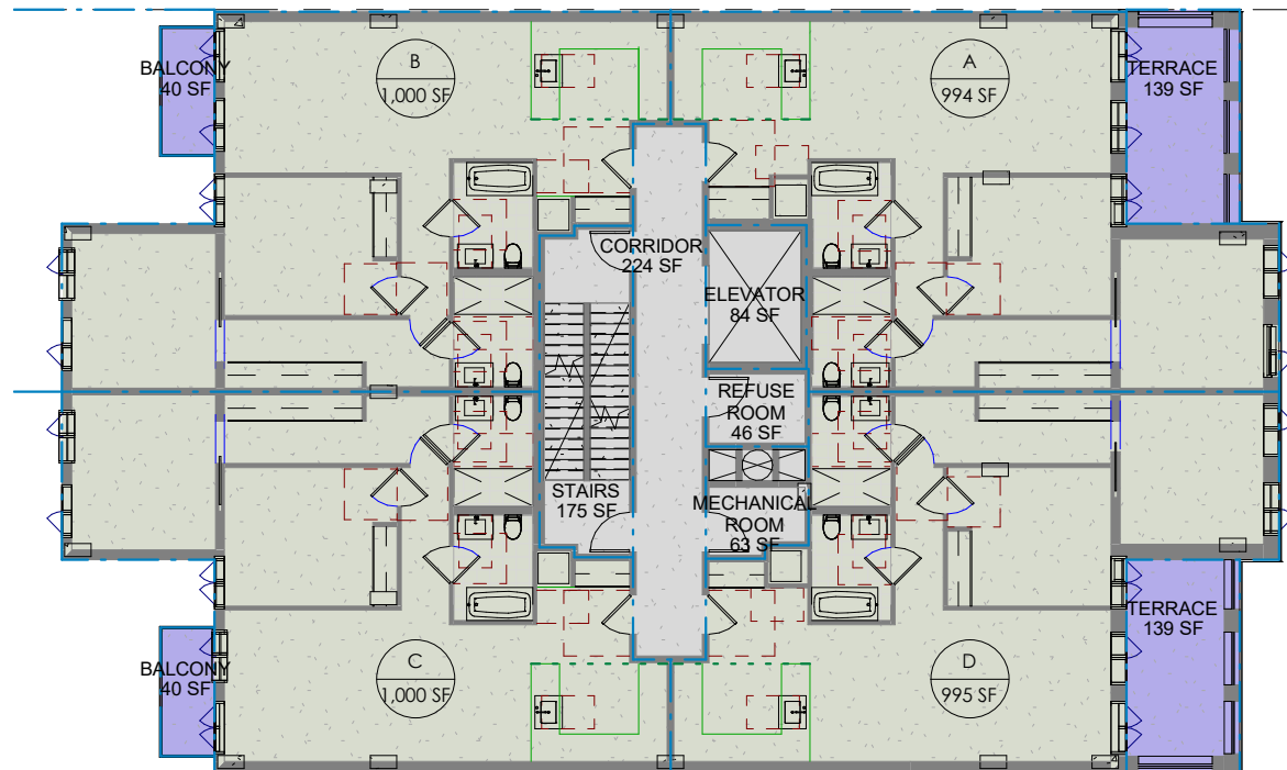
1 4TH - 5TH FLOOR PLAN 1/16" = 1'-0"
