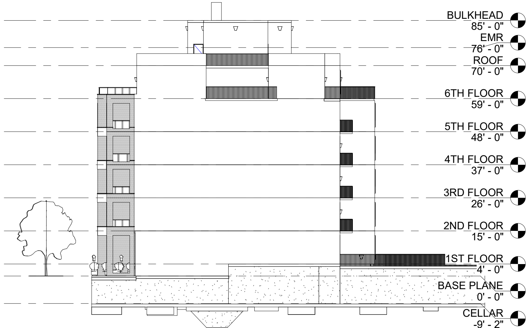
1 NORTH ELEVATION 1" = 20'-0"
