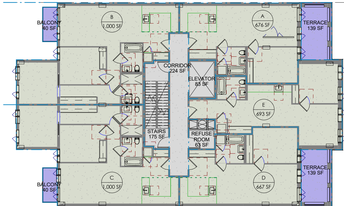
① 2ND - 3RD FLOOR PLAN 1/16" = 1'-0"
