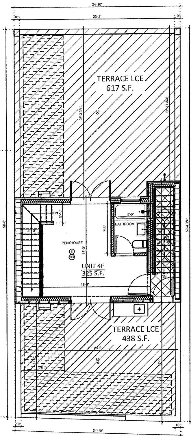
PENTHOUSE/BULKHEAD FLOOR PLAN
