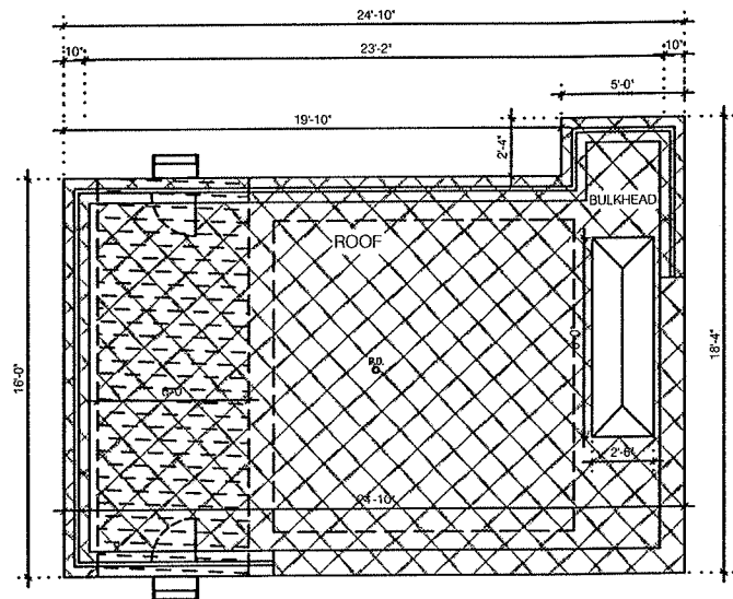
ROOF FLOOR PLAN
