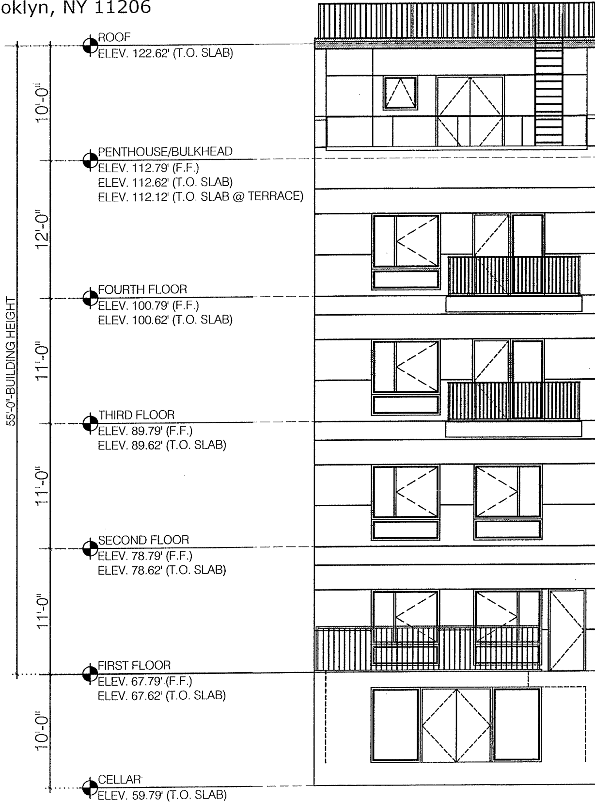
REAR ELEVATIONS
