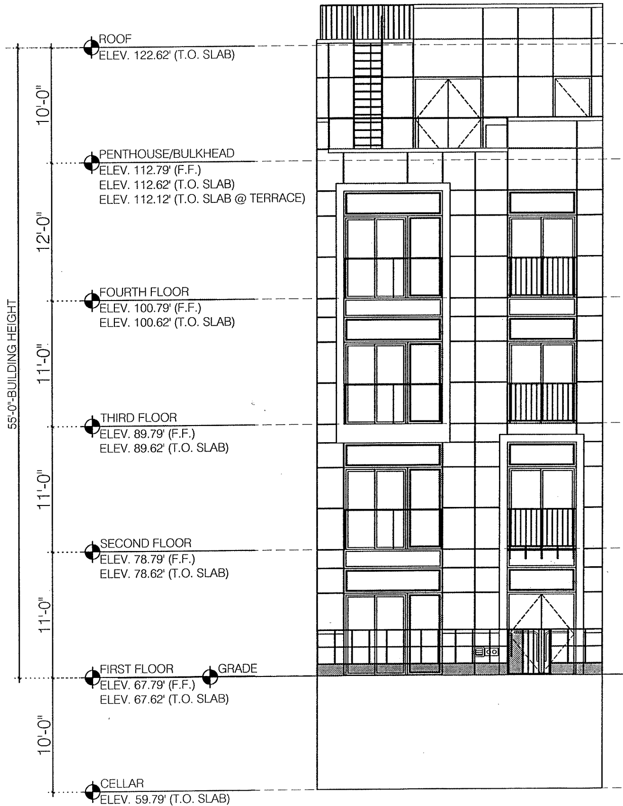
FRONT ELEVATIONS
