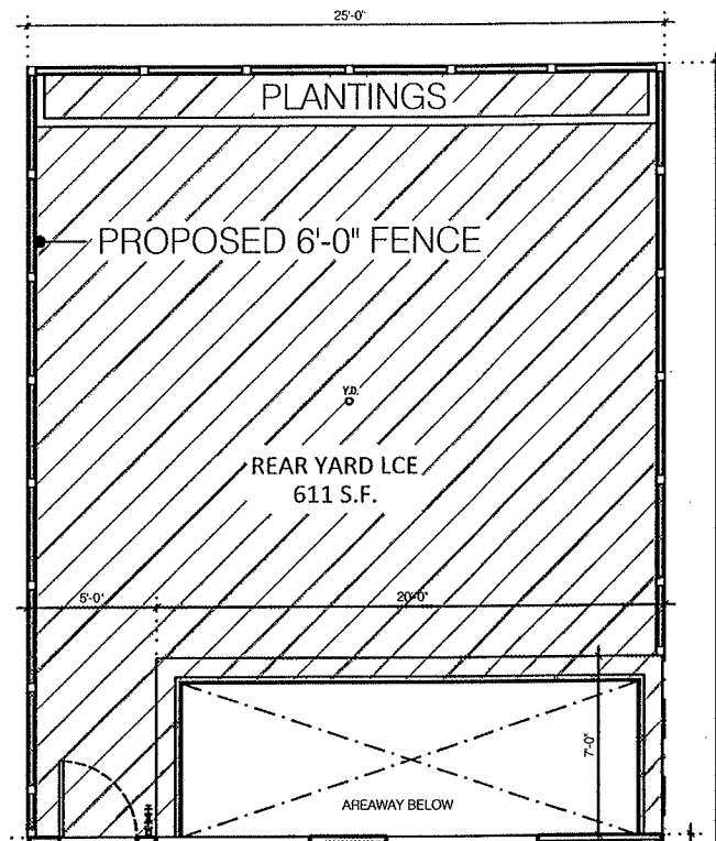
FIRST FLOOR PLAN REAR YARD CONTINUED
