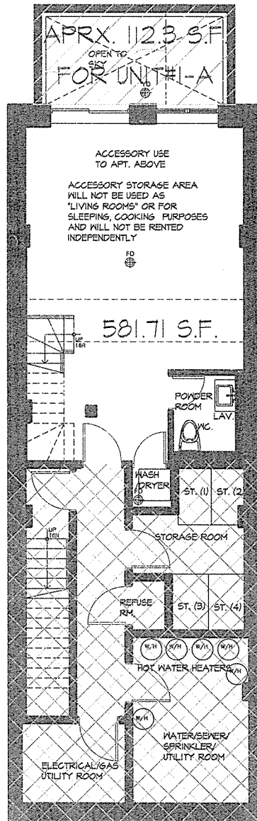
CELLAR FLOOR
