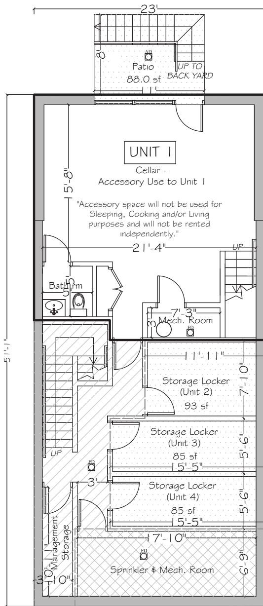
CELLAR FLOOR PLAN
