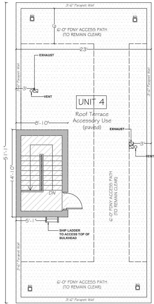
ROOF PLAN
