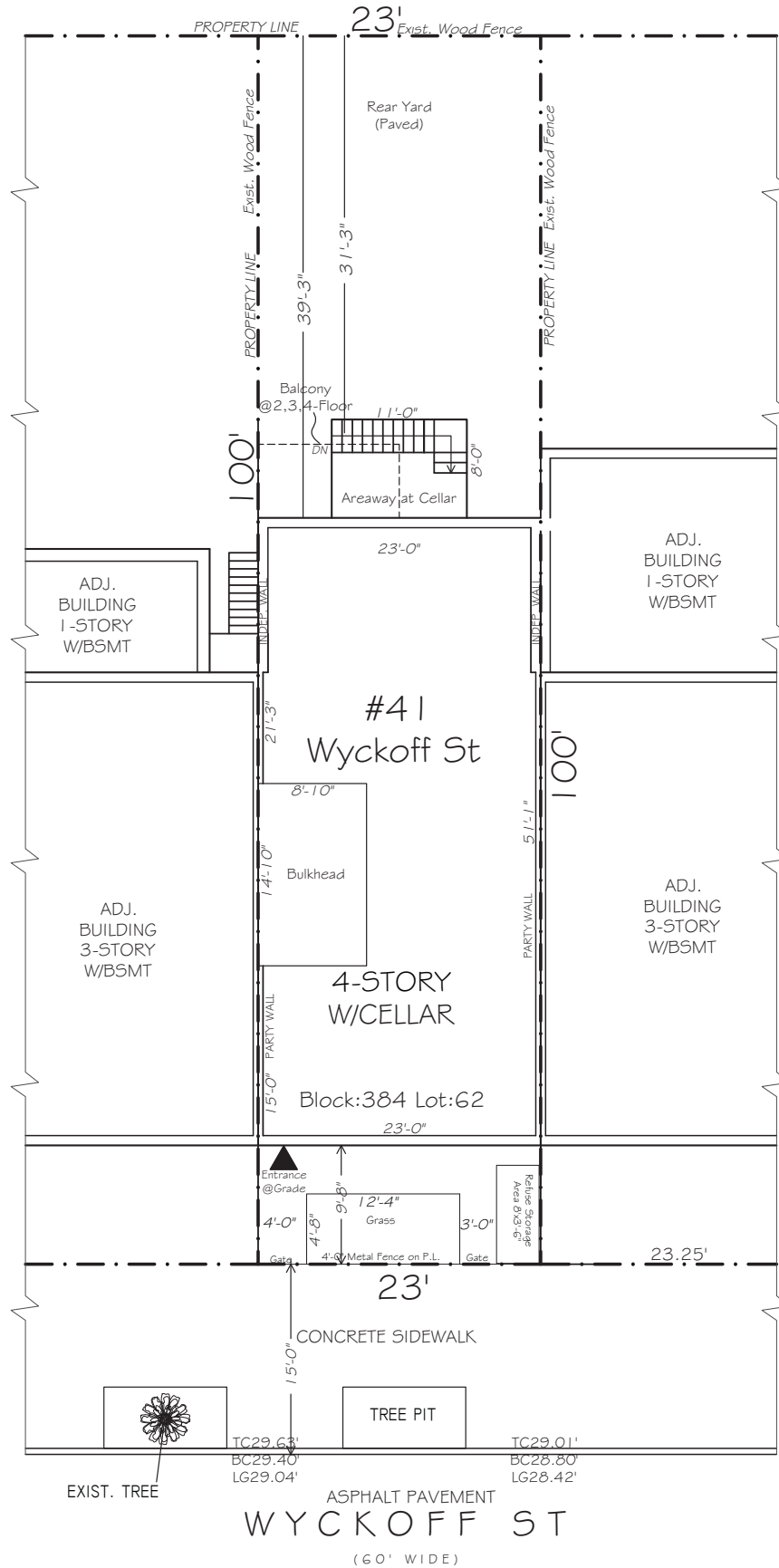
PLOT PLAN
