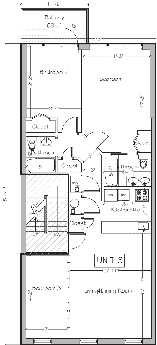
3-FLOOR PLAN
