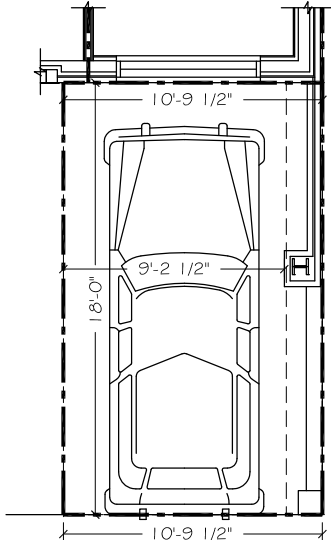
PARKING UNIT 139 P: 194 SQFT
