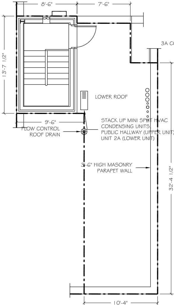
ROOF-COMMON BULKHEAD: 115.8 SQFT ROOF: 382 SQFT
