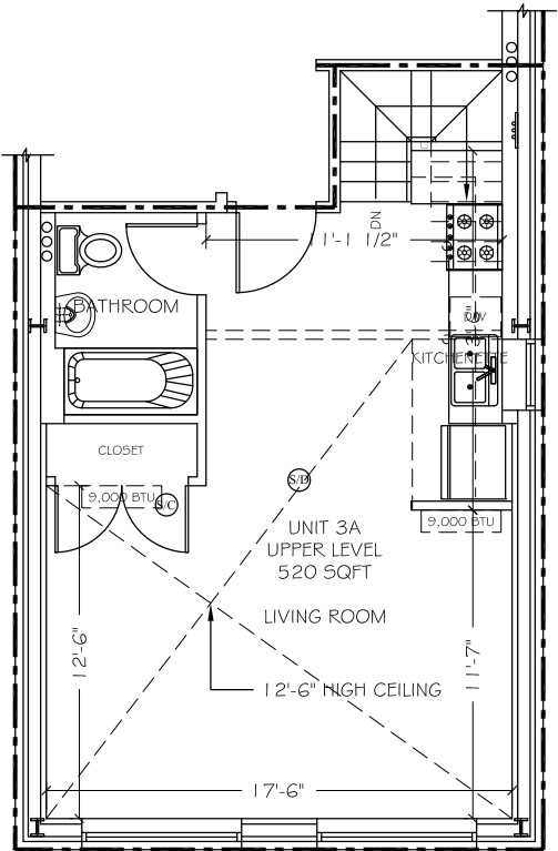
FOURTH FLOOR-UNIT 3A (UPPER LEVEL) AREA: 520 SQFT
