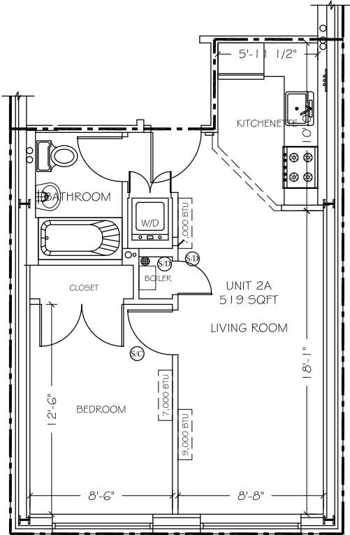
SECOND FLOOR UNIT-2A AREA: 519 SQFT
