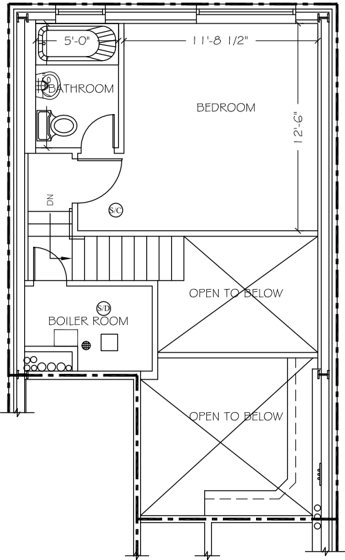
FOURTH FLOOR MEZZANINE-UNIT 4A AREA: 357 SQFT
