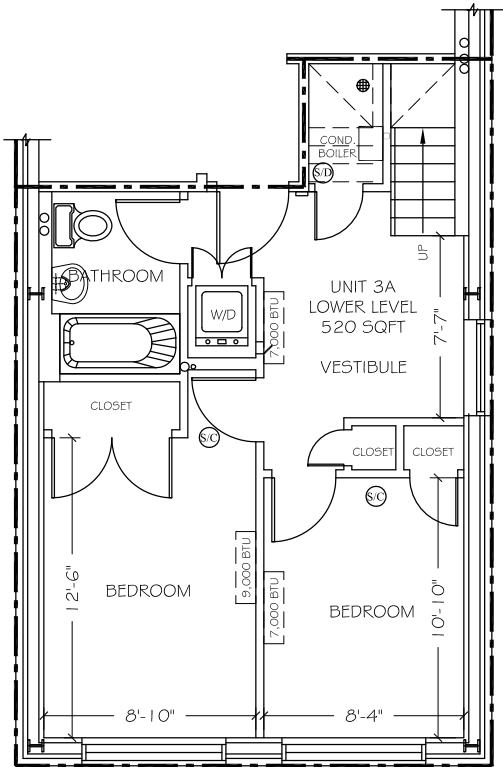
THIRD FLOOR-UNIT 3A (LOWER LEVEL) AREA: 520 SQFT
