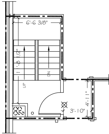
THIRD TO FOURTH FLOOR-COMMON AREA: 131 SQFT
