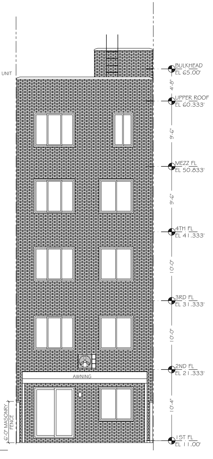
REAR ELEVATION
