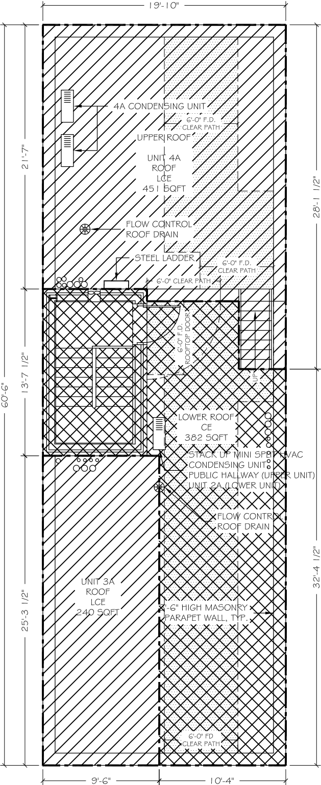
ROOF KEY PLAN
