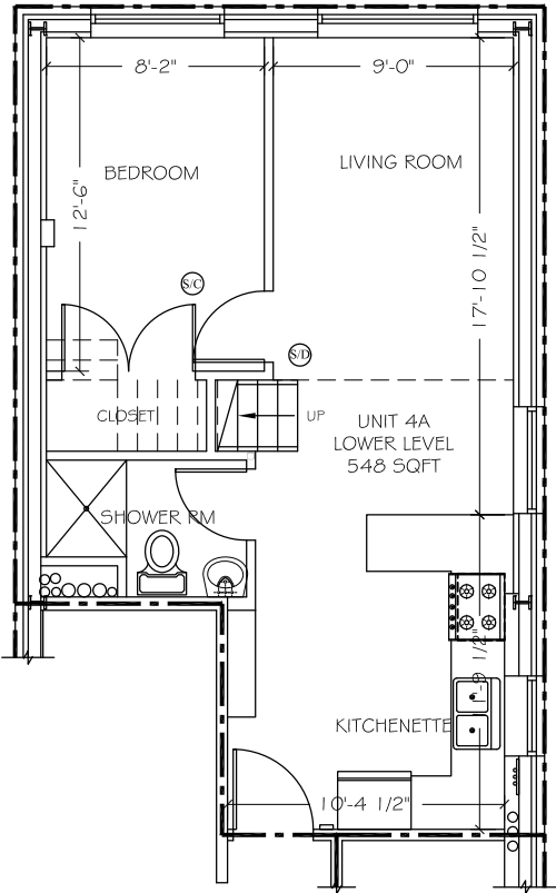
FOURTH FLOOR-UNIT 4A AREA: 548 SQFT
