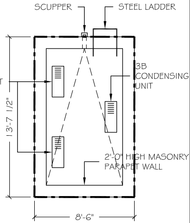
STAIR BULKHEAD ROOF-COMMON AREA: 116 SQFT
