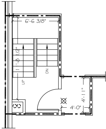
SECOND-COMMON AREA: 132 SQFT
