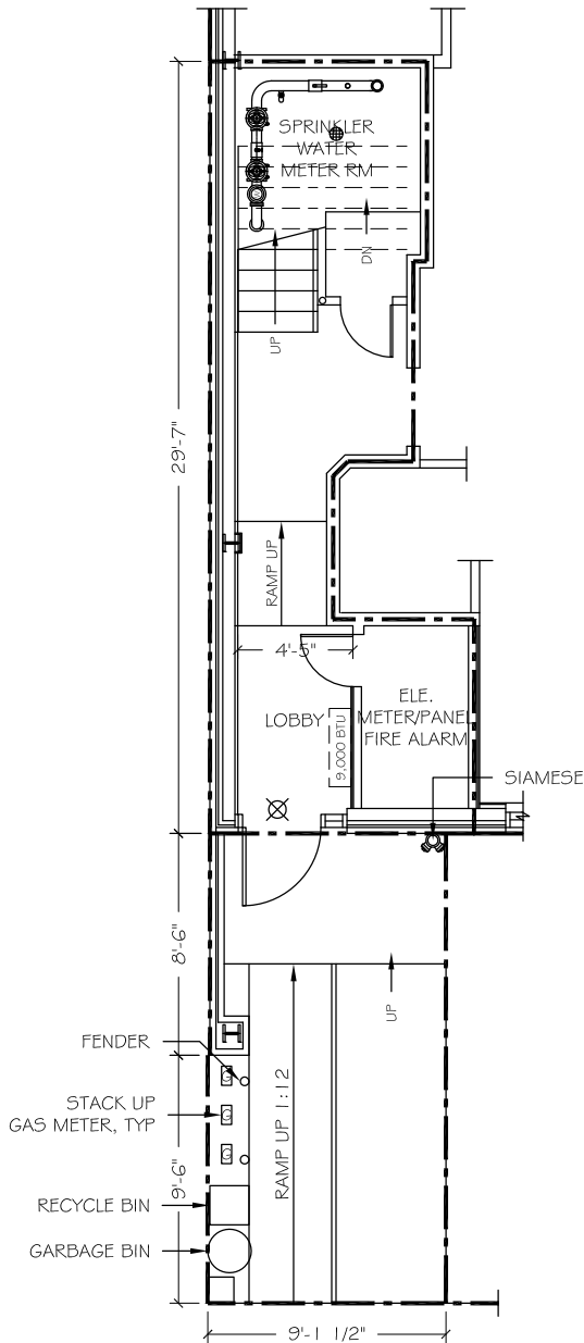
FIRST FLOOR-COMMON AREA: 235 SQFT FRONT YARD: 164 SQFT
