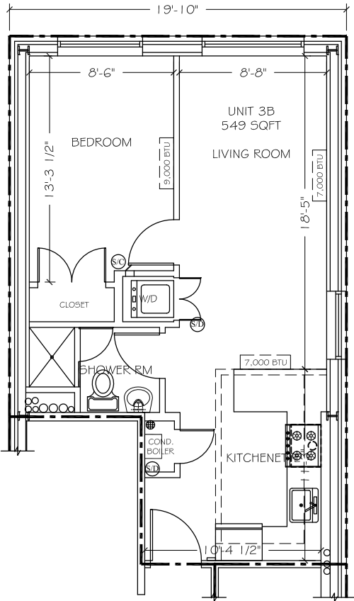
THIRD FLOOR-UNIT 3B AREA: 549 SQFT
