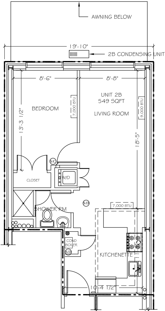
SECOND FLOOR-UNIT 2B AREA: 549 SQFT
