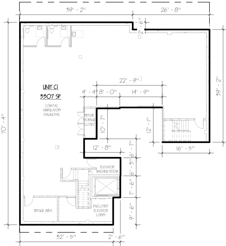
1 00-UNIT C1 CELLAR 1/16" = 1'-0"
