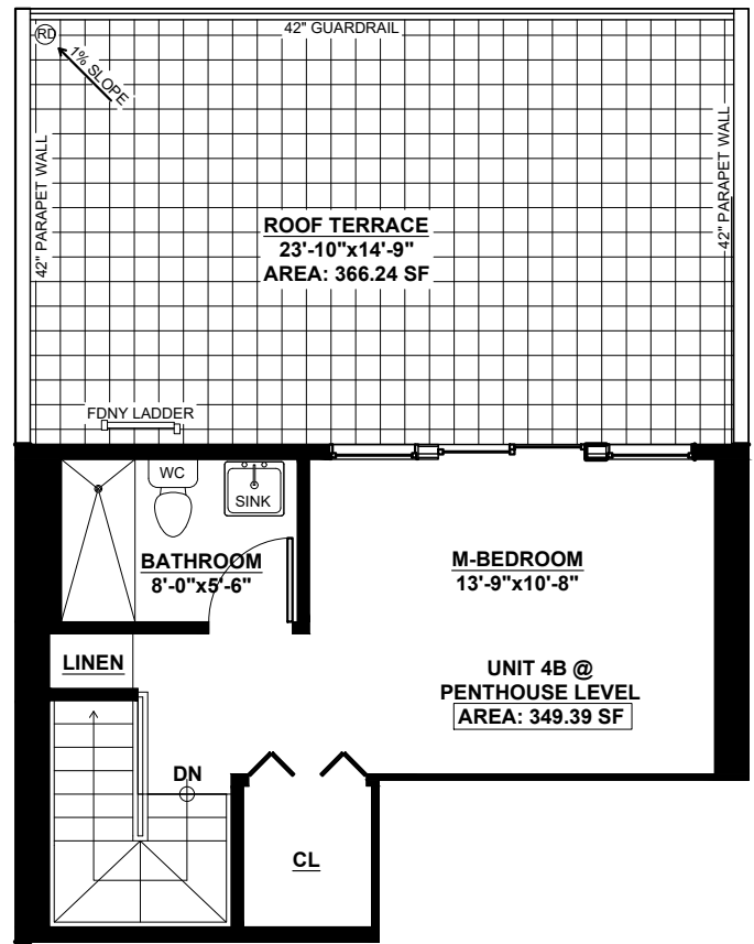
PENTHOUSE LEVEL
