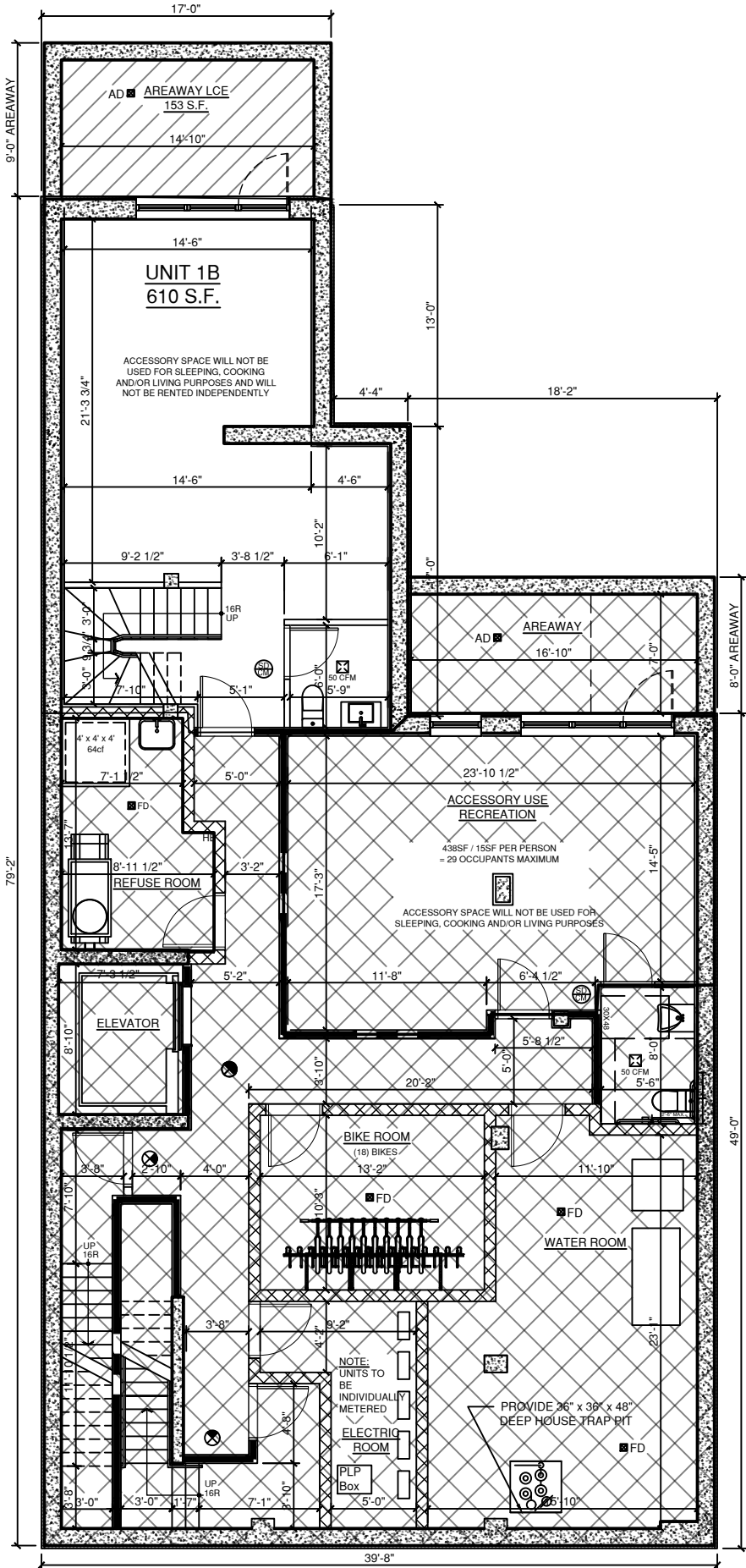
CELLAR FLOOR PLAN
