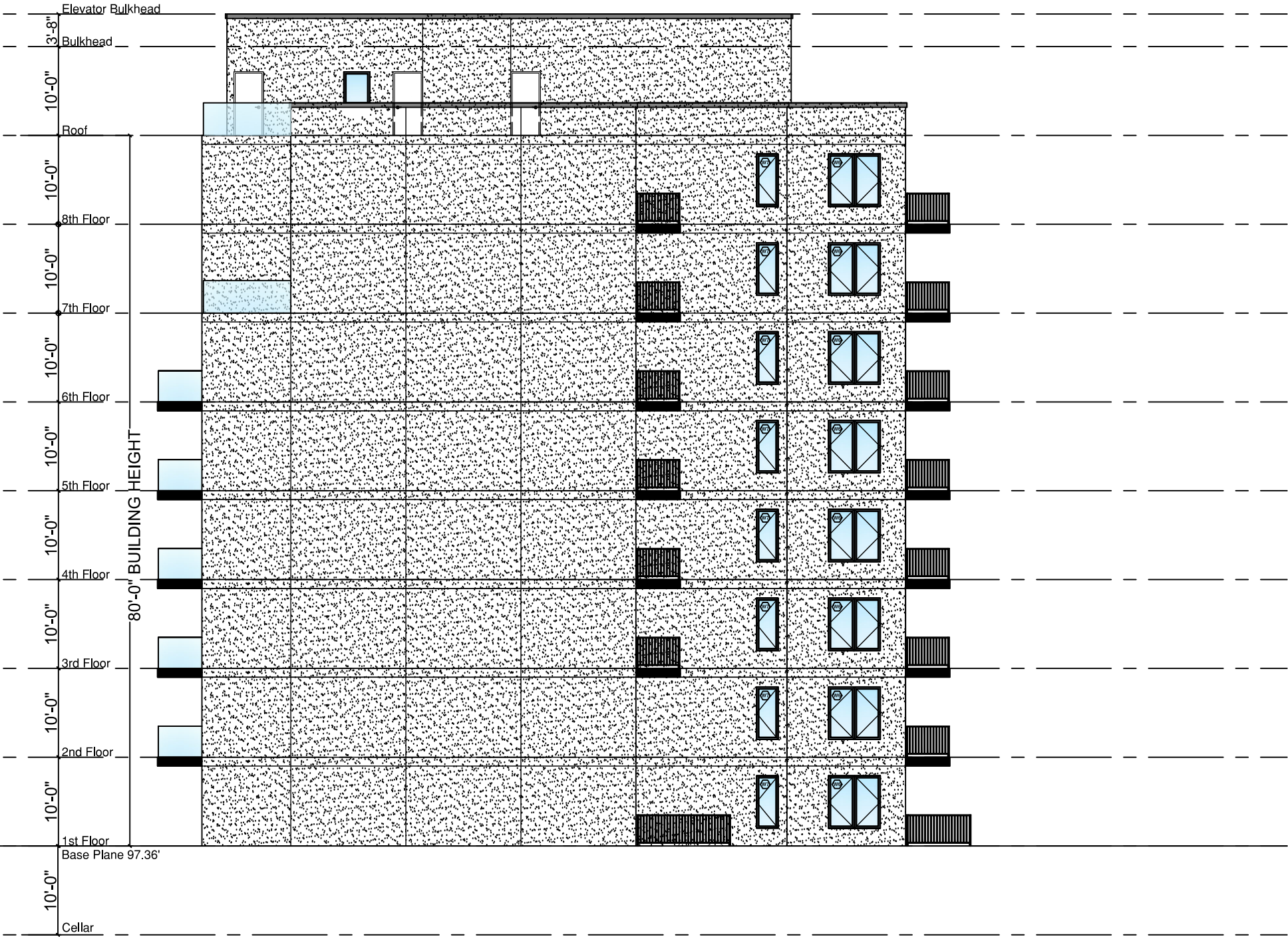
WEST ELEVATIONS
