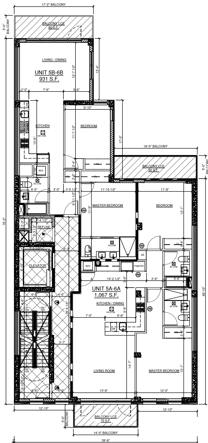
FIFTH AND SIXTH FLOOR PLAN
