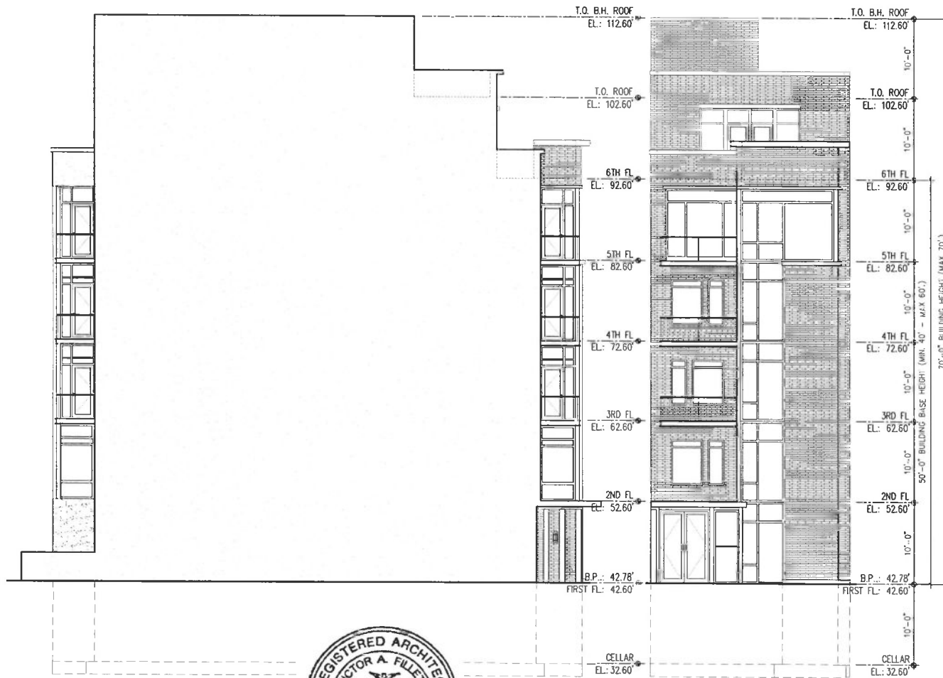
SIDE ELEVATION 1
